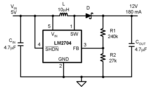
Figure 7. 5V to 12V Application
