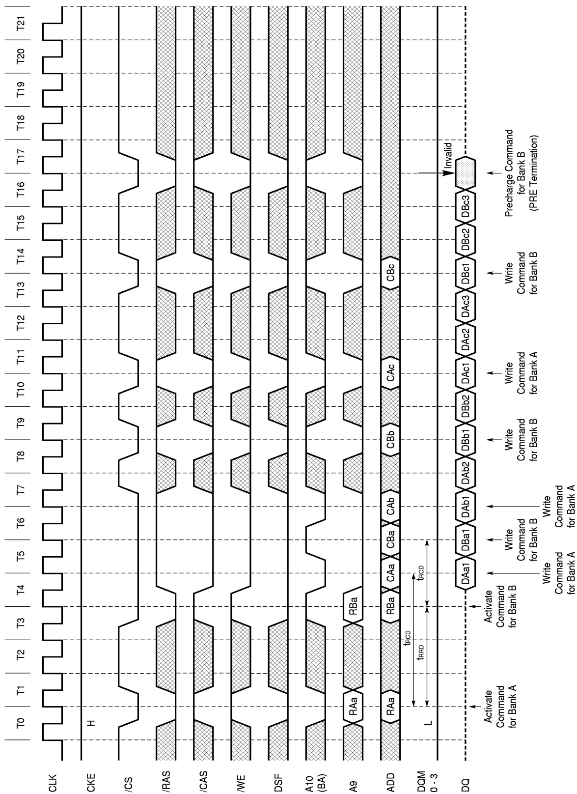
Full Page Random Column Write (Burst length = Full Page, /CAS latency = 2)
