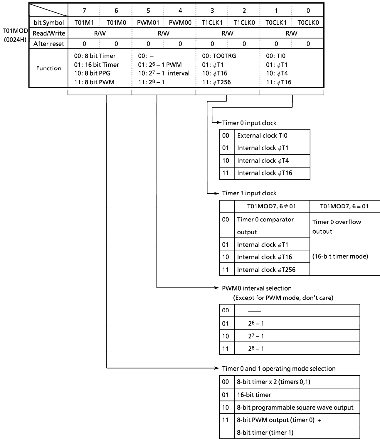
Figure 3.8 (4) Timer 0/1 Mode Register (T01MOD)
