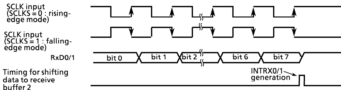
Figure 3.11 (21) Data Receive in I/O Interface Mode (SCLK Input Mode)
