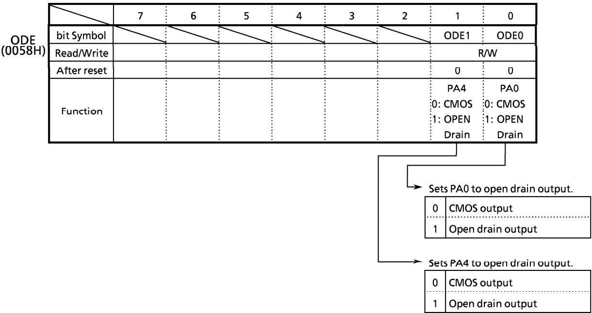
Figure 3.11 (11) Port A Open Drain Enable Register (ODE)
