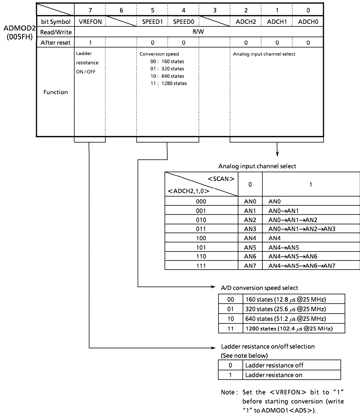
Figure 3.12 (2-2) A/D Control Register
