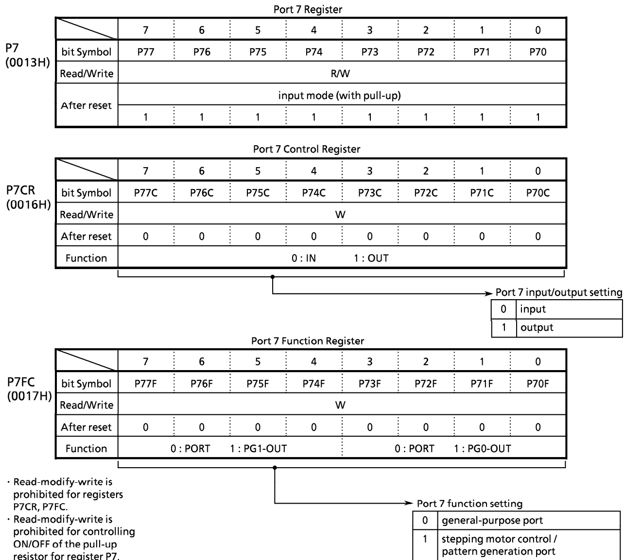
Figure 3.5 (11) Port 7 Registers
