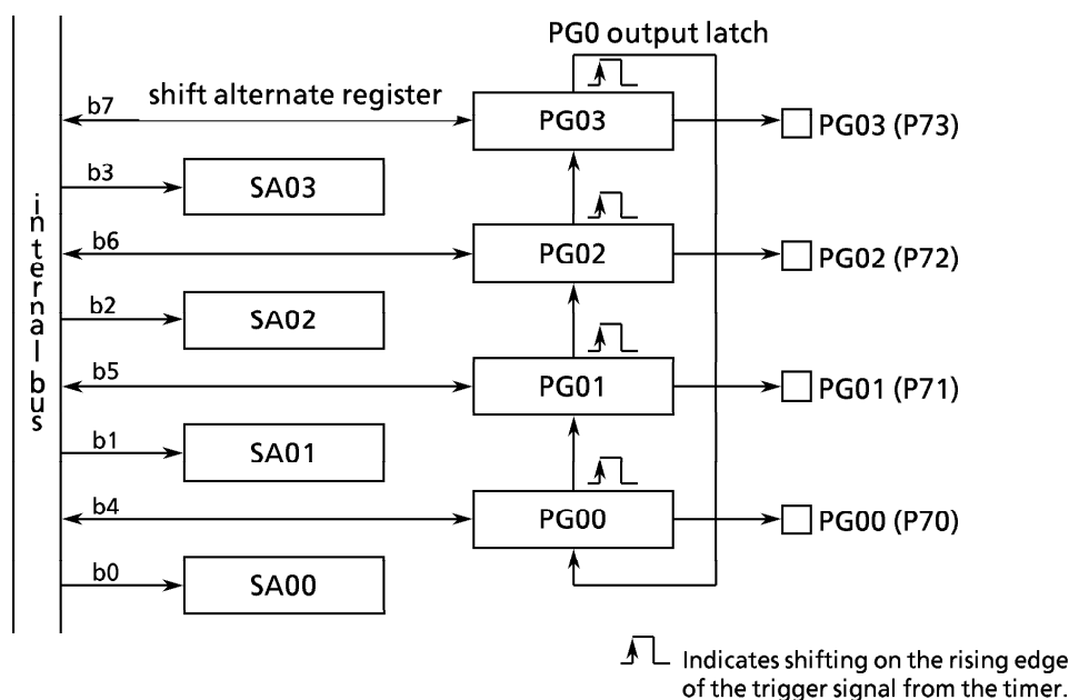
Figure 3.10 (10) Block Diagram of 4-Phase, 1 or 2 Excitation (Normal)
