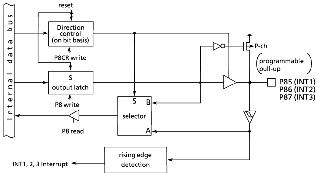
Figure 3.5 (14) Port 8 : P85, P86, and P87
