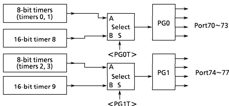
Figure 3.10 (6) Connections Between Timers and Pattern Generator
