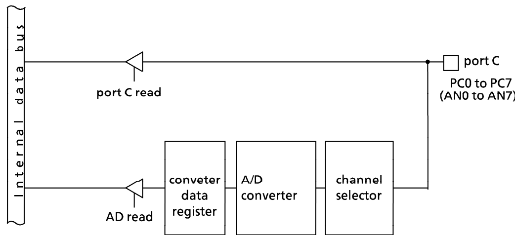
Figure 3.5 (25) Port C
