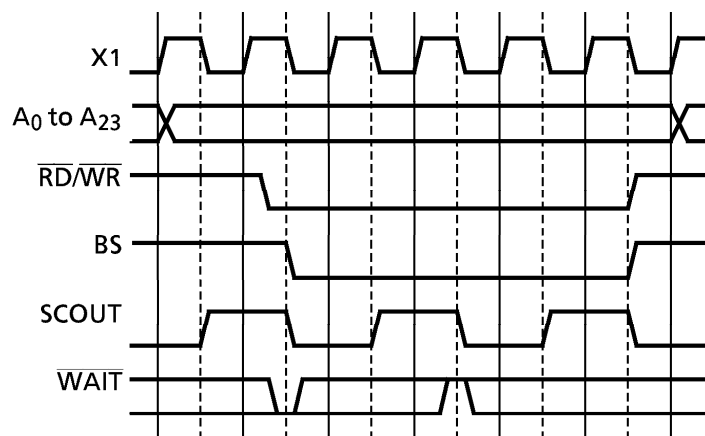
Figure 3.6 (2) 0 + N WAIT Read / Write Cycle (N = 1)
