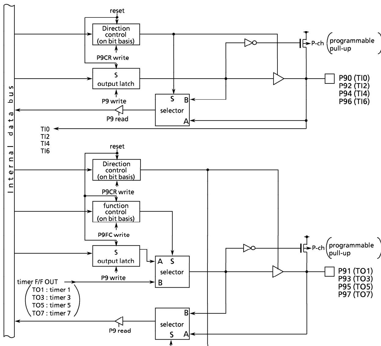
Figure 3.5 (16) Port 9
