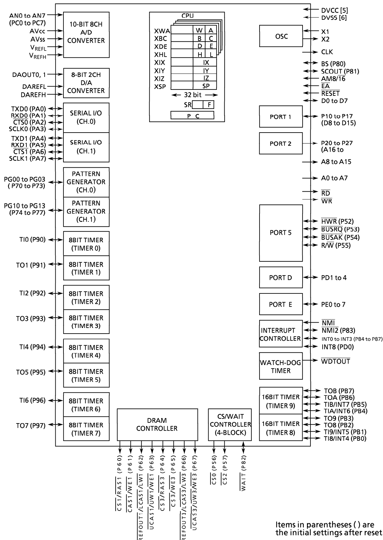
Figure 1 TMP95C063 Block Diagram
