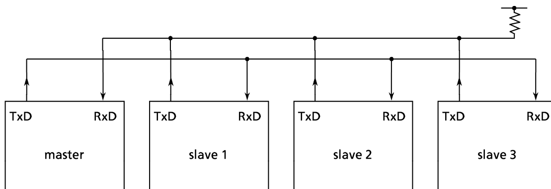
Figure 3.11 (22) Serial Link with Wake-Up Function
