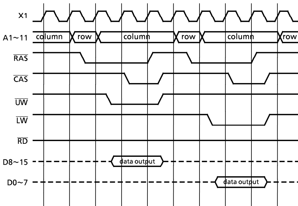
Figure 3.7 (4) c DRAM Access Timing (2WE Mode, Write Cycle, and Byte Access)
