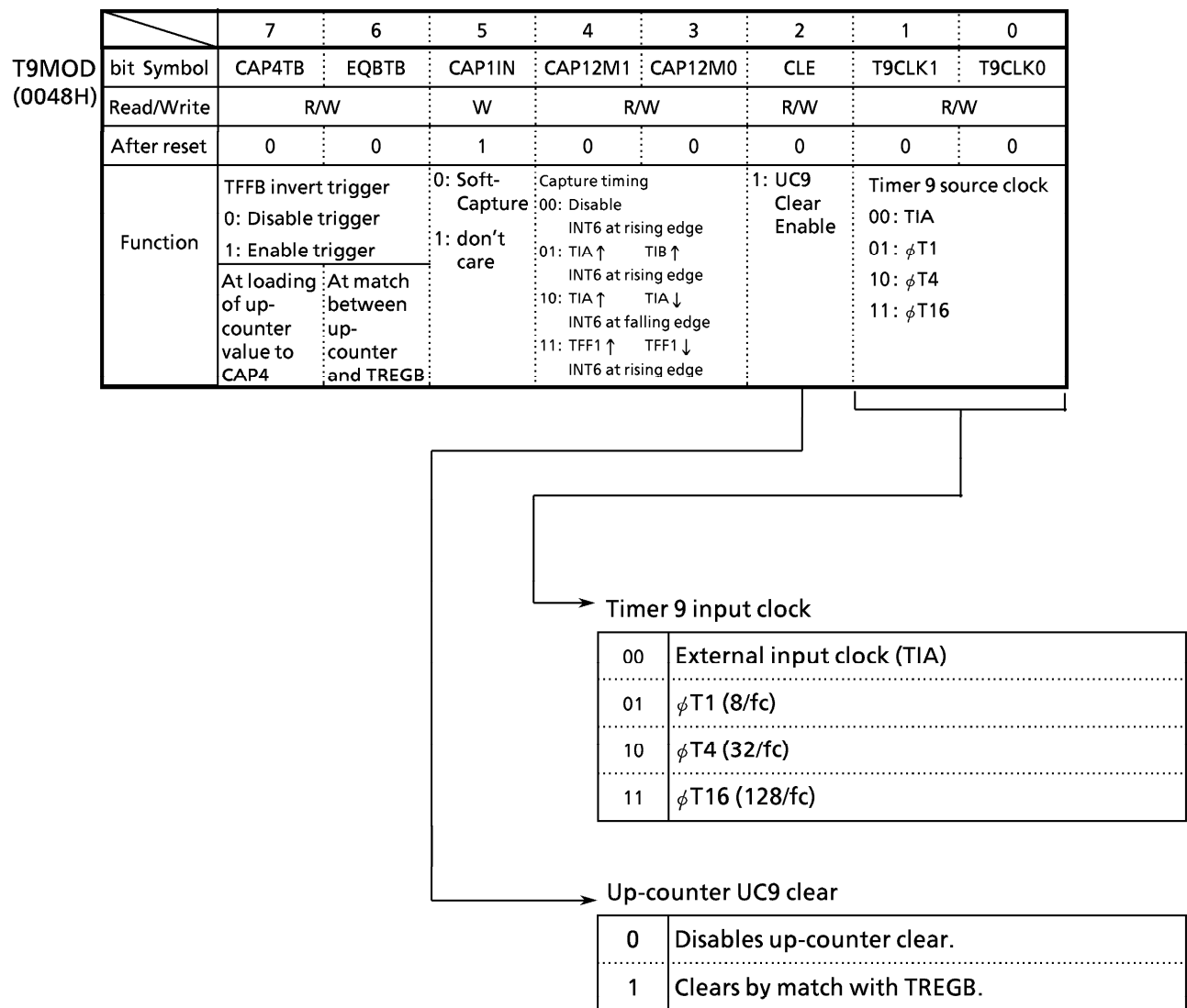
Figure 3.9 (5) 16-Bit Timer Mode Control Register (T9MOD) (1/2)
