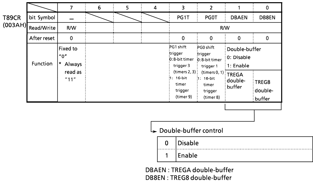
Figure 3.9 (8) 16-Bit Timer (8/9) Control Register (T89CR)
