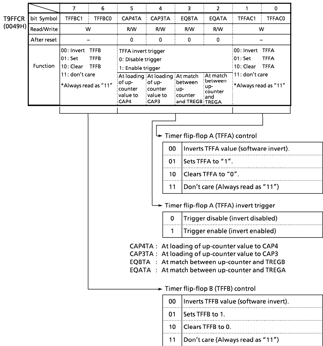
Figure 3.9 (7) 16-Bit Timer 9 F/F Control (T9FFCR)
