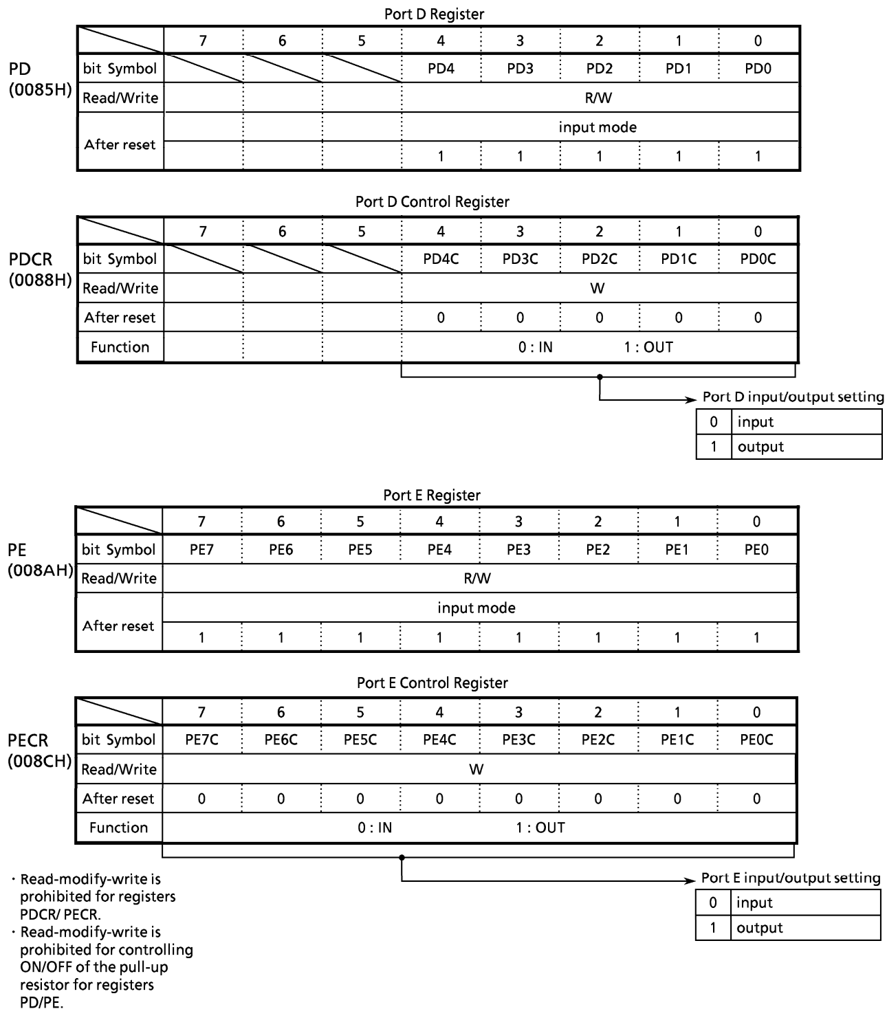
Figure 3.5 (29) Port D, E Registers
