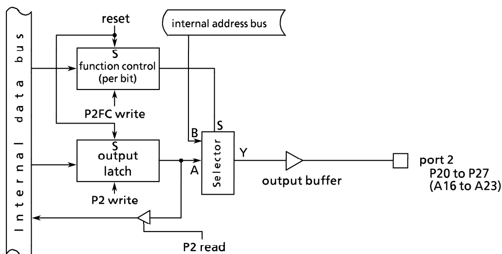
Figure 3.5 (3) Port 2
