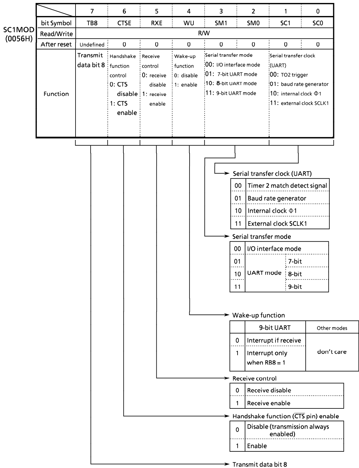
Figure 3.11 (6) Serial Mode Control Register (SC1MOD, Channel 1)
