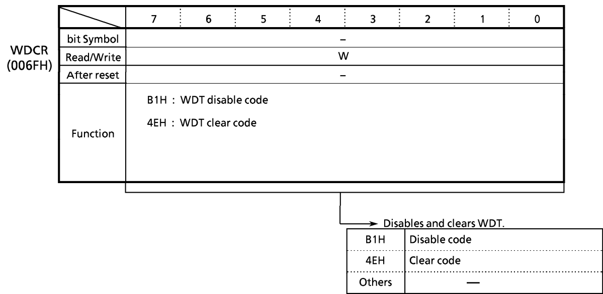
Figure 3.14 (5) Watchdog Timer Control Register
