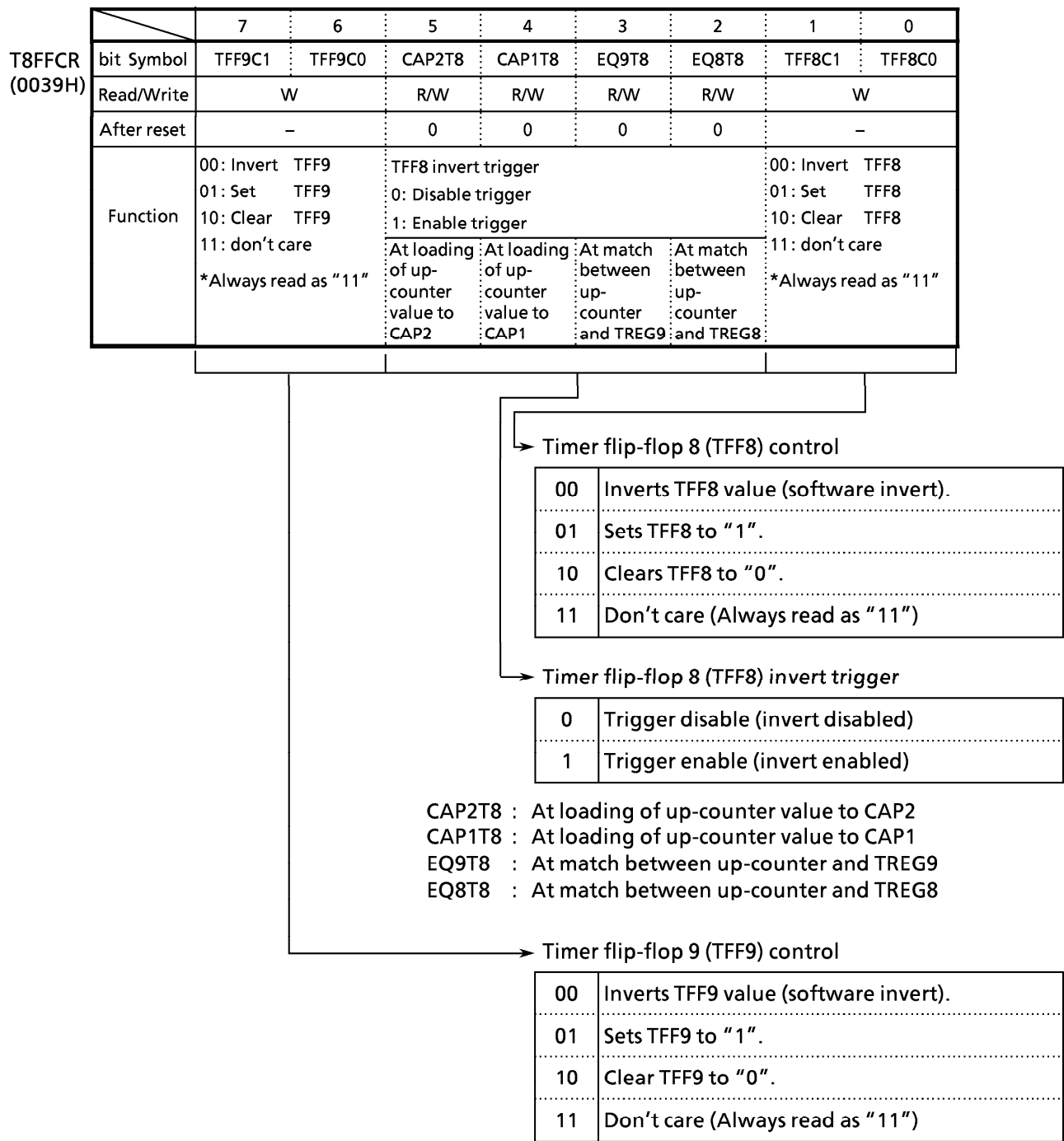
Figure 3.9 (4) 16-Bit Timer 8 F/F Control (T8FFCR)
