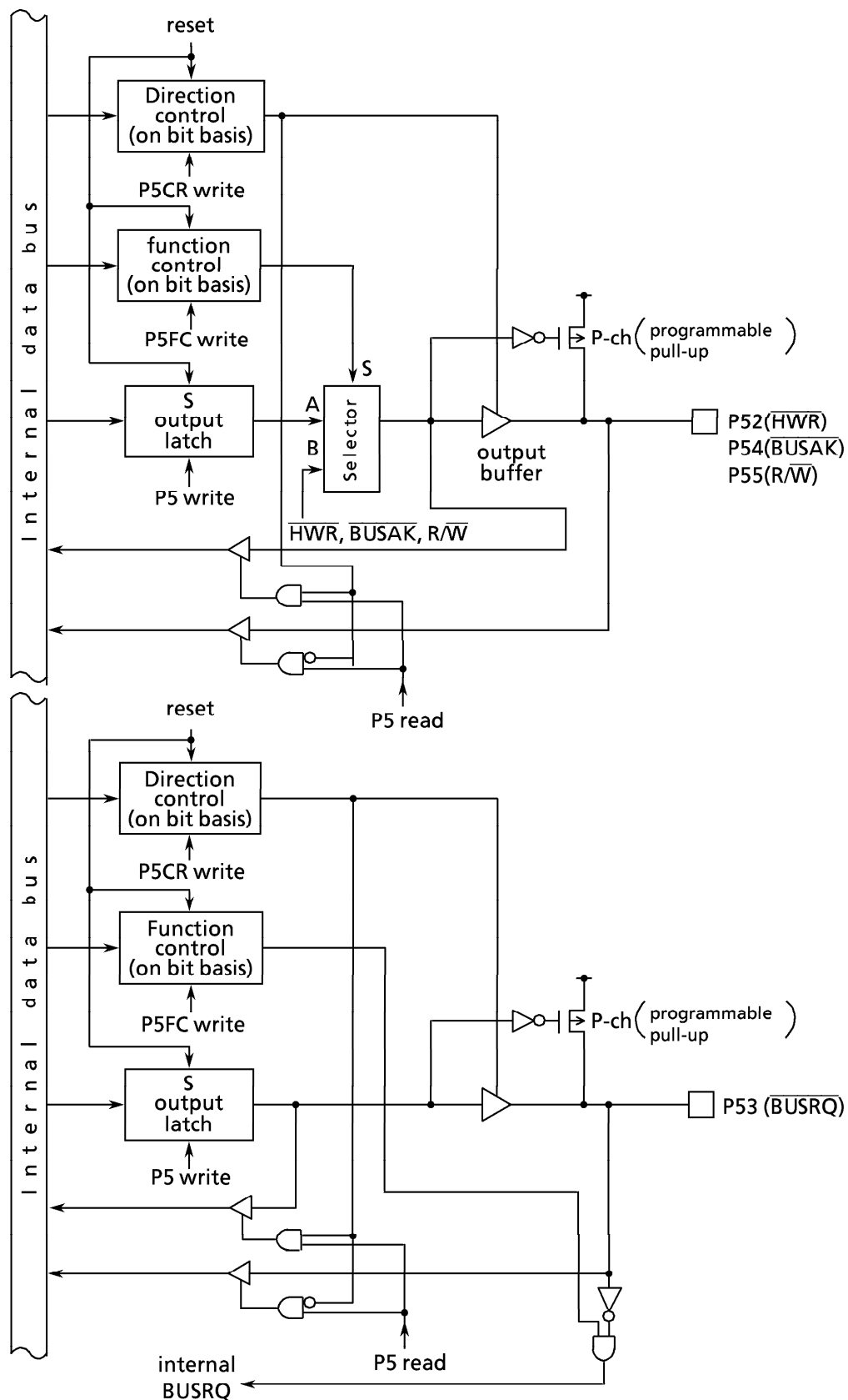
Figure 3.5 (5) Port 5 : P52 to P55
