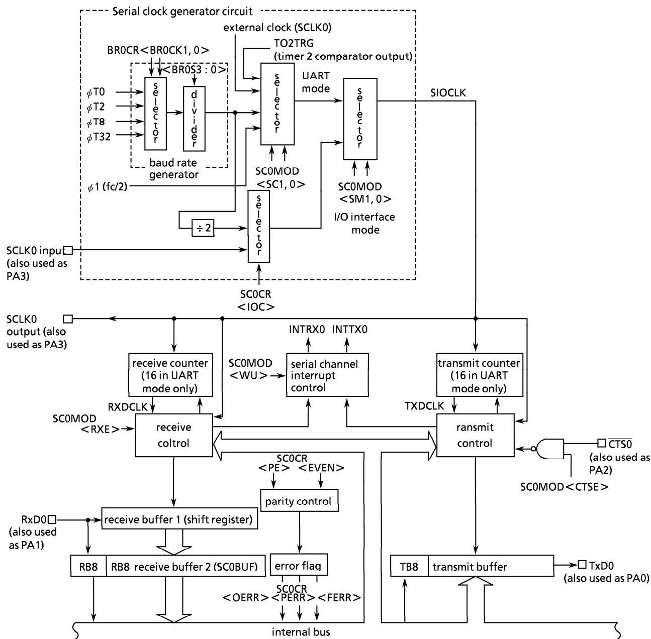
Figure 3.11 (12) Serial Channel 0 Block Diagram
