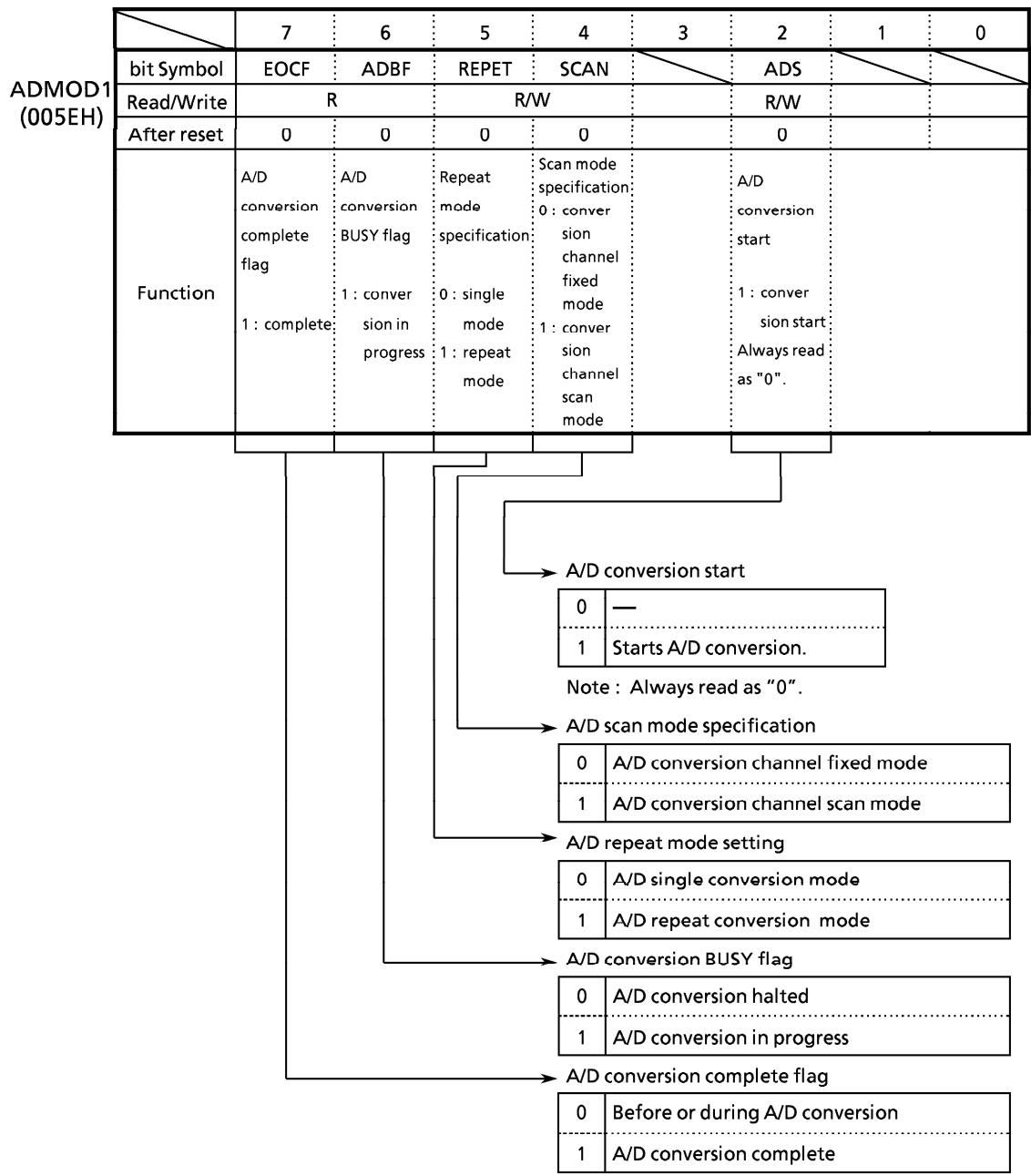
Figure 3.12 (2-1) A/D Control Register
