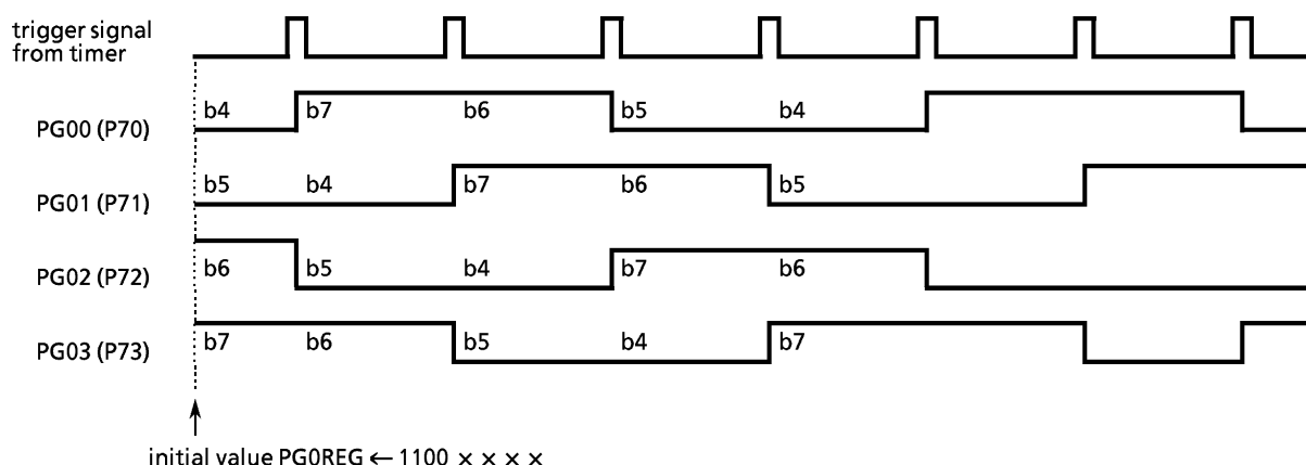
Figure 3.10 (9) 4-Phase, 2 Excitation Output Waveform (Normal)
