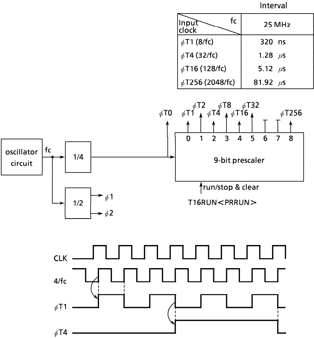
Figure 3.8 (2) Prescaler
