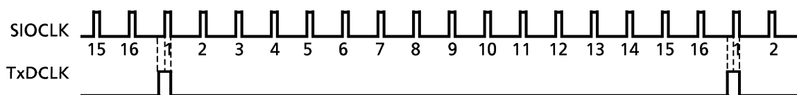
Figure 3.11 (13) Transmission Clock Generation
