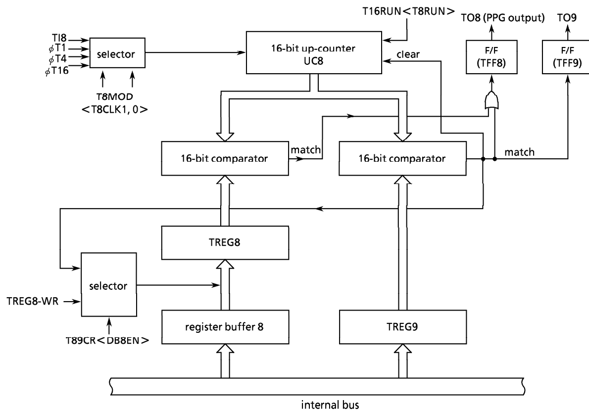
Figure 3.9 (12) 16-Bit PPG Mode Block Diagram
