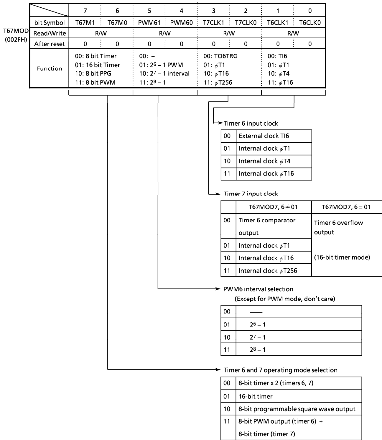
Figure 3.8 (7) Timer 6/7 Mode Register (T67MOD)
