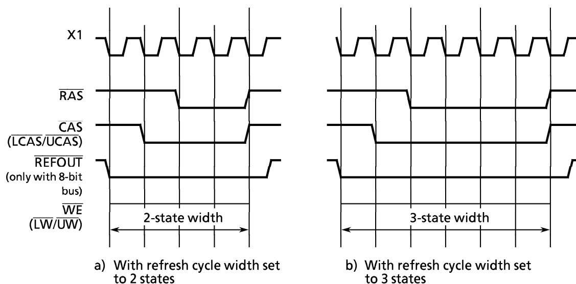
Figure 3.7 (5) Refresh Cycle Timing Examples
