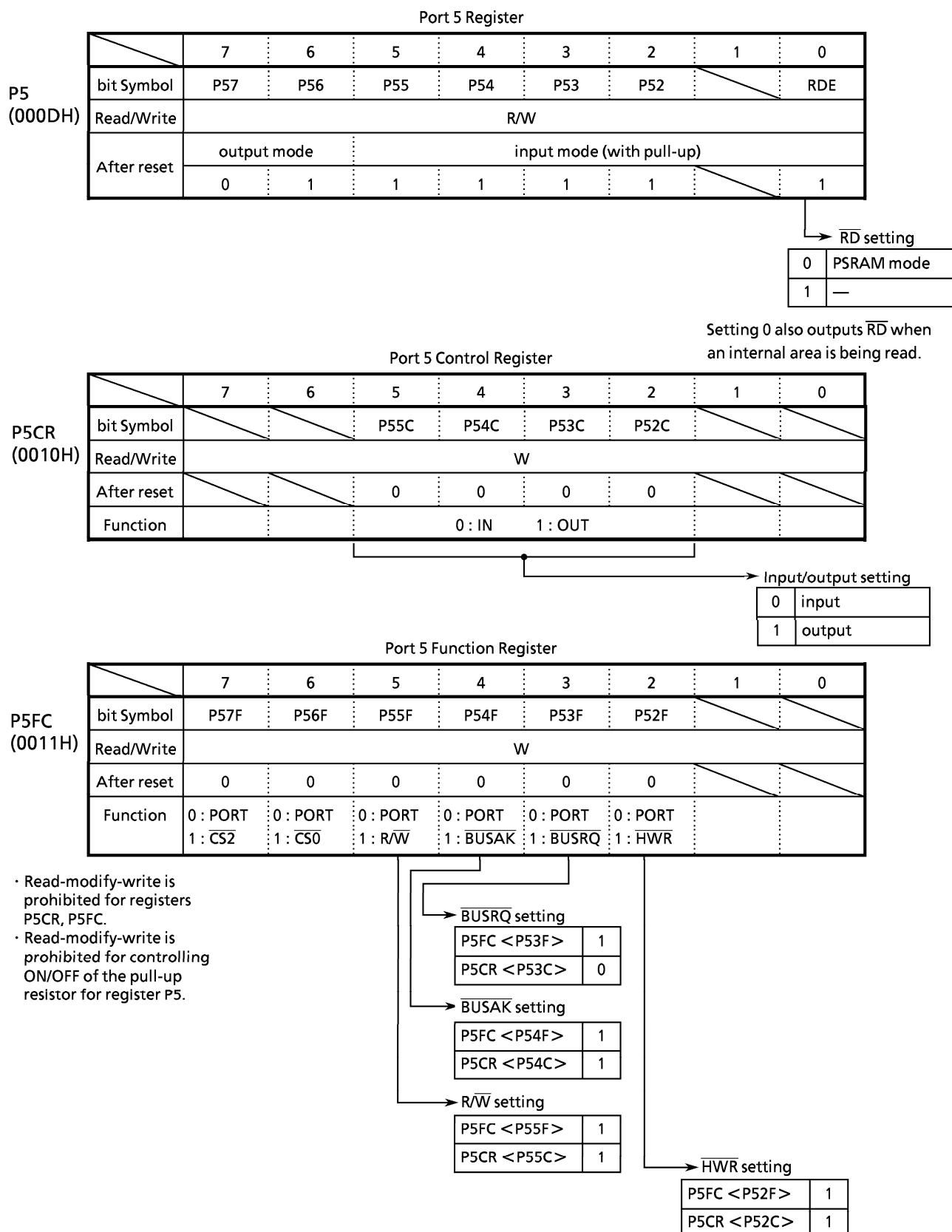
Figure 3.5 (7) Port 5 Registers
