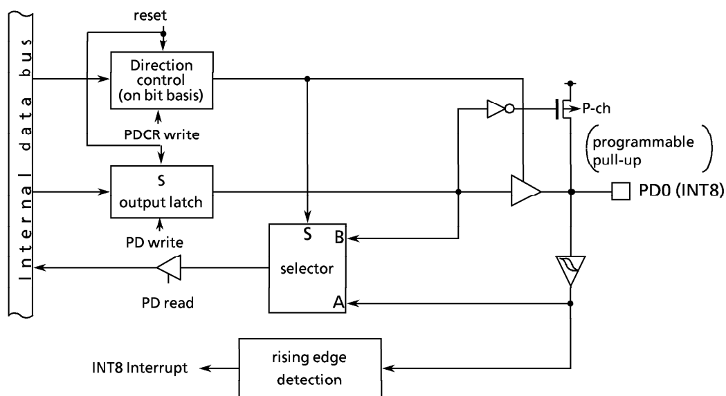
Figure 3.5 (27) Port D : PD0
