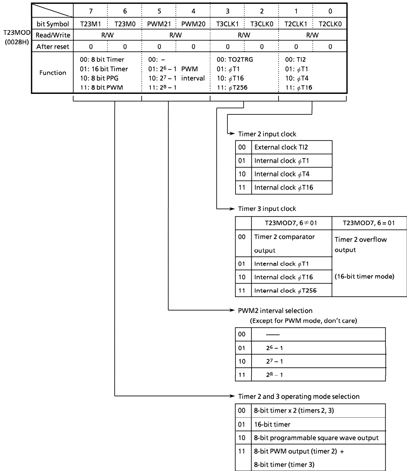
Figure 3.8 (5) Timer 0/1 Mode Register (T23MOD)
