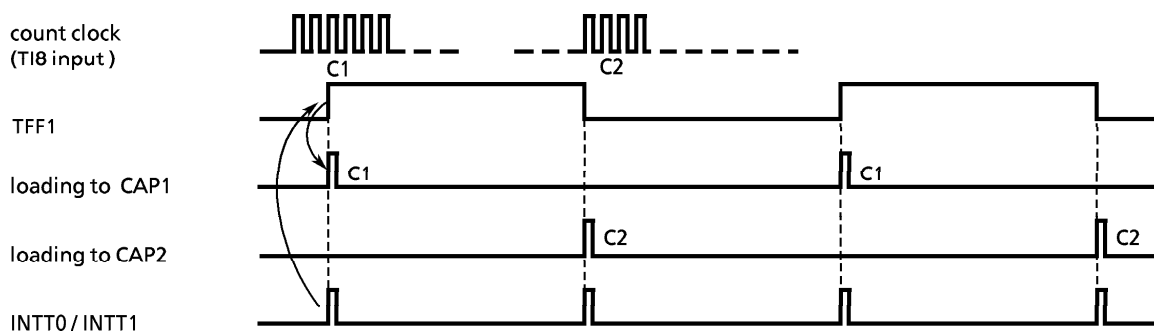
Figure 3.9 (15) Frequency Measurement
