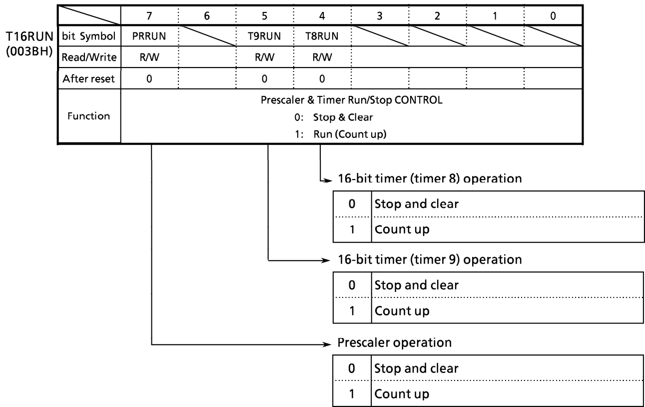
Figure 3.9 (9) 16-Bit Timer Operation Control Register (T16RUN)
