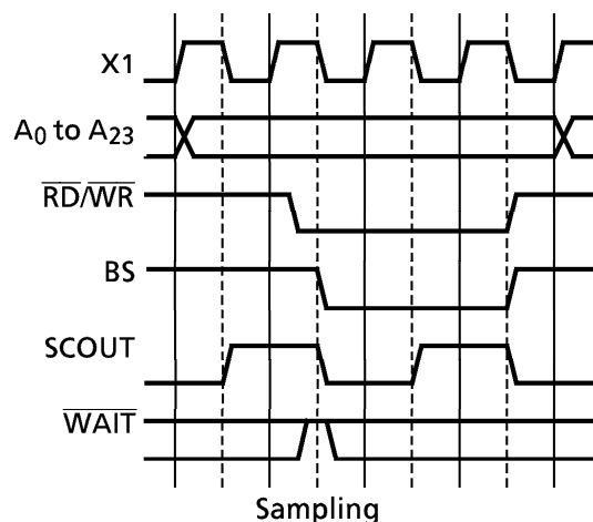
Figure 3.6 (1) 0 + N WAIT Read / Write Cycle (N = 0)
