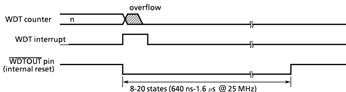
Figure 3.14 (3) Reset Mode
