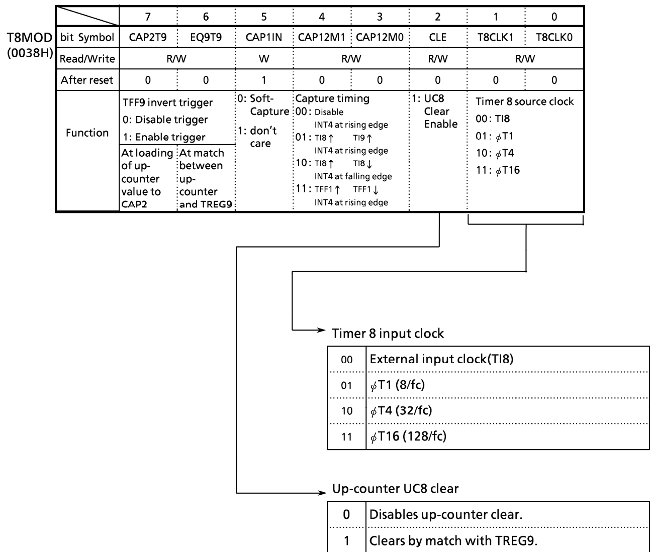
Figure 3.9 (2) 16-Bit Timer Mode Control Register (T8MOD) (1/2)
