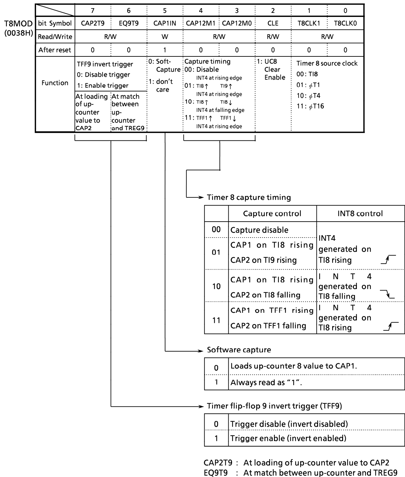
Figure 3.9 (3) 16-Bit Timer Control Register (T8MOD) (2/2)
