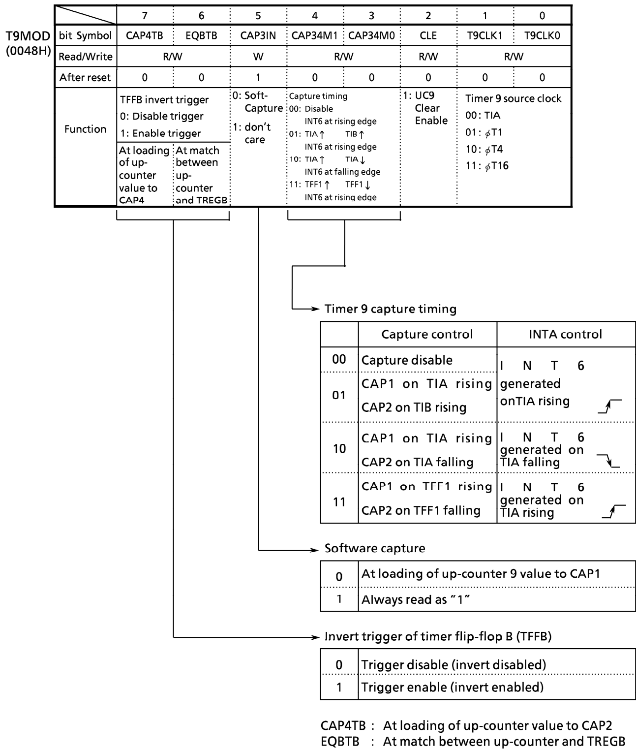
Figure 3.9 (6) 16-Bit Timer Control Register (T9MOD) (2/2)
