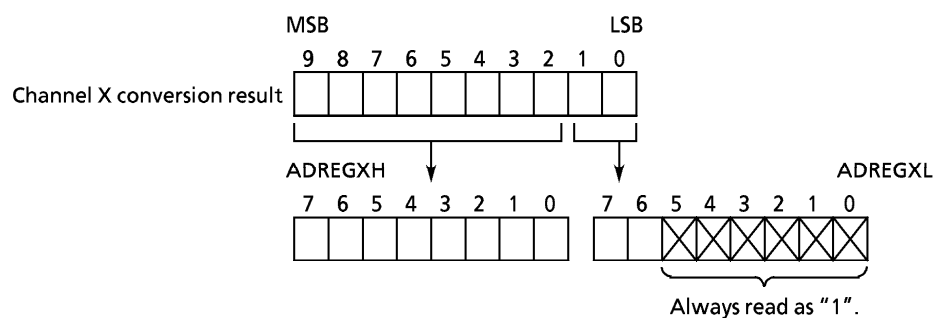
Figure 3.12 (3-1) A/D Conversion Result Registers (ADREG04, 15)
