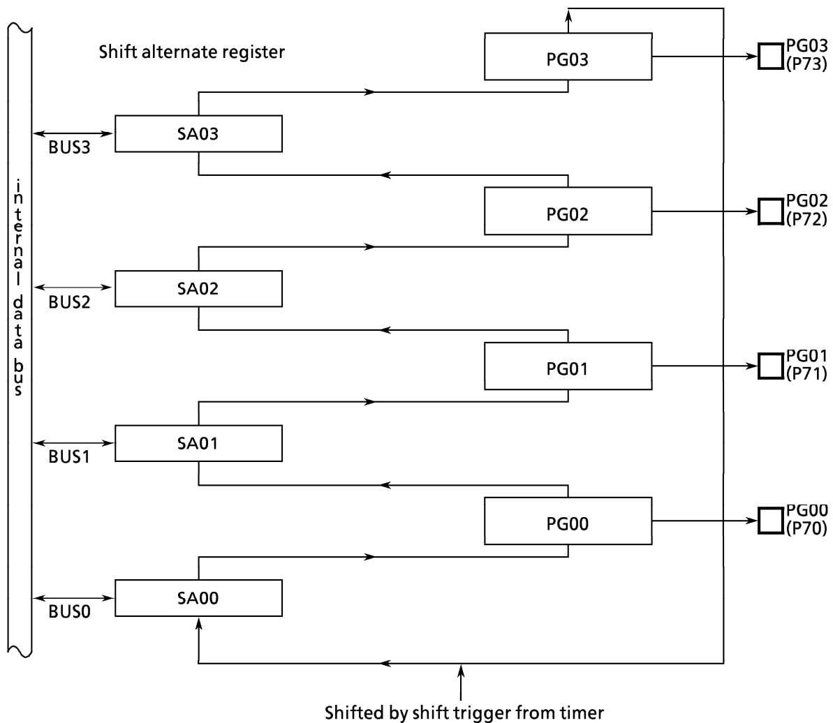
Figure 3,10 (7) Block Diagram of Pattern Generation Mode (PG0)
