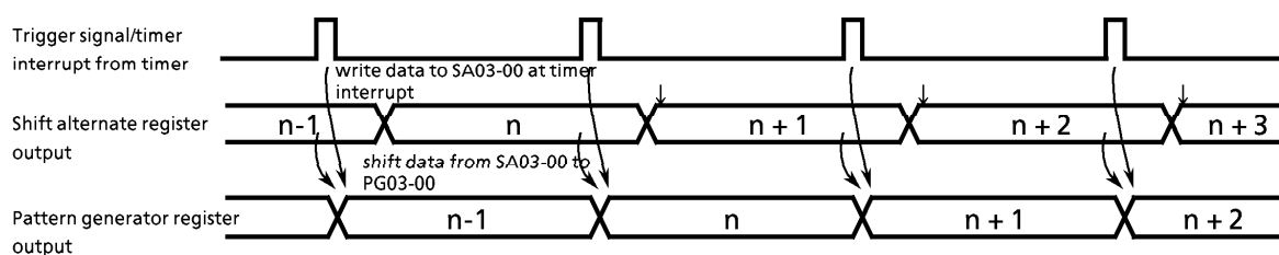
Example of Pattern Generation Mode Timing
