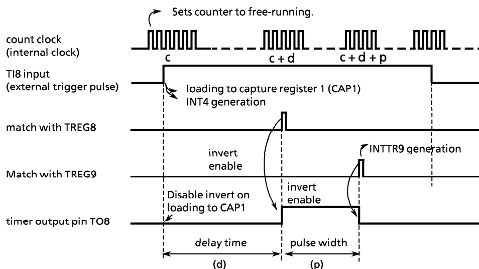
Figure 3.9 (13) One-Shot Pulse Output (With Delay)
