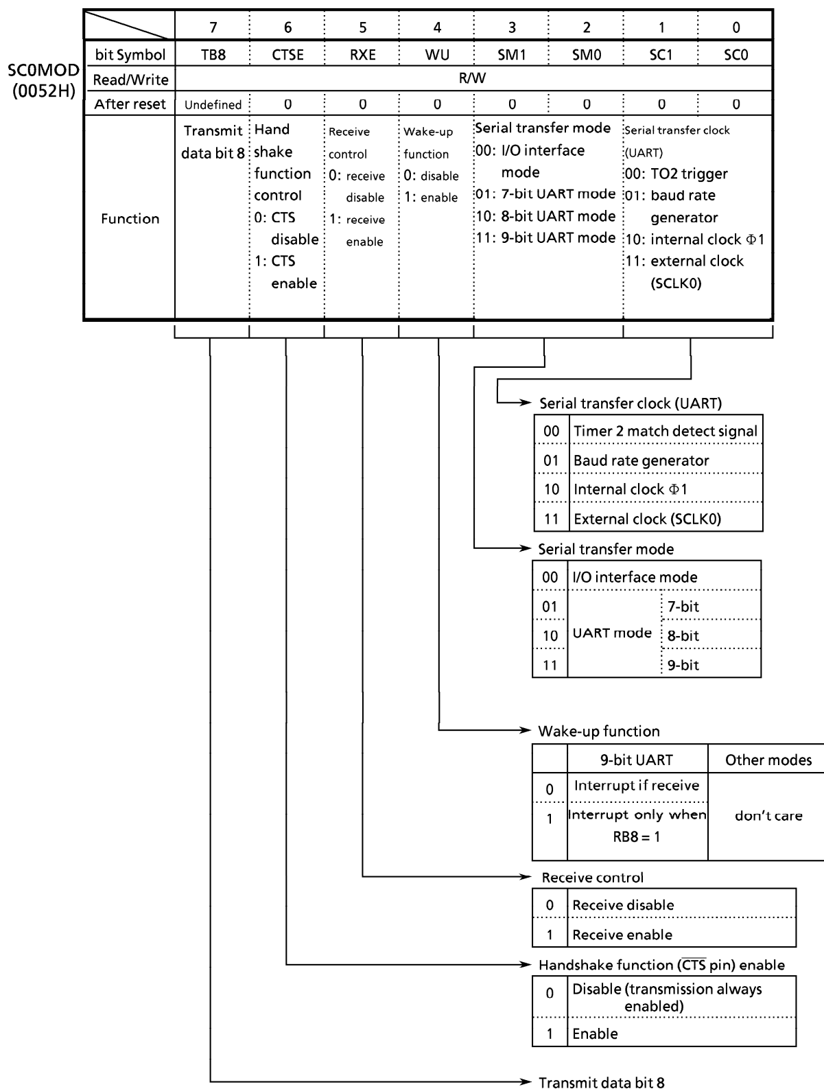
Figure 3.11 (2) Serial Mode Control Register (SC0MOD, Channel 0)
