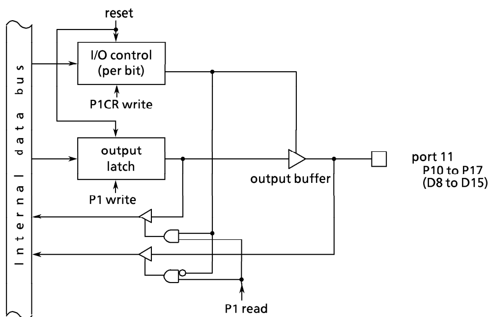
Figure 3.5 (1) Port 1
