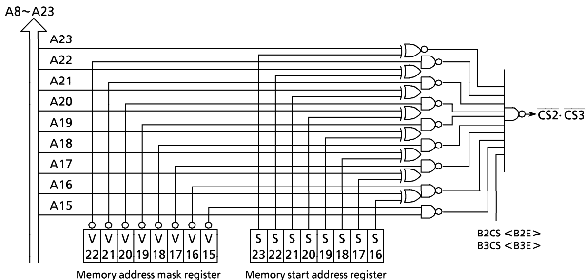
Figure 3.6 (7) \overline{CS2} and \overline{CS3} Address Decoder Block Diagram
