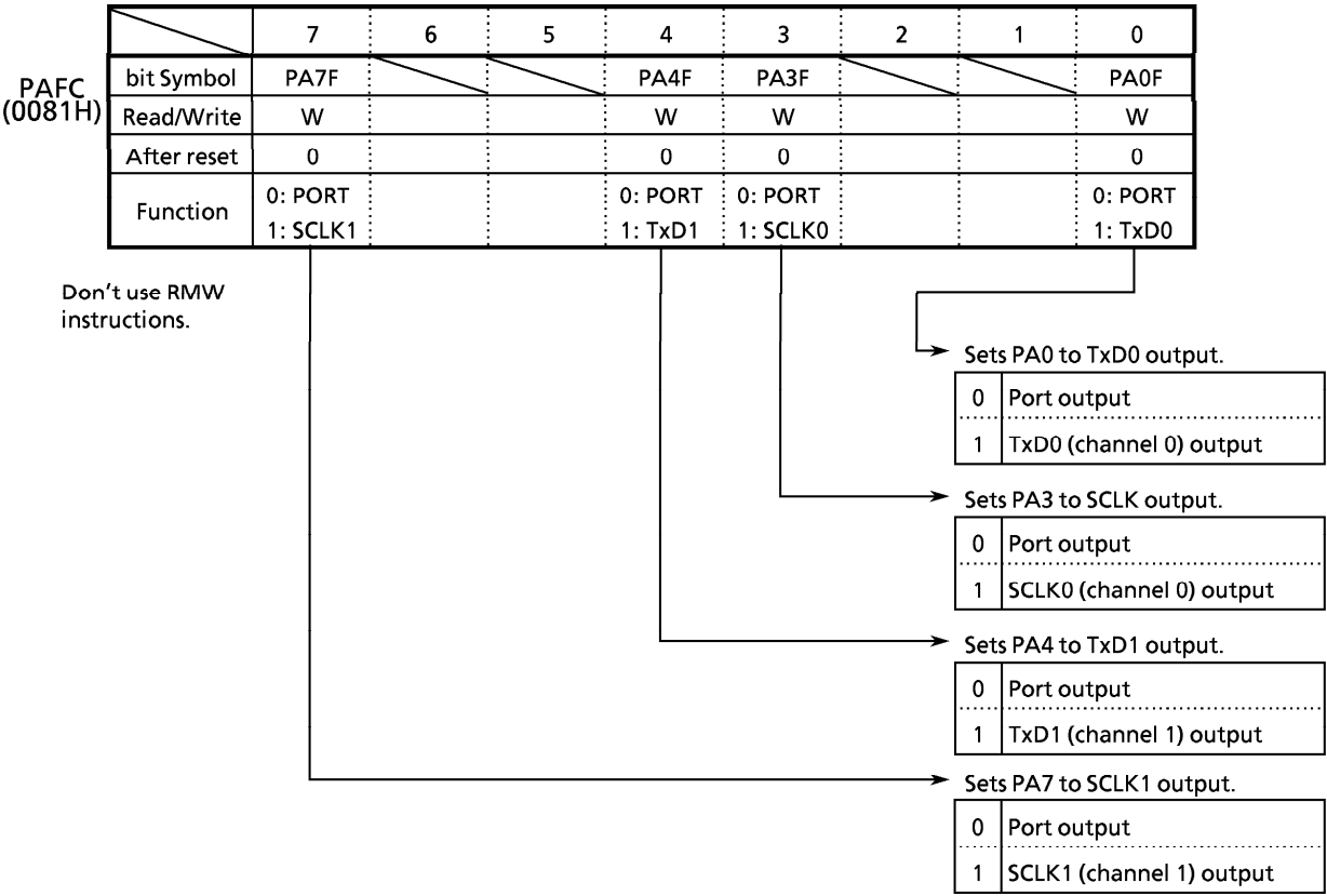
Figure 3.11 (10) Port A Function Register (PAFC)
