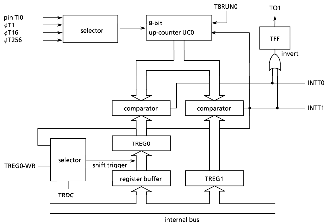
Figure 3.8 (16) 8-Bit PPG Output Mode Block Diagram
