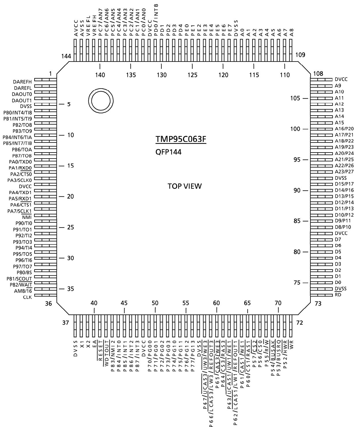
Figure 2.1 Pin Assignment
