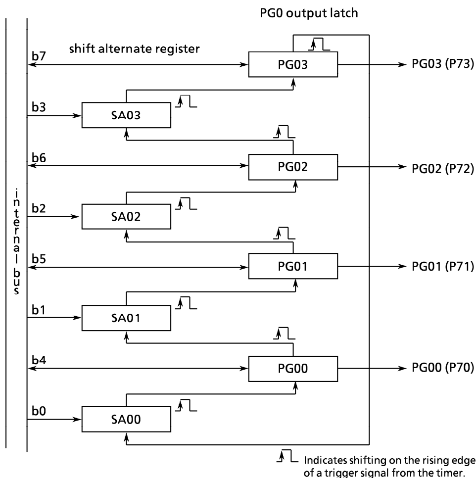
Figure 3.10 (12) 4-Phase, 1-2 Excitation (Normal)
