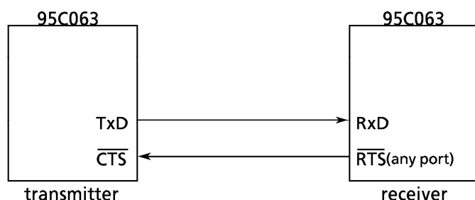
Figure 3.11 (14) Handshake Function
