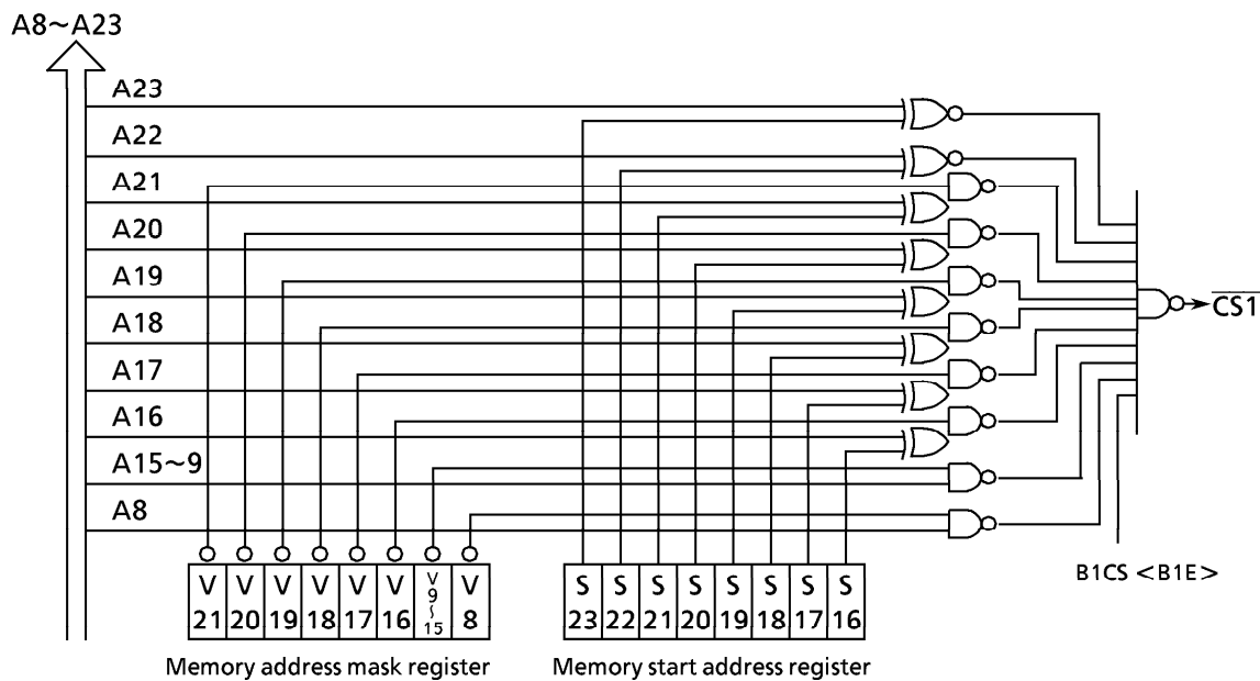
Figure 3.6 (6) \overline{CS1} Address Decoder Block Diagram
