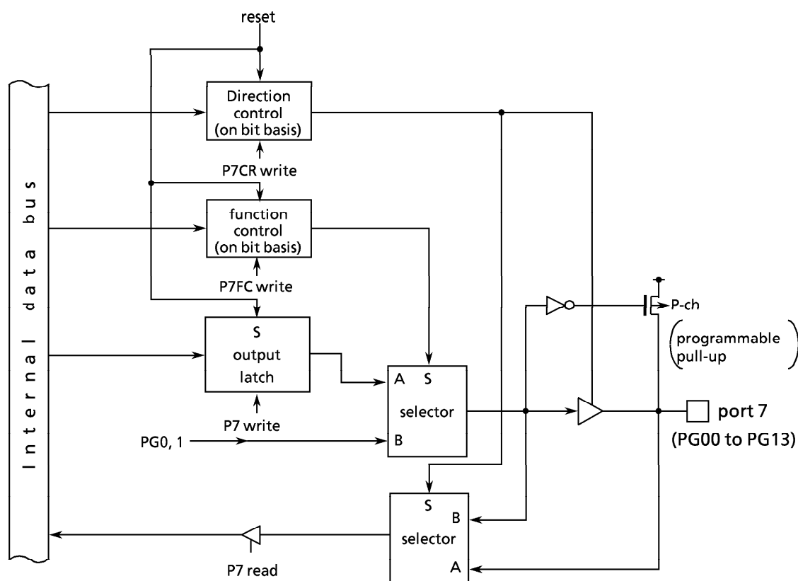
Figure 3.5 (10) Port 7
