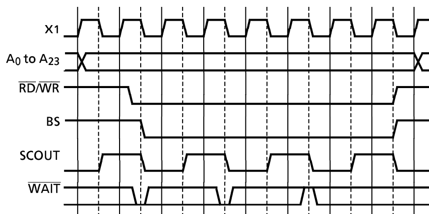
Figure 3.6 (3) 0 + N WAIT Read / Write Cycle (N = 2)
