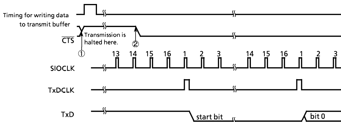
Figure 3.11 (14) Handshake Function
