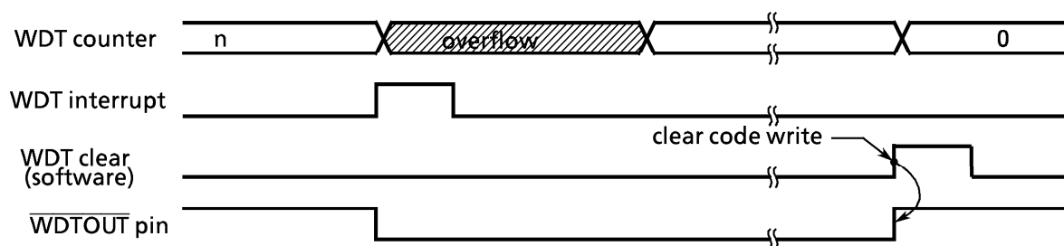
Figure 3.14 (2) Normal Mode
