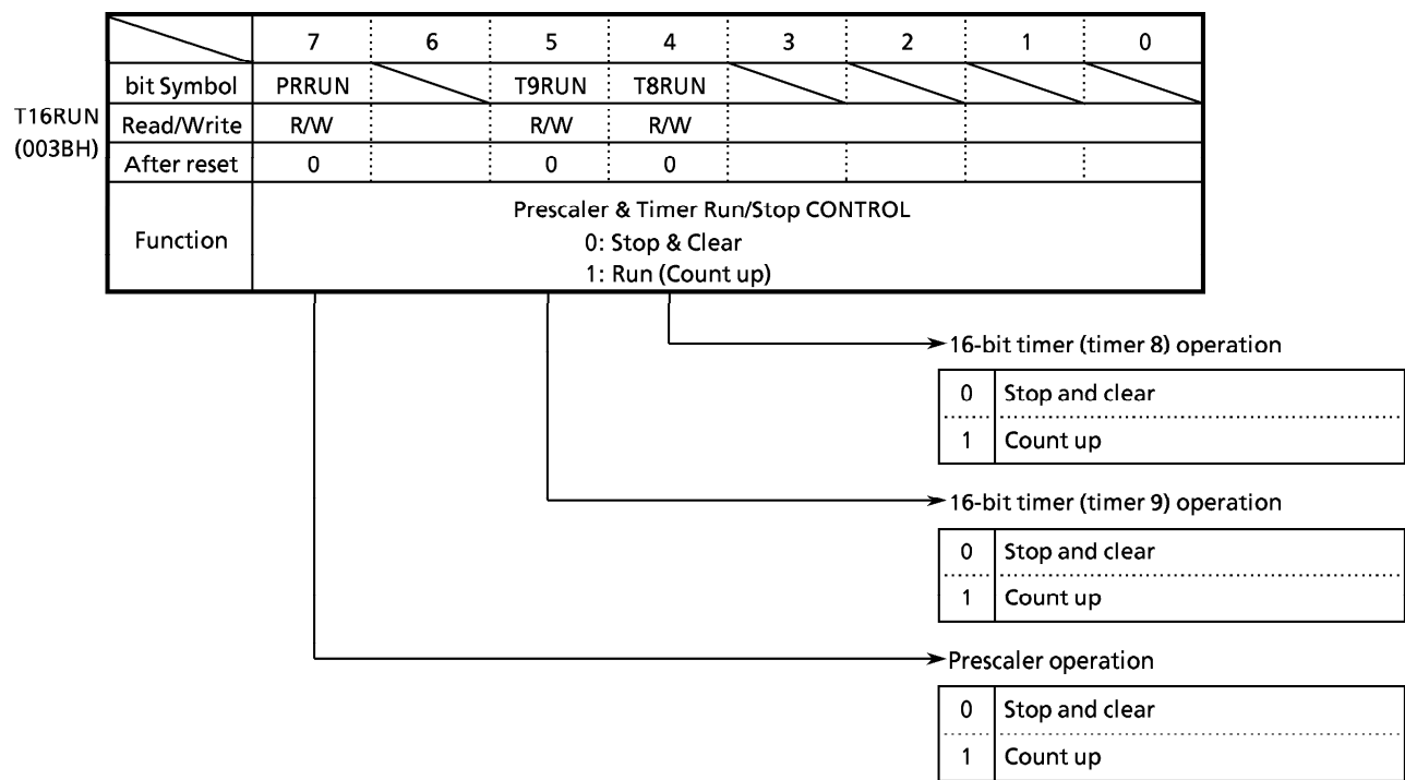
Figure 3.8 (11) 16-Bit Timer Operation Control Register (T16RUN)
