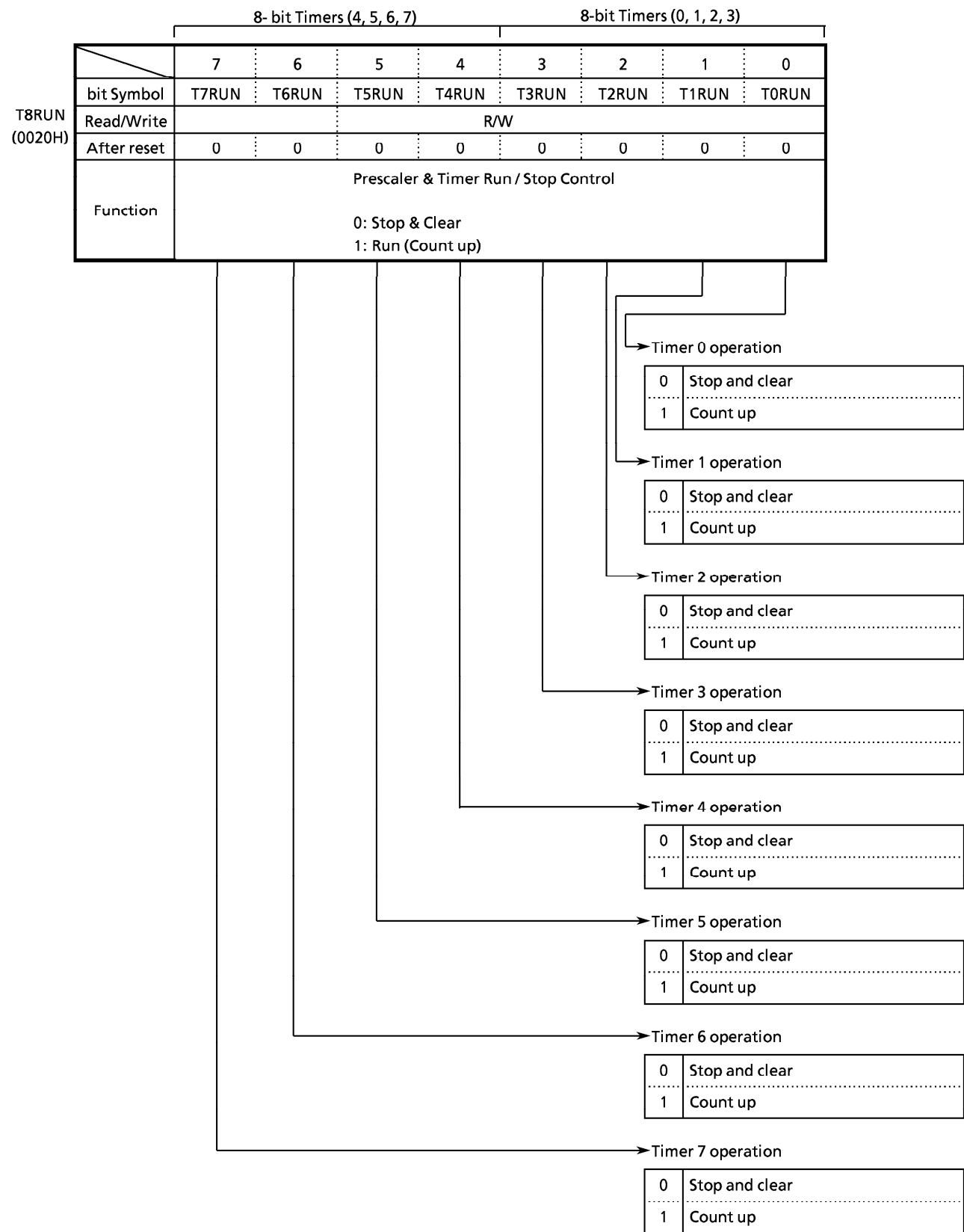
Figure 3.8 (10) 8-Bit Timer Operation Control Register (T8RUN)
