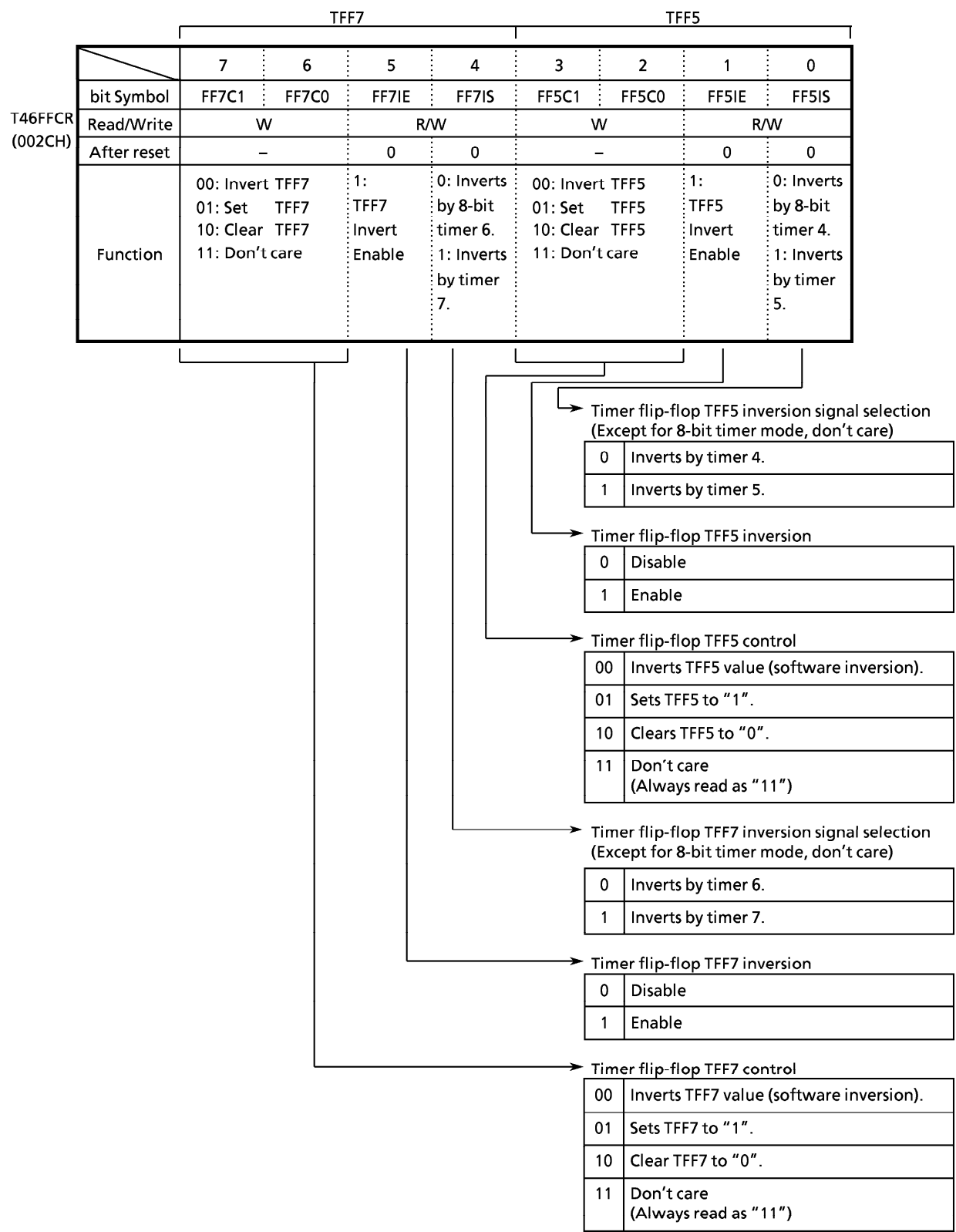
Figure 3.8 (9) 8-Bit Timer Flip-Flop Control Register (T46FFCR)
