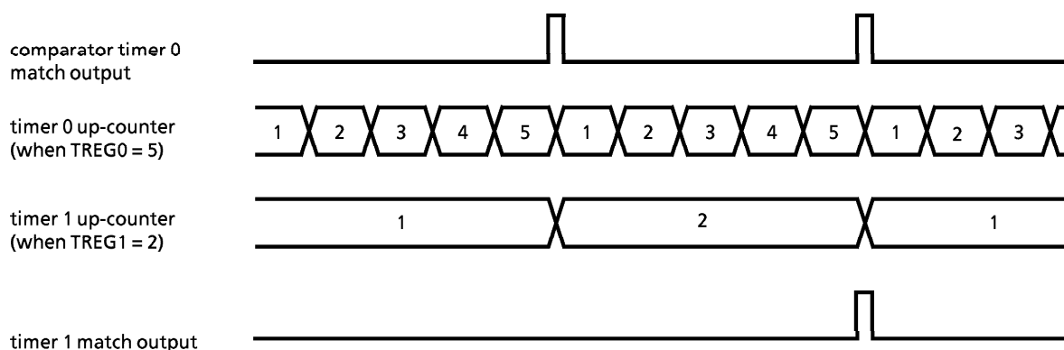
Figure 3.8 (14)
