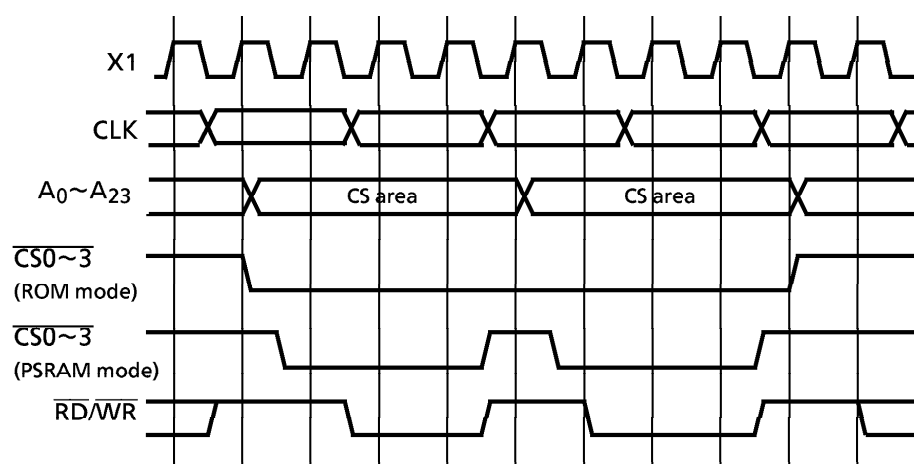
Figure 3.6 (4) Chip Select ( \overline{CS0} - \overline{CS3} ) Timing (ROM Mode and PSRAM Mode)
