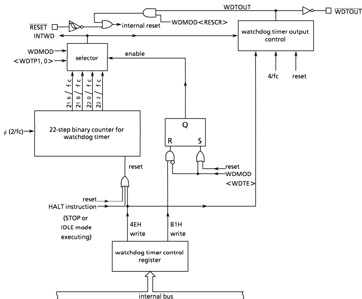
Figure 3.14 (1) Watchdog Timer Block Diagram
