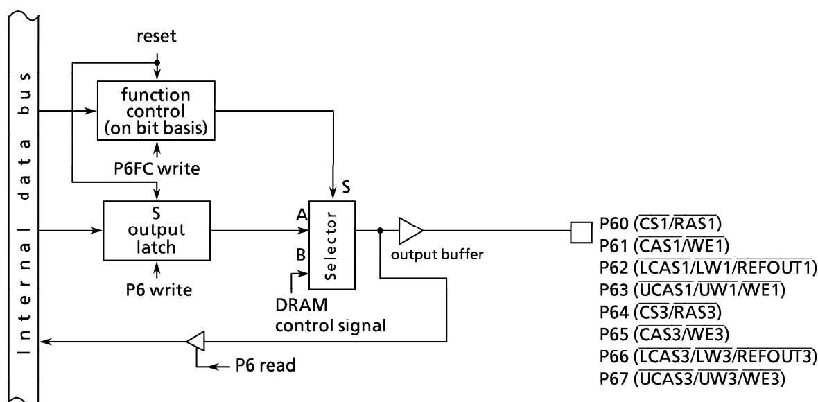
Figure 3.5 (8) Port 6
