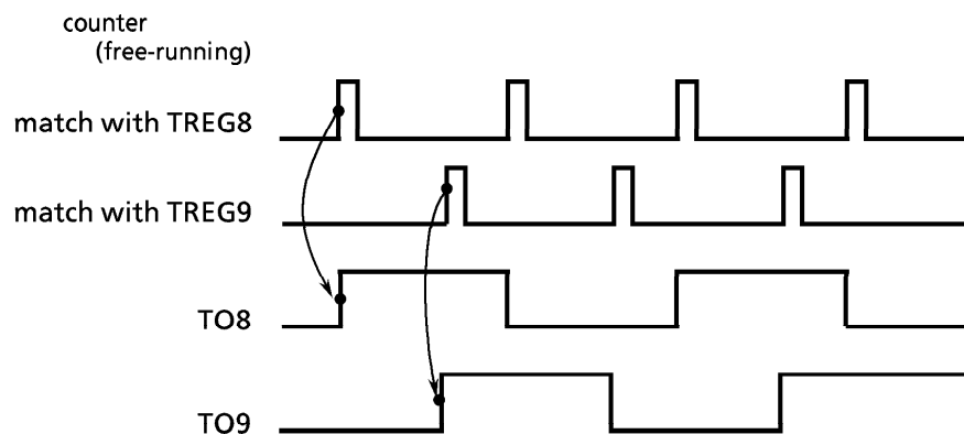
Figure 3.9 (18) Phase Output
