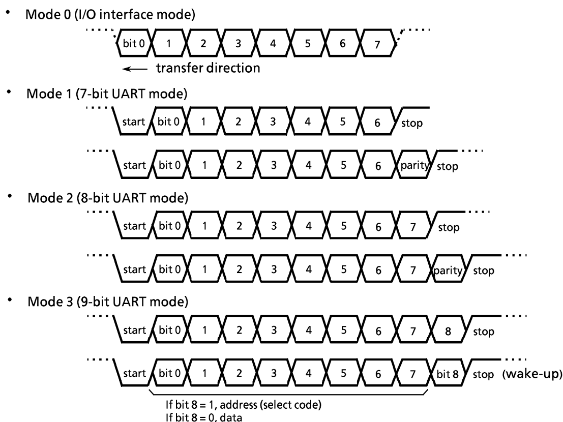
Figure 3.11 (1) Data Formats
