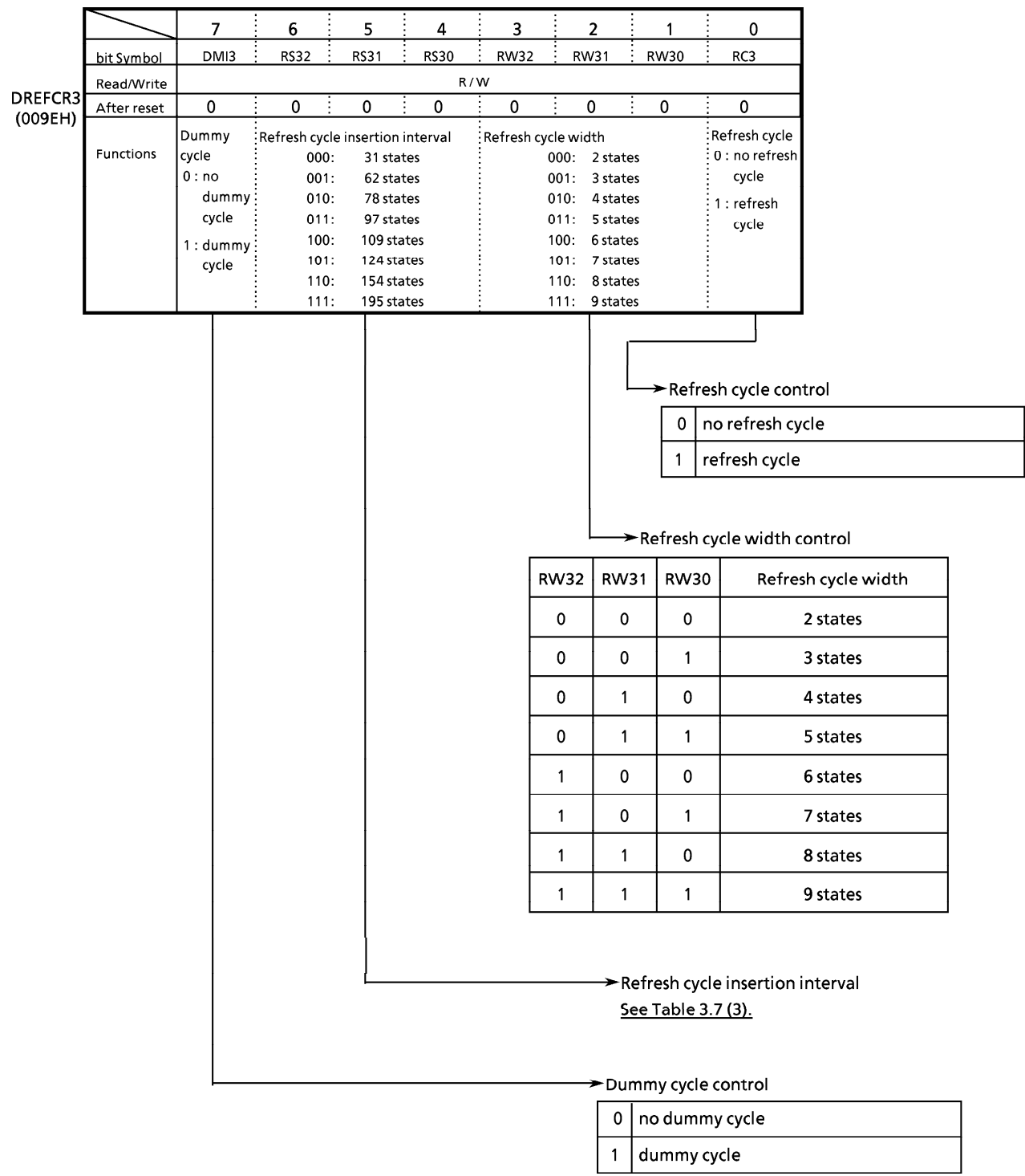
Figure 3.7 (2) (a) Refresh Control Register
