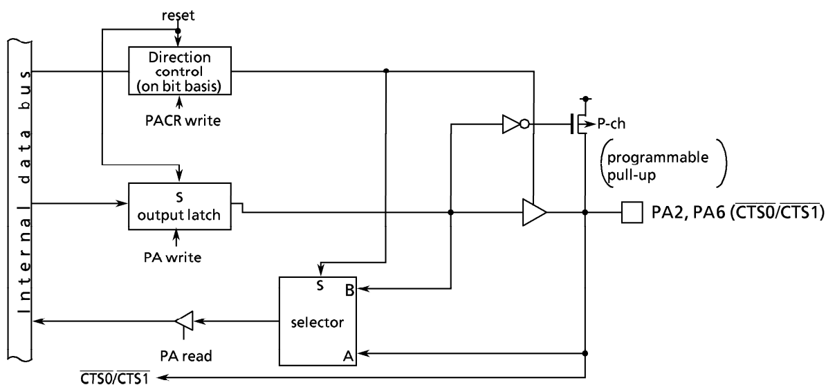
Figure 3.5 (20) Port A : PA2 and PA6
