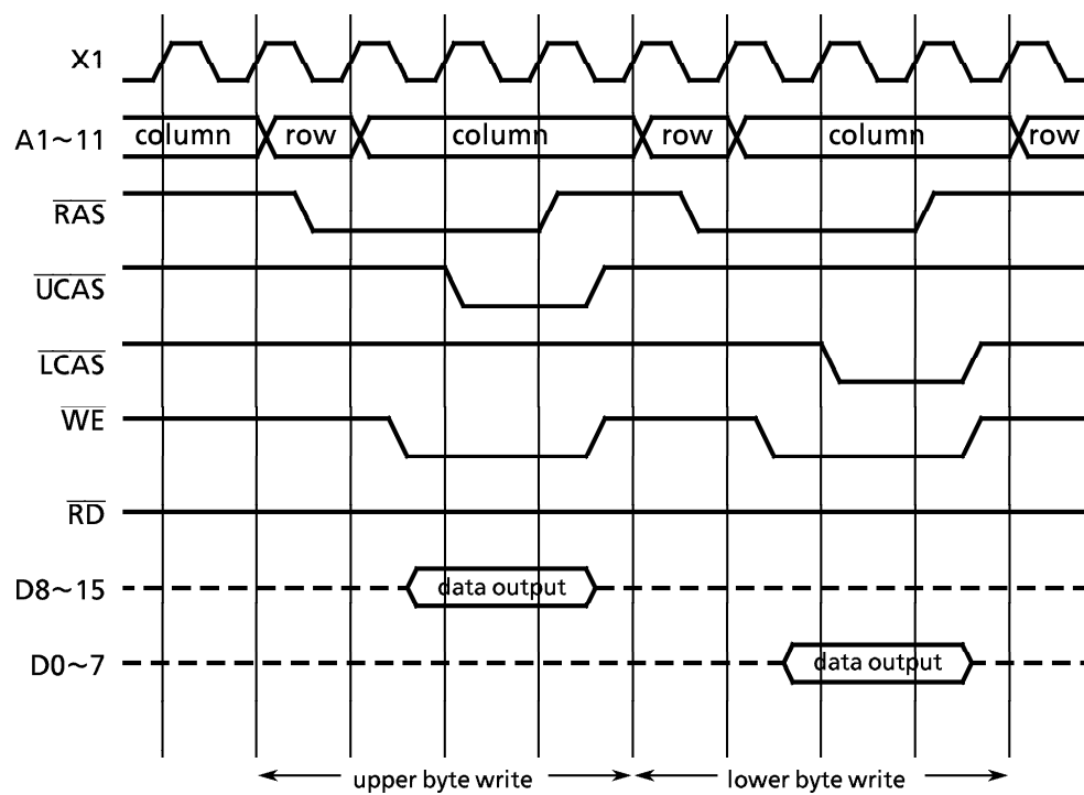
Figure 3.7 (3) (c) DRAM Access Timing (2CAS Mode, Write Cycle, and Byte Access)
