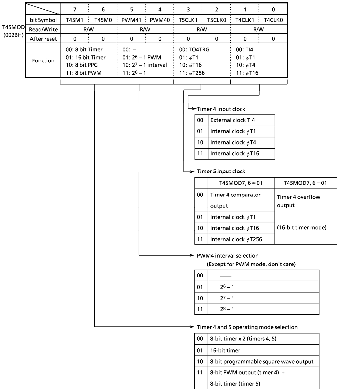
Figure 3.8 (6) Timer 4/5 Mode Register (T45MOD)
