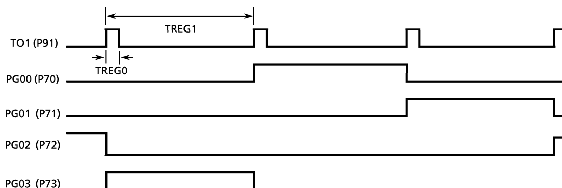
Figure 3.10 (13) 4-Phase, 1 Excitation Output Waveform
