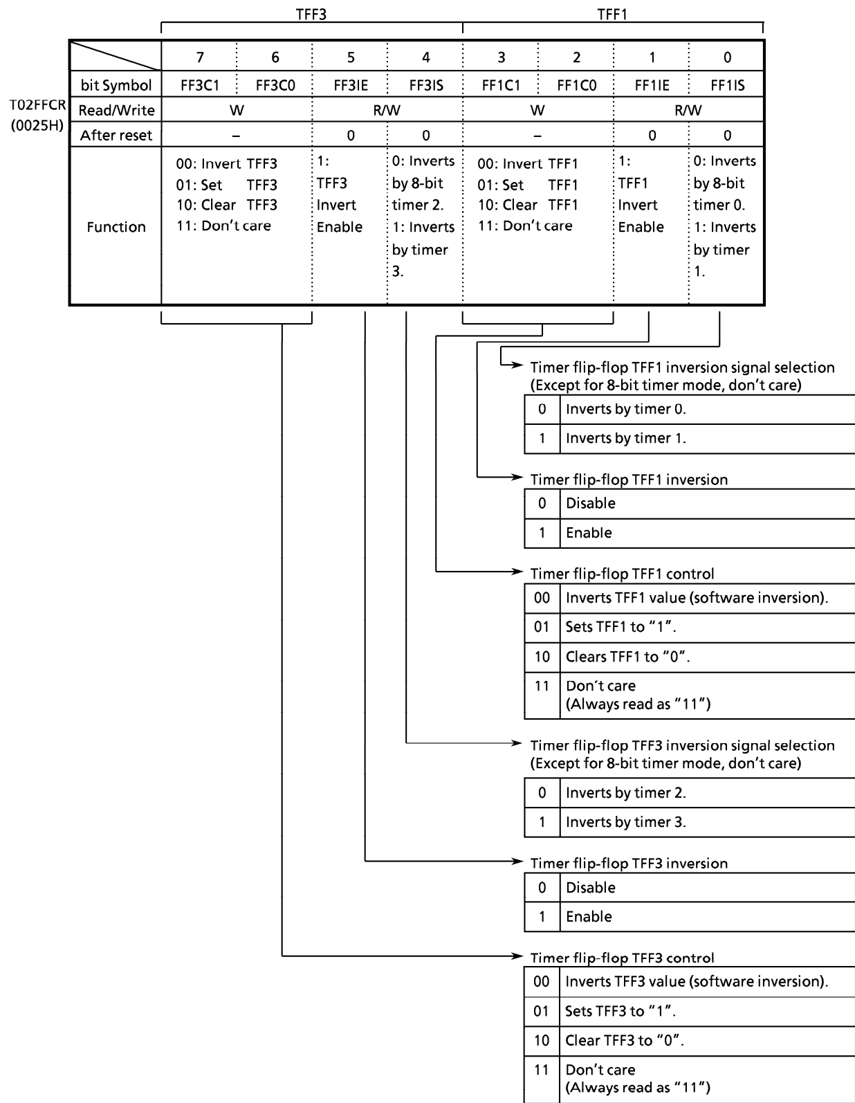
Figure 3.8 (8) 8-Bit Timer Flip-Flop Control Register (T02FFCR)
