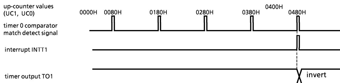
Figure 3.8 (15) Timer Output for 16-Bit Timer Mode
