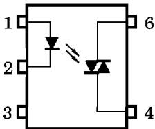
PIN CONFIGURATIONS (TOP VIEW)
