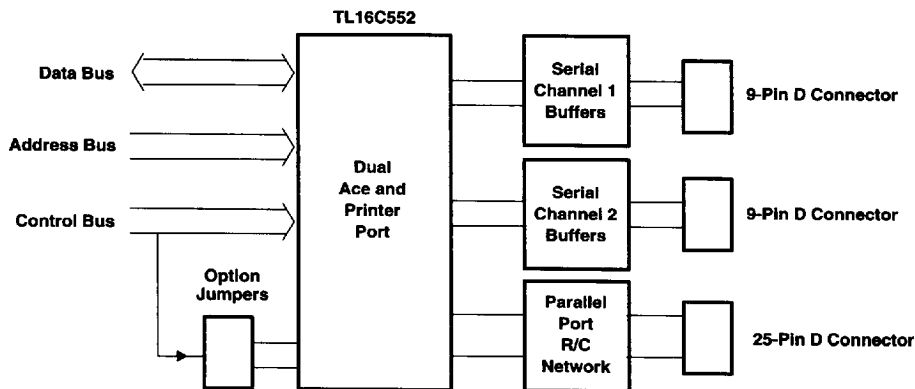
Figure 3. Basic Test Configuration
