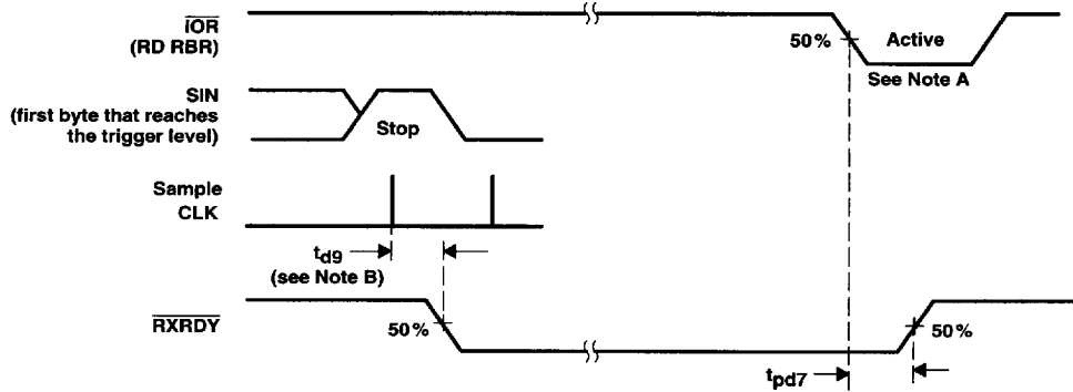
Figure 13. Receiver Ready Mode 1 Waveforms
