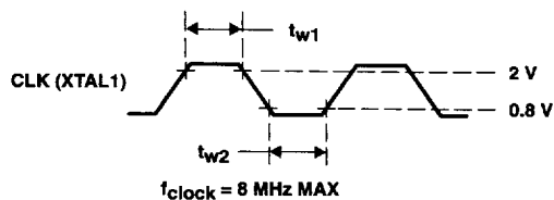
Figure 1. Clock Input (CLK) Voltage Waveform
