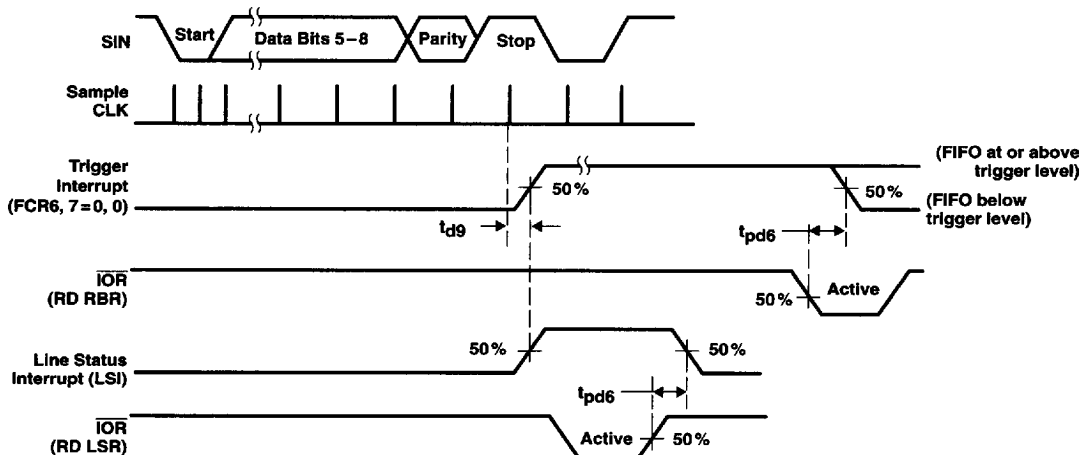
Figure 10. Receiver FIFO First Byte (Sets RDR) Waveforms
