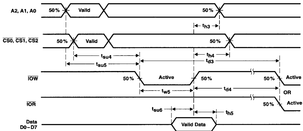
Figure 5. Write Cycle Timing Waveforms
