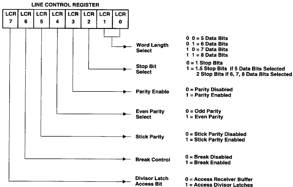
Figure 17. Line Control Register Contents
