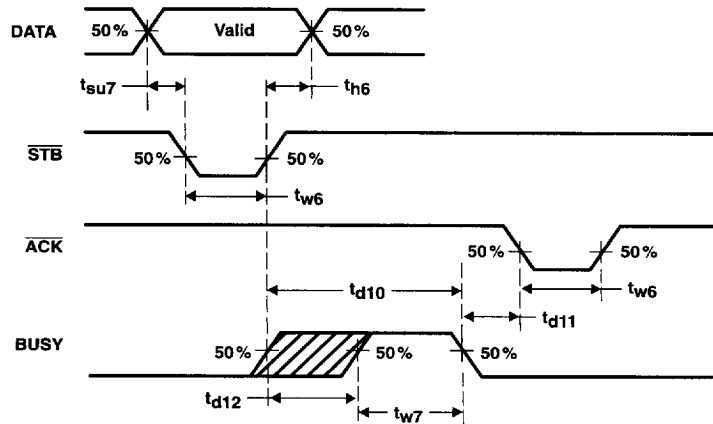
Figure 15. Parallel Port Timing Waveforms
