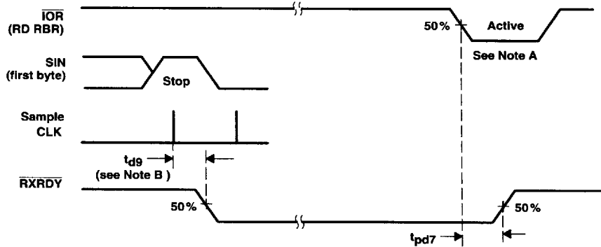
Figure 12. Receiver Ready Mode 0 Waveforms
