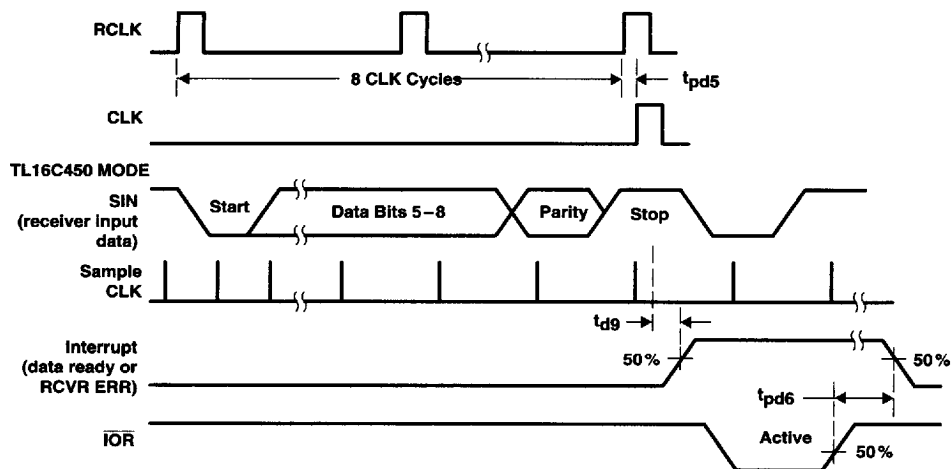
Figure 9. Receiver Timing Waveforms
