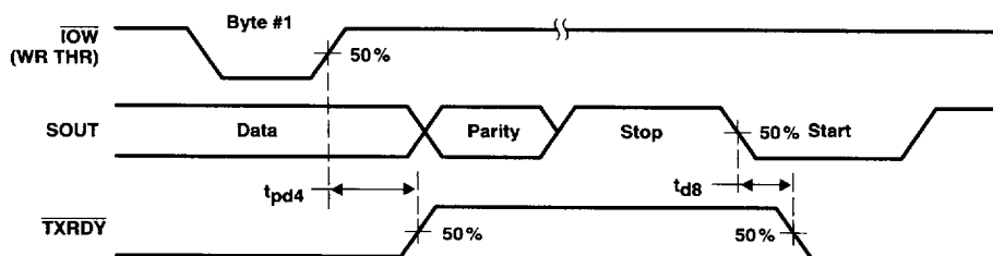
Figure 7. Transmitter Ready Mode 0 Timing Waveforms
