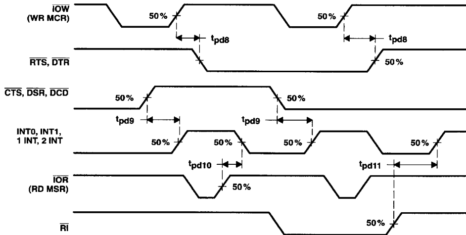
Figure 14. Modem Control Timing Waveforms
