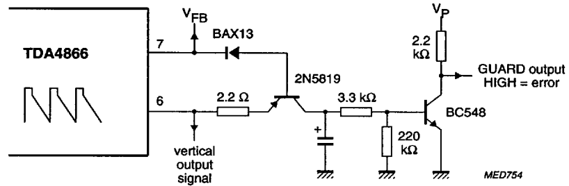
Fig.6 Application circuit for external guard signal generation.
