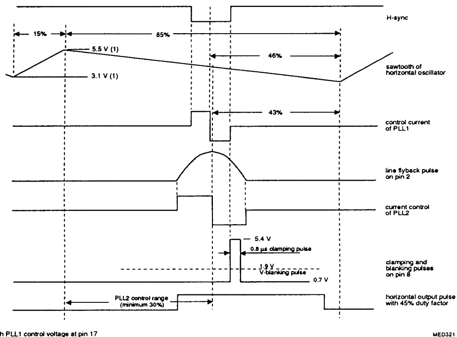
Fig.6 Horizontal timing diagram.
