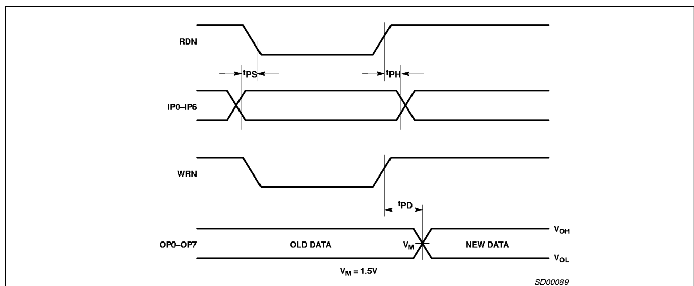
Figure 5. Port Timing
