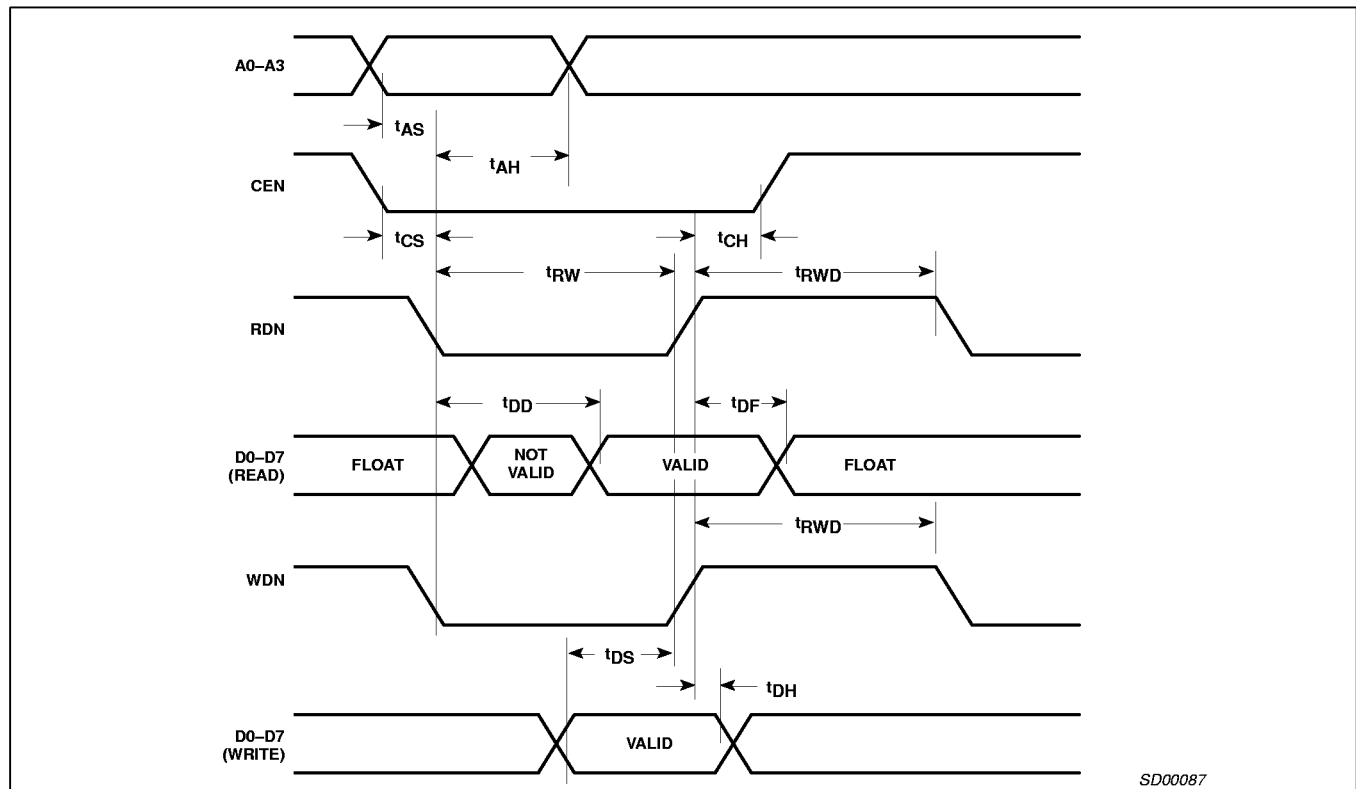
Figure 4. Bus Timing
