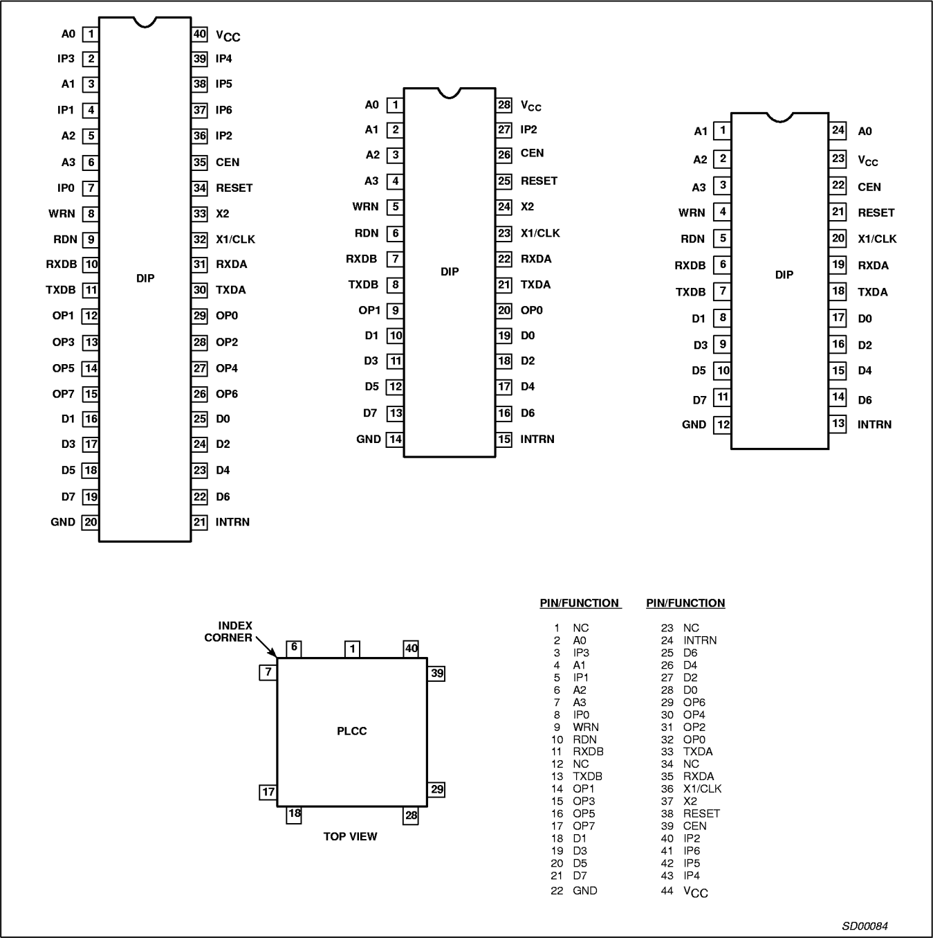
Figure 1. Pin Configurations
