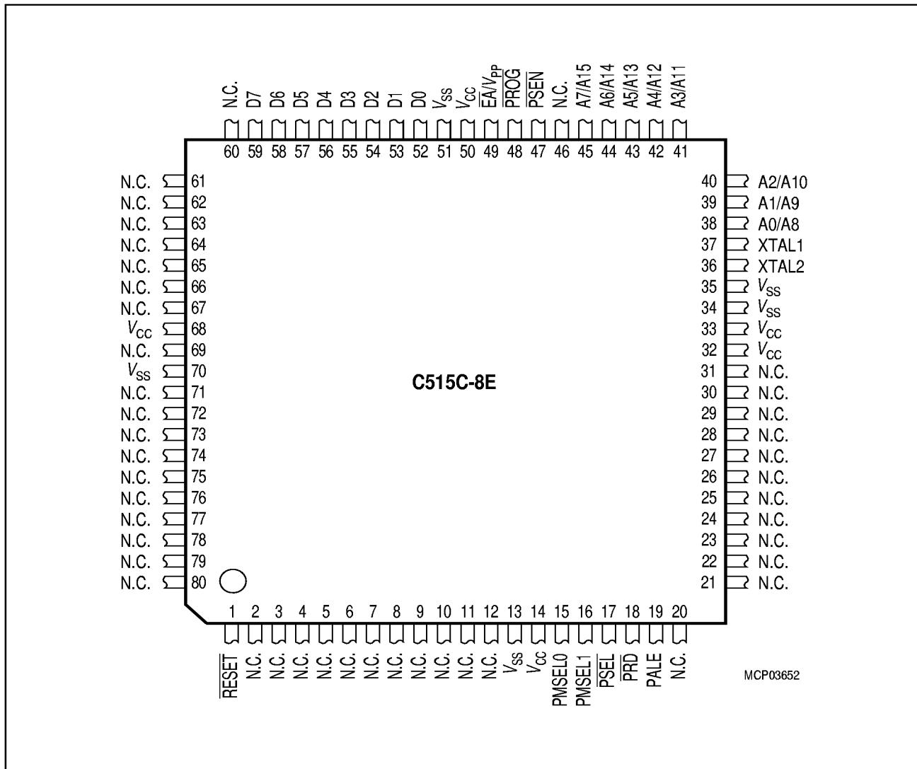
Figure 26 P-MQFP-80 Pin Configuration of the C515C-8E in Programming Mode (Top View)
