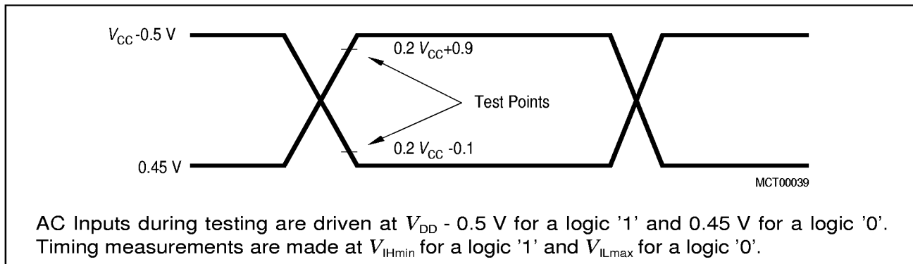
Figure 40 AC Testing: Input, Output Waveforms
