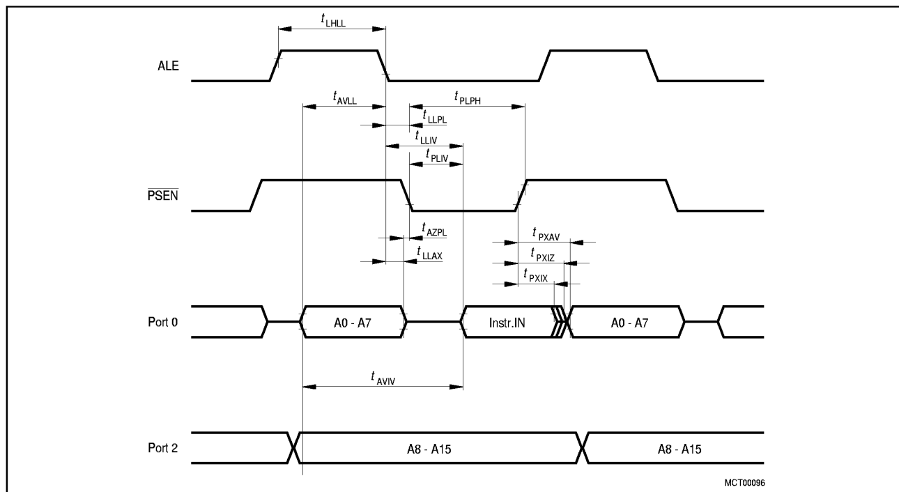
Figure 29 Program Memory Read Cycle
