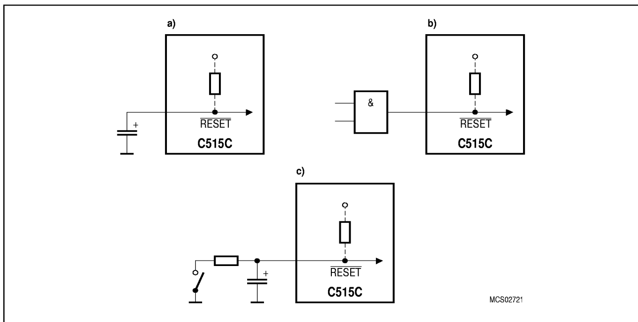
Figure 6 Reset Circuitries
