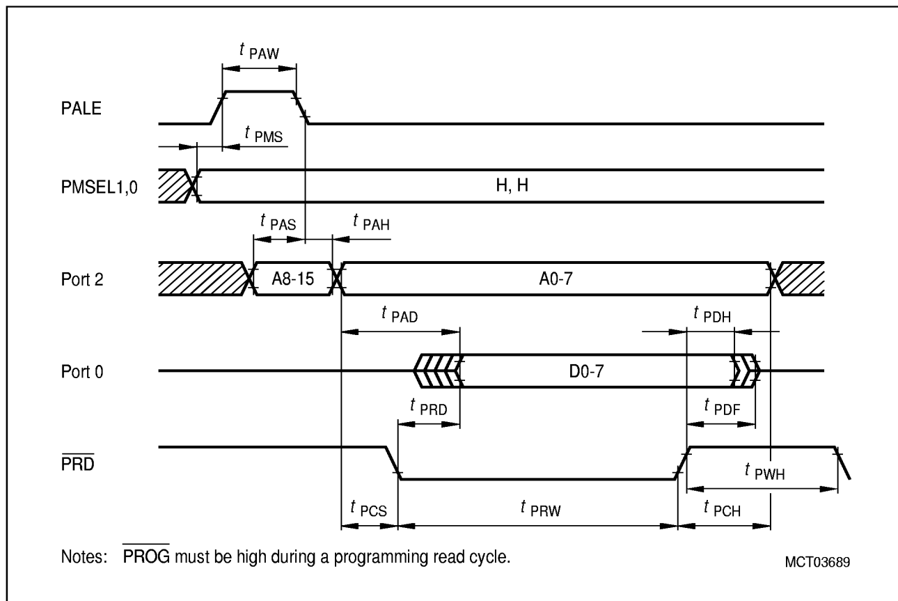
Figure 35 Verify Code Byte - Read Cycle Timing
