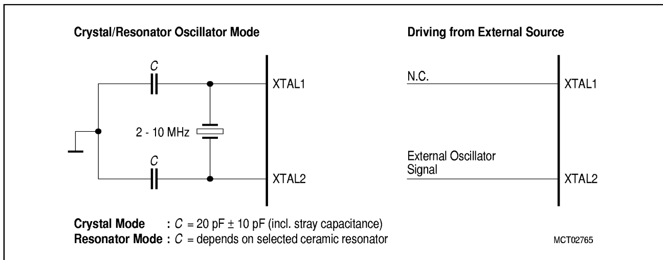
Figure 42 Recommended Oscillator Circuits for Crystal Oscillator
