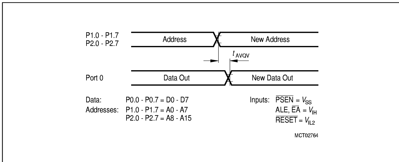
Figure 38 ROM Verification Mode 1
