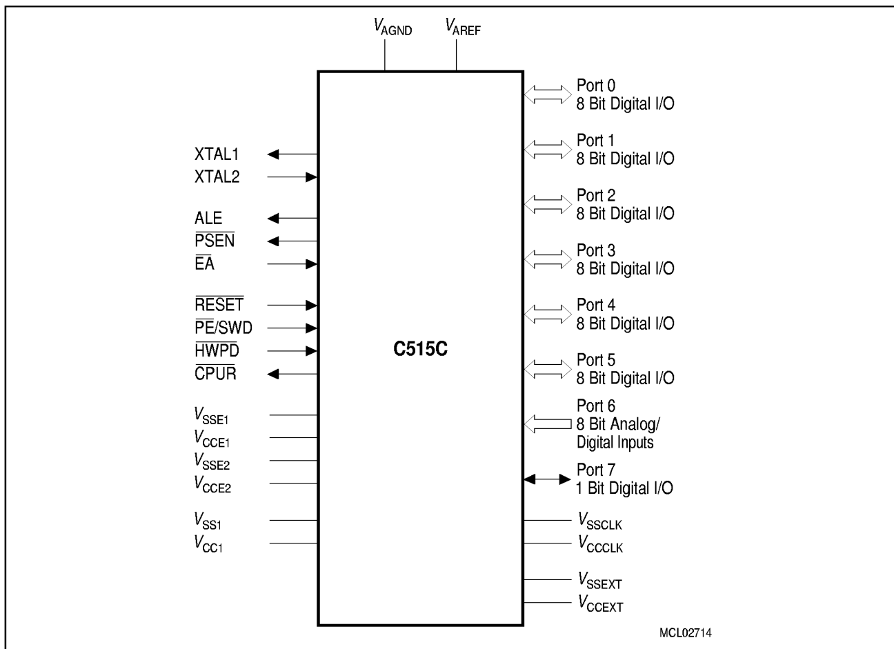
Figure 2 Logic Symbol
