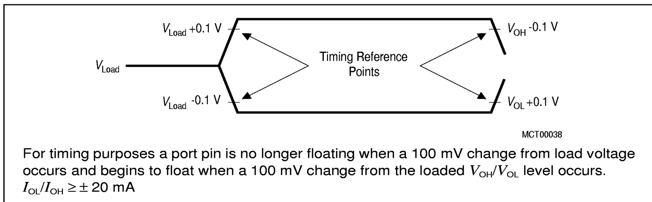
Figure 41 AC Testing : Float Waveforms
