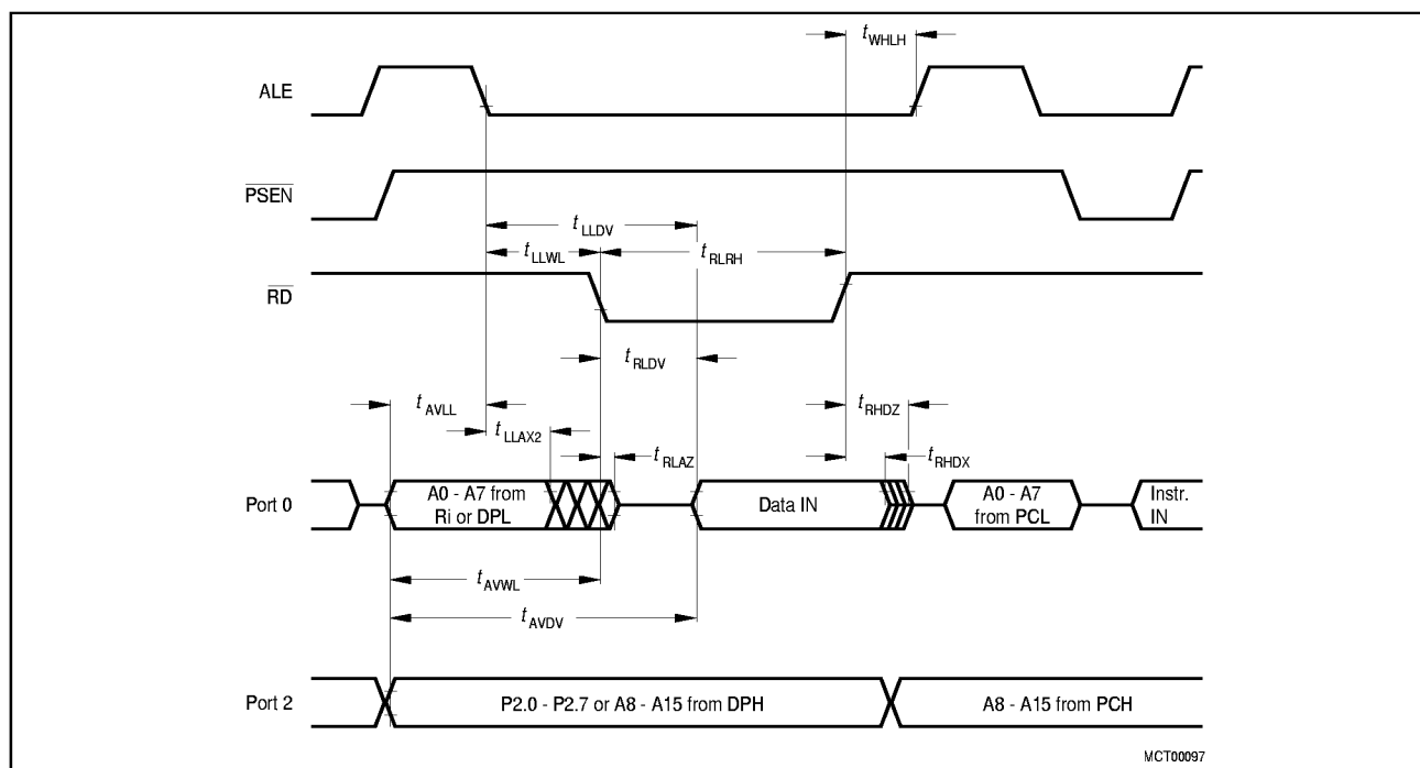
Figure 30 Data Memory Read Cycle
