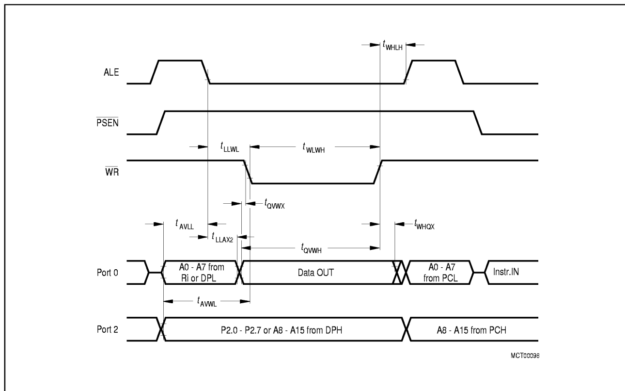
Figure 31 Data Memory Write Cycle
