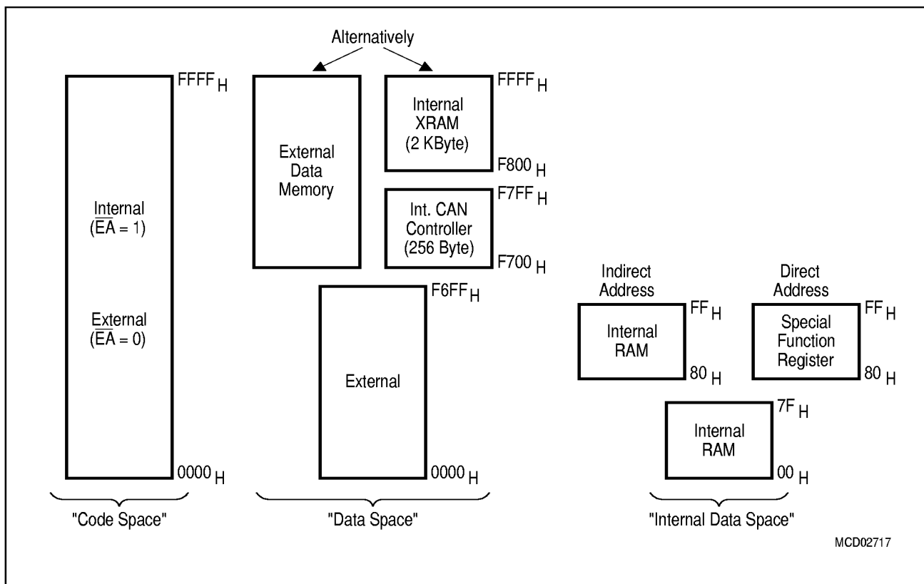
Figure 5 C515C Memory Map
