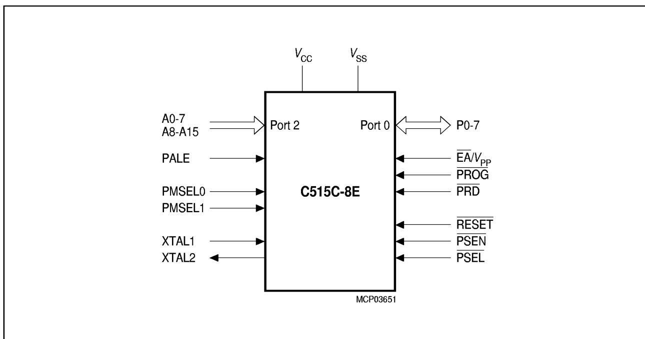
Figure 25 Programming Mode Configuration of the C515C-8E
