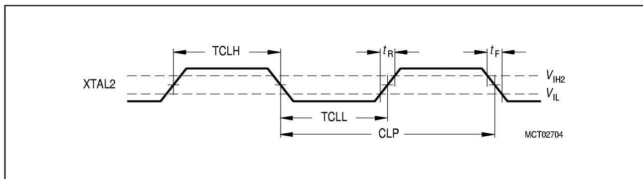
Figure 32 External Clock Drive at XTAL2
