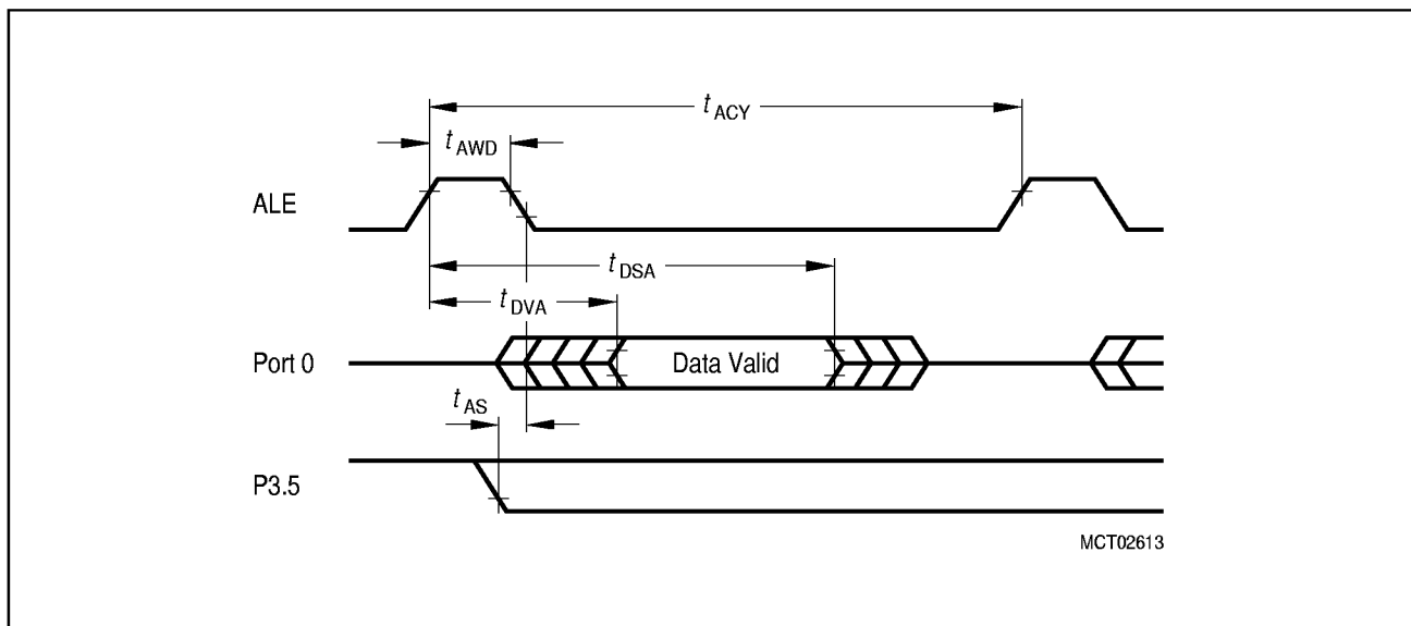
Figure 39 ROM/OTP Verification Mode 2
