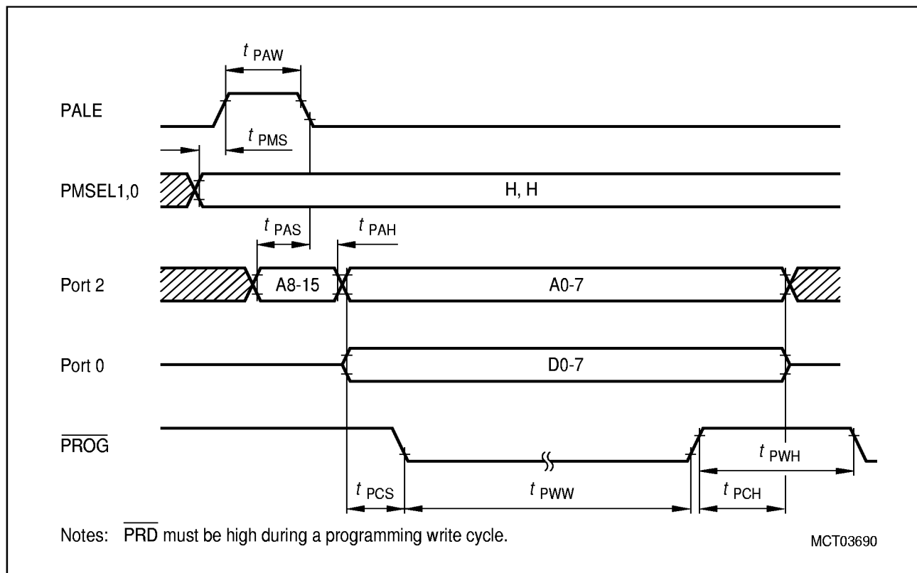
Figure 34 Programming Code Byte - Write Cycle Timing
