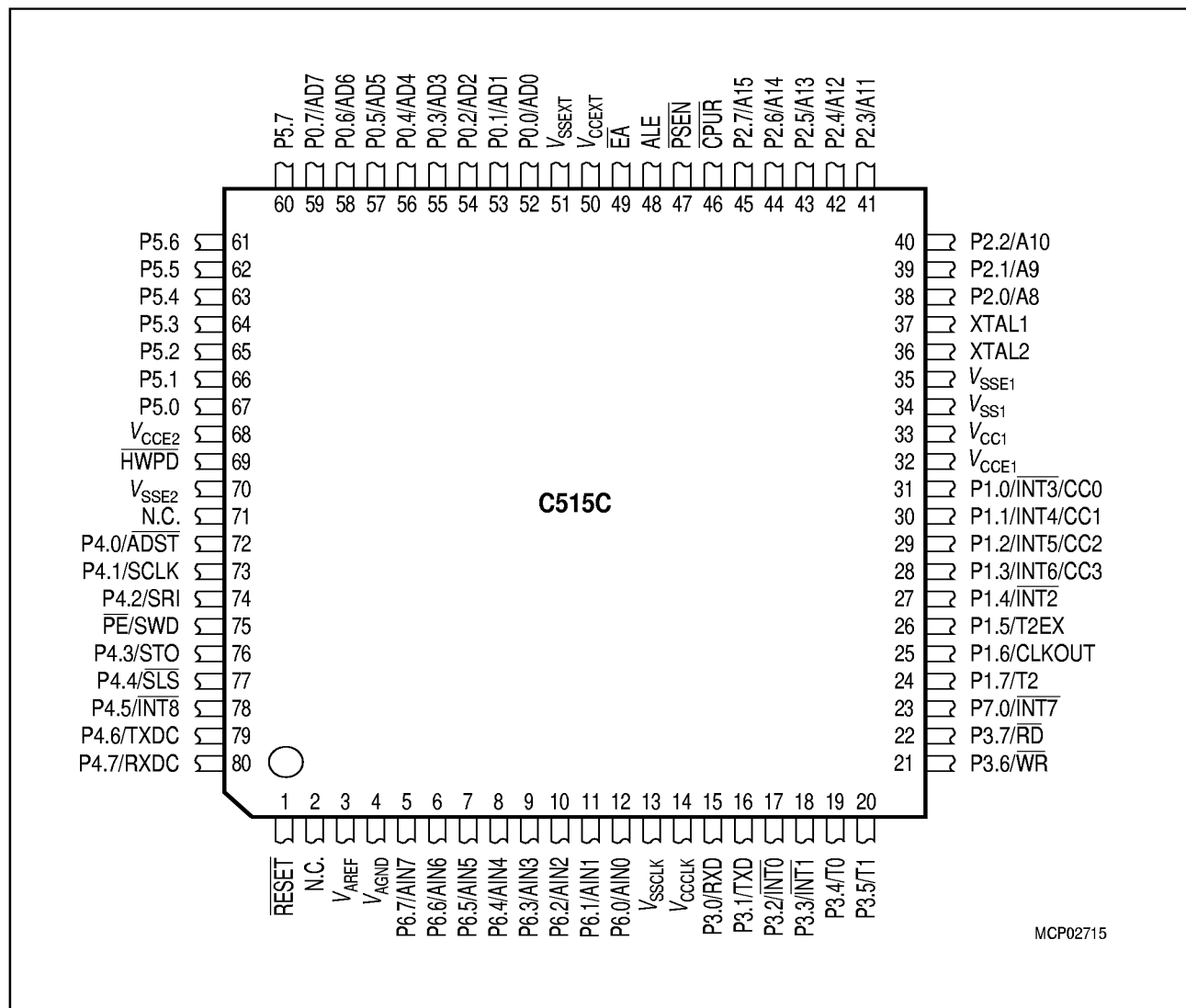
Figure 3 C515C Pin Configuration (P-MQFP-80-1, Top View)
