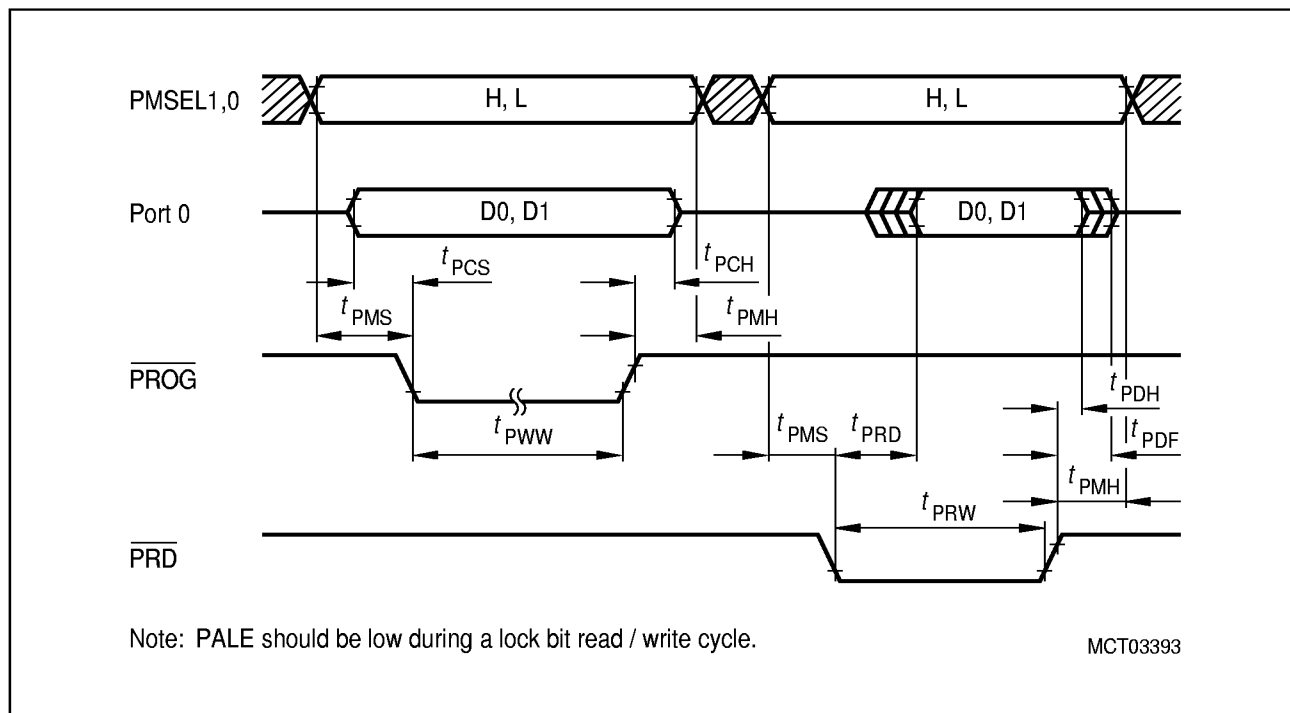
Figure 36 Lock Bit Access Timing
