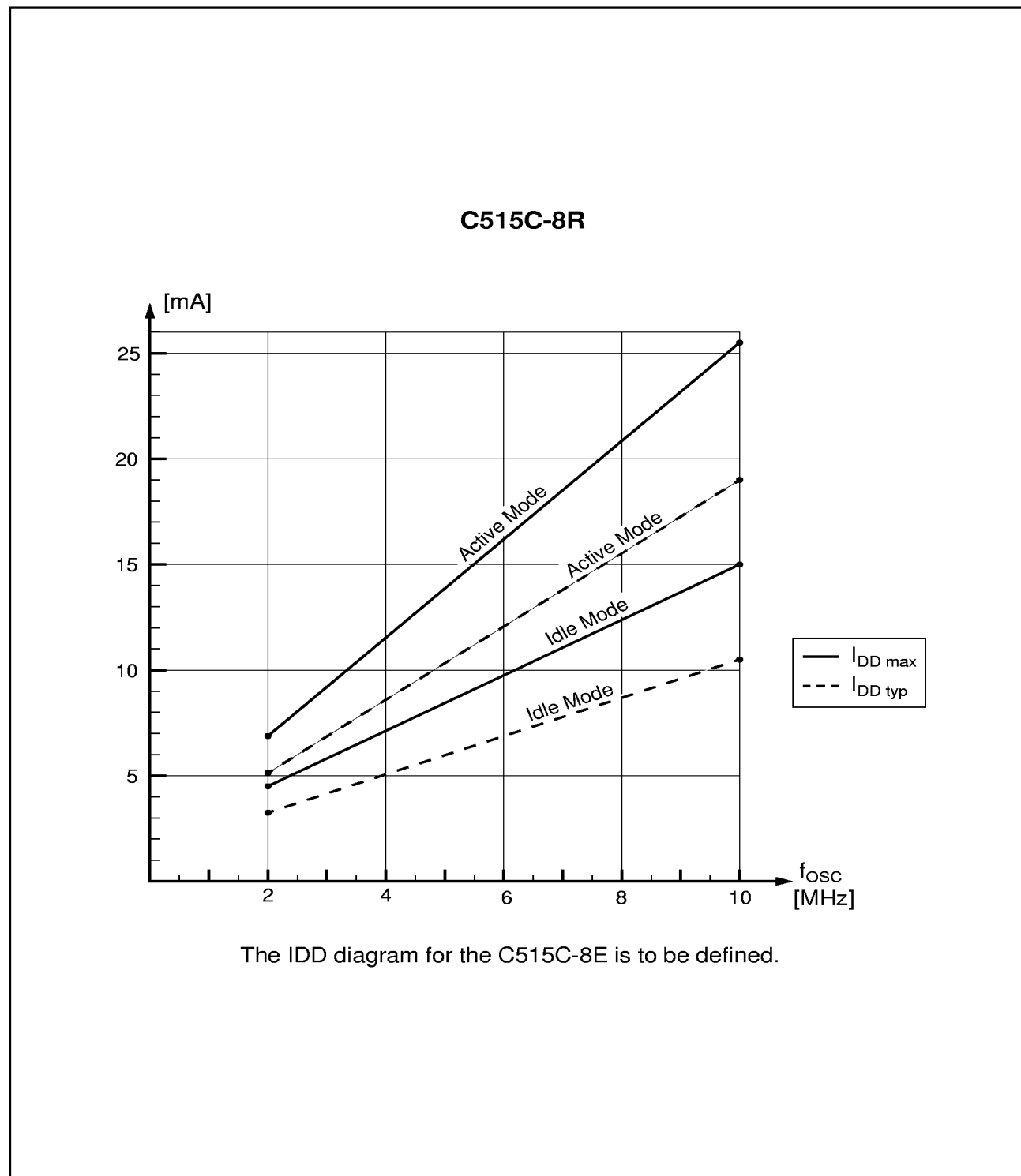
Figure 28 IDD Diagrams
