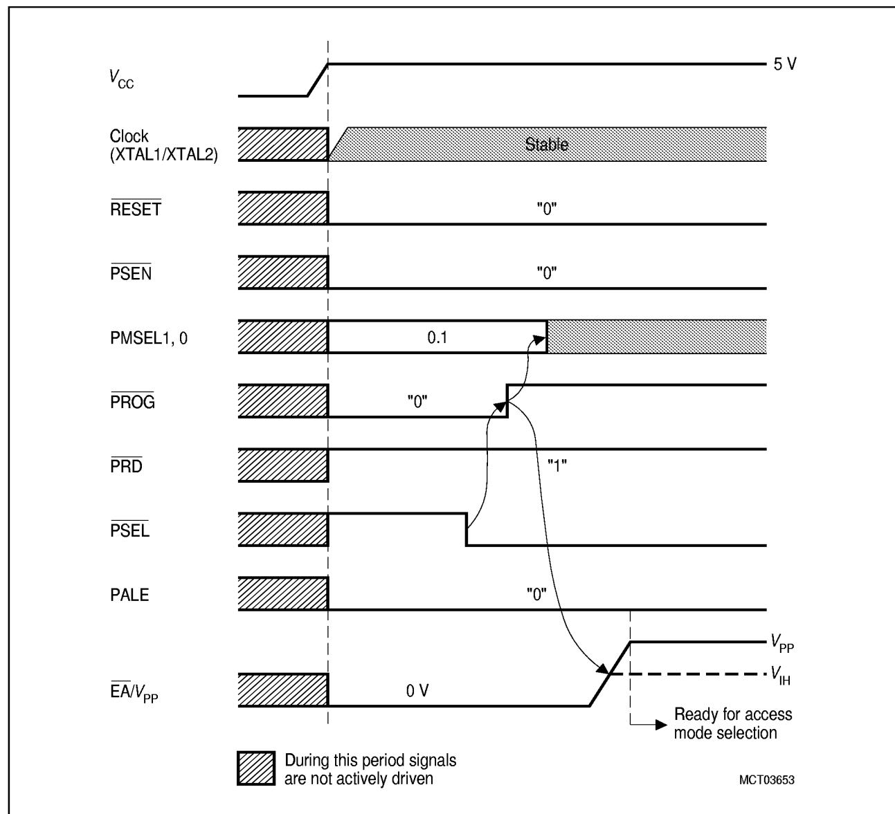
Figure 27 C515C-8E Basic Programming Mode Selection
