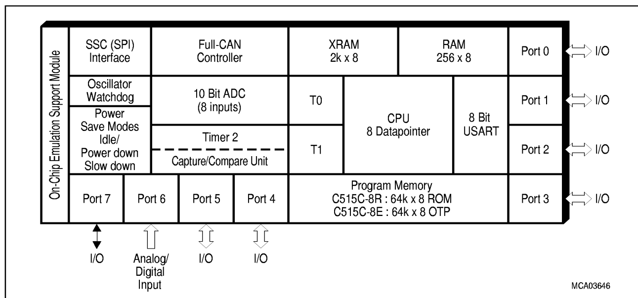
Figure 1 C515C Functional Units
