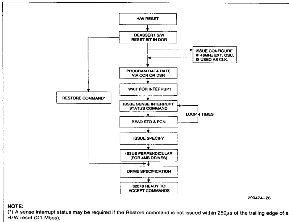
Figure 9-3. Initialization Flowchart
