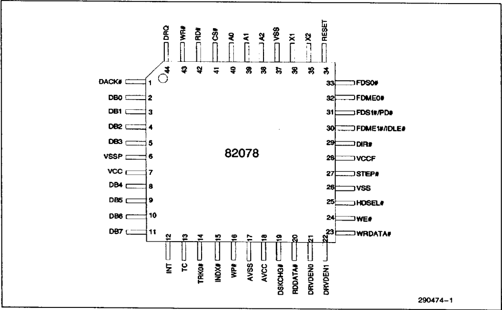
Figure 1-0. 82078 44 Pin Pinout
