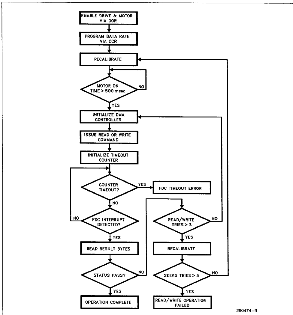
Figure 9-5. Read/Write Operation
