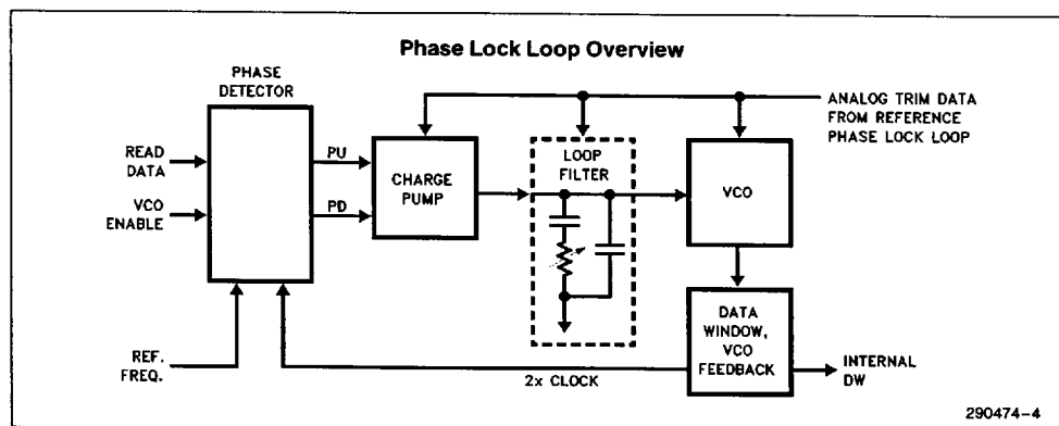
Figure 3-2. Data PLL
