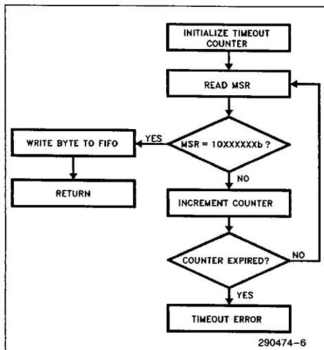
Figure 9-1. Send_byte Routine
