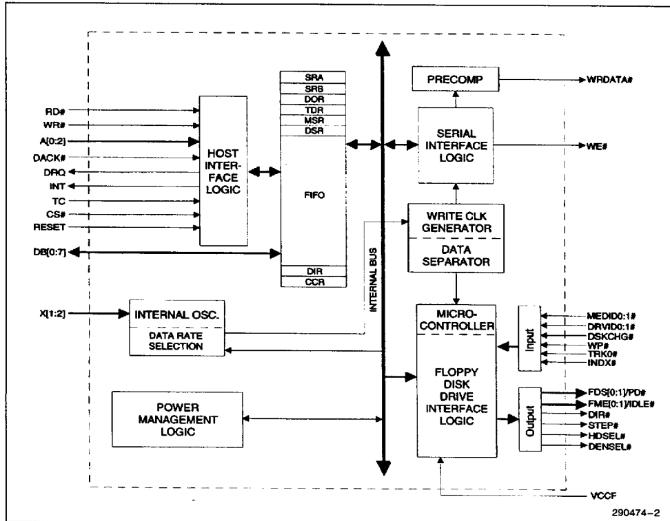
Figure 1-1. 82078 Block Diagram
