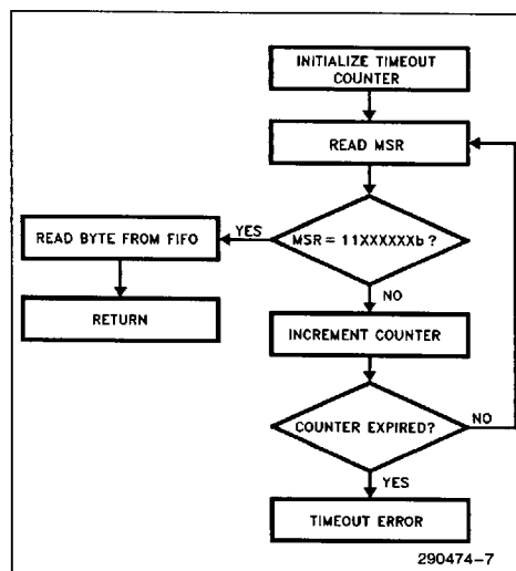
Figure 9-2. Get_byte Routine
