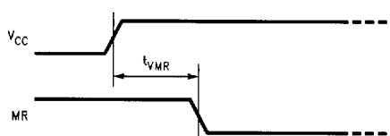
FIGURE 12-26. MR Timing
