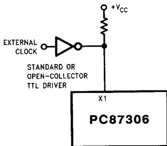
FIGURE 10-11. External Clock Connection
