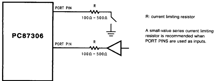
FIGURE 10-9. Using Port Pins as Inputs
