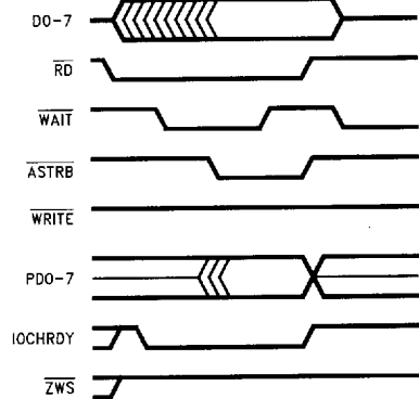
FIGURE 8-5. EPP 1.9 Address Read
