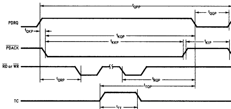
FIGURE 12-12. ECP DMA Timing
