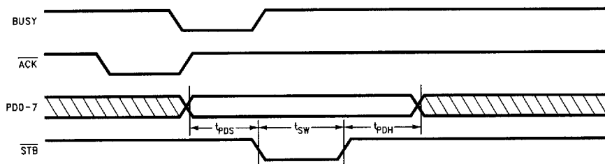
FIGURE 12-20. Typical Parallel Port Data Exchange
