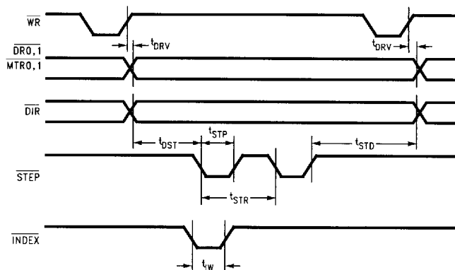
FIGURE 12-16. Drive Control Timing
