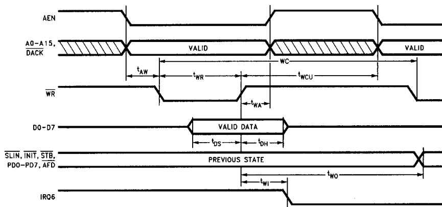
FIGURE 12-3. Microprocessor Write Timing
