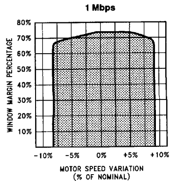
FIGURE 5-2. PC87306 Dynamic Window Margin Performance (Typical performance at V_{DD} = 5.0V , 25^{\circ}C )
