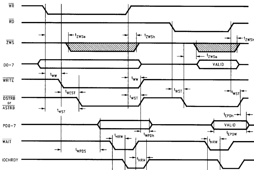
FIGURE 12-21. Enhanced Parallel Port Timing
