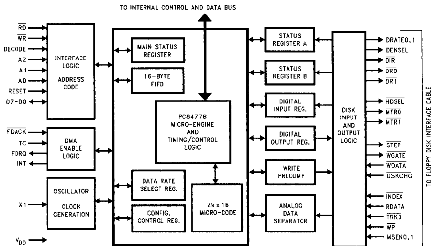
FIGURE 3-1. FDC Functional Block Diagram
