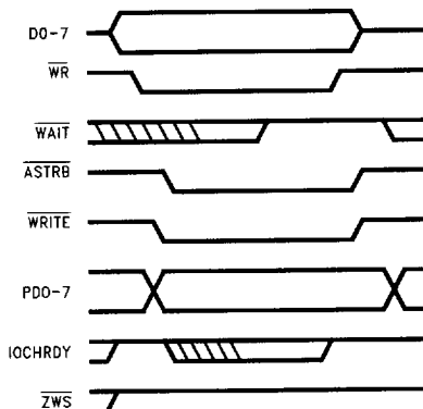
FIGURE 8-1. EPP 1.7 Address Write
