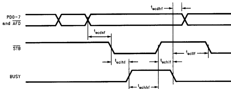
FIGURE 12-22. ECP Parallel Port Forward Timing Diagram
