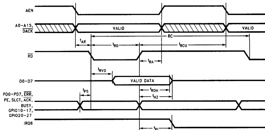
FIGURE 12-2. Microprocessor Read Timing
