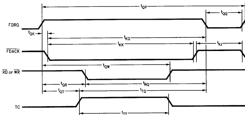
FIGURE 12-11. FDC DMA Timing
