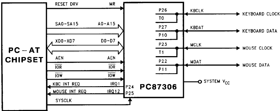
FIGURE 10-2. Keyboard Controller to Host System Interface
