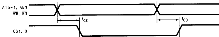
FIGURE 12-27. Chip Select Timing
