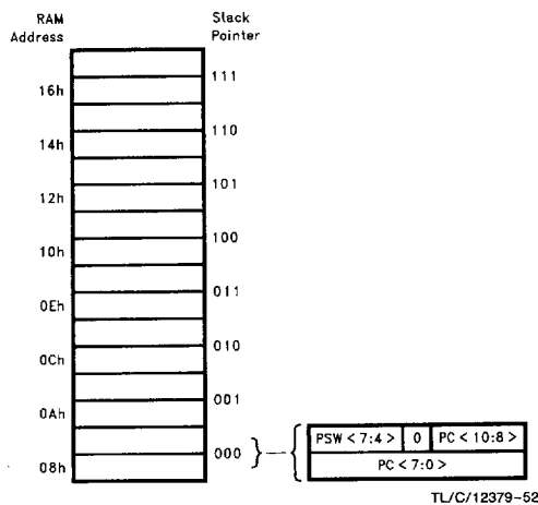
FIGURE 10-6. Keyboard Controller Stack Organization
