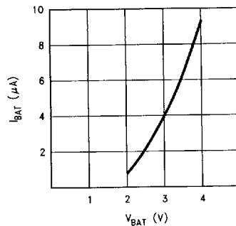
FIGURE 10-16. Typical Battery Current during Battery Backed Mode
