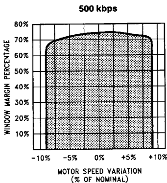
FIGURE 5-2. PC87306 Dynamic Window Margin Performance (Typical performance at V_{DD} = 5.0V , 25^{\circ}C )
