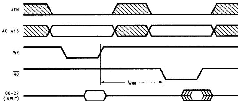
FIGURE 12-4. Read after Write Operation to All Registers and RAM Timing
