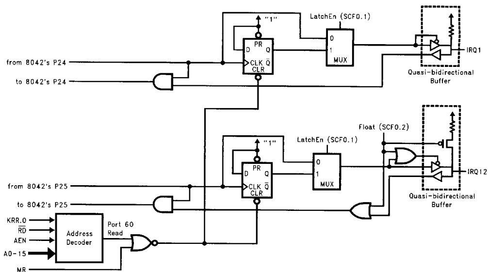
FIGURE 10-4. Fast IRQ Latching and Clearing
