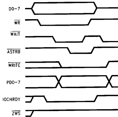
FIGURE 8-4. EPP 1.9 Address Write
