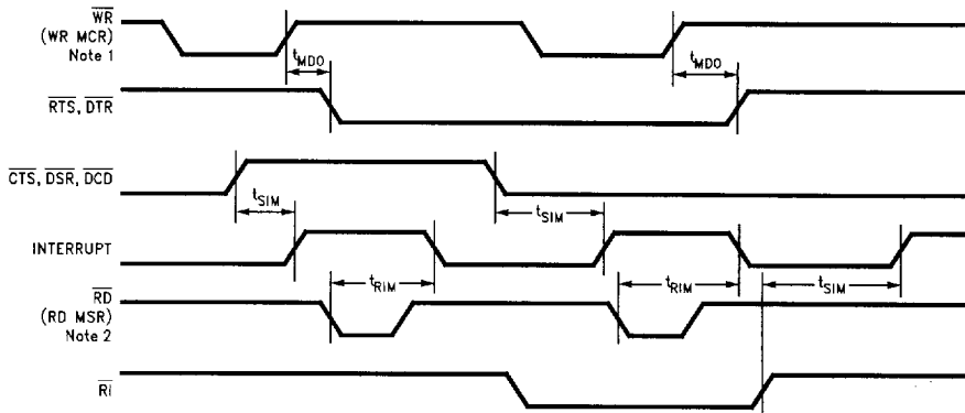
FIGURE 12-10. MODEM Control Timing
