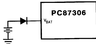
FIGURE 10-15. Typical Battery Configuration
