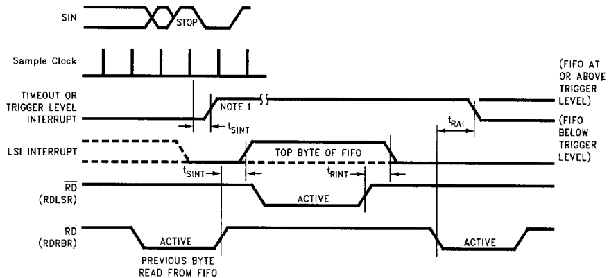
FIGURE 12-9. Timeout Receiver Timing
