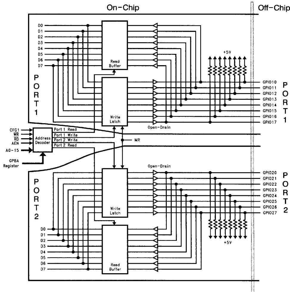
FIGURE 11-1. General Purpose I/O (GPIO) Ports
