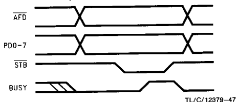
FIGURE 8-6. ECP Forward Write Cycle
