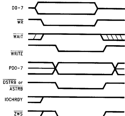
FIGURE 8-3. EPP Write with ZWS
