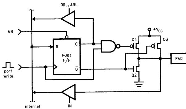
FIGURE 10-8. Active Pull-Up I/O Port Structure
