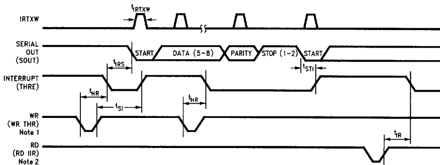
FIGURE 12-6. Transmitter Timing
