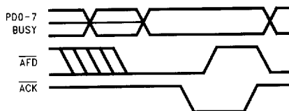
FIGURE 8-7. ECP Backward Read Cycle
