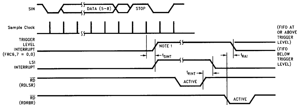
FIGURE 12-7. Receiver Timing
