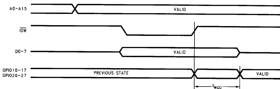
FIGURE 12-24. GPIO Write Timing
