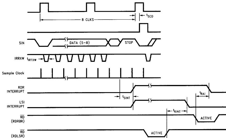
FIGURE 12-7. Receiver Timing
