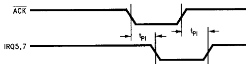
FIGURE 12-18. Compatible Mode Parallel Port Interrupt Timing
