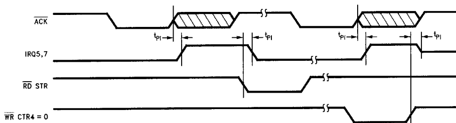
FIGURE 12-19. Extended Mode Parallel Port Interrupt Timing
