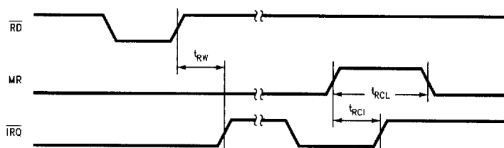
FIGURE 12-25. \overline{IRQ} Release Delay
