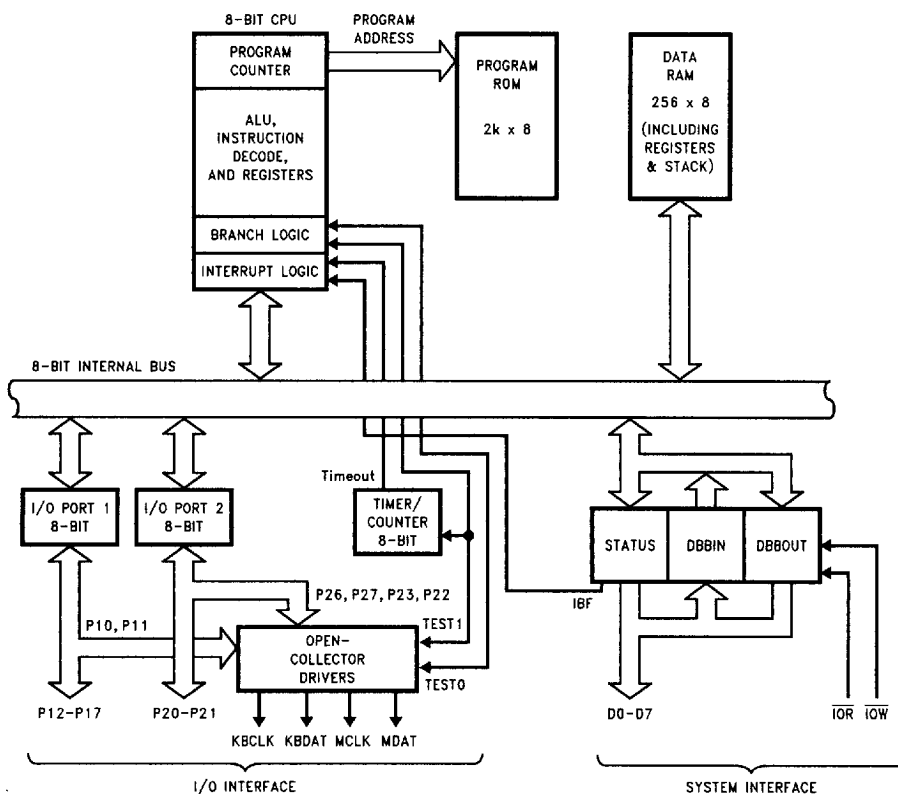
FIGURE 10-1. Keyboard Controller Functional Block Diagram
