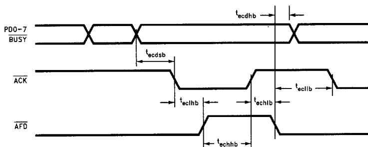
FIGURE 12-23. ECP Parallel Port Backward Timing Diagram
