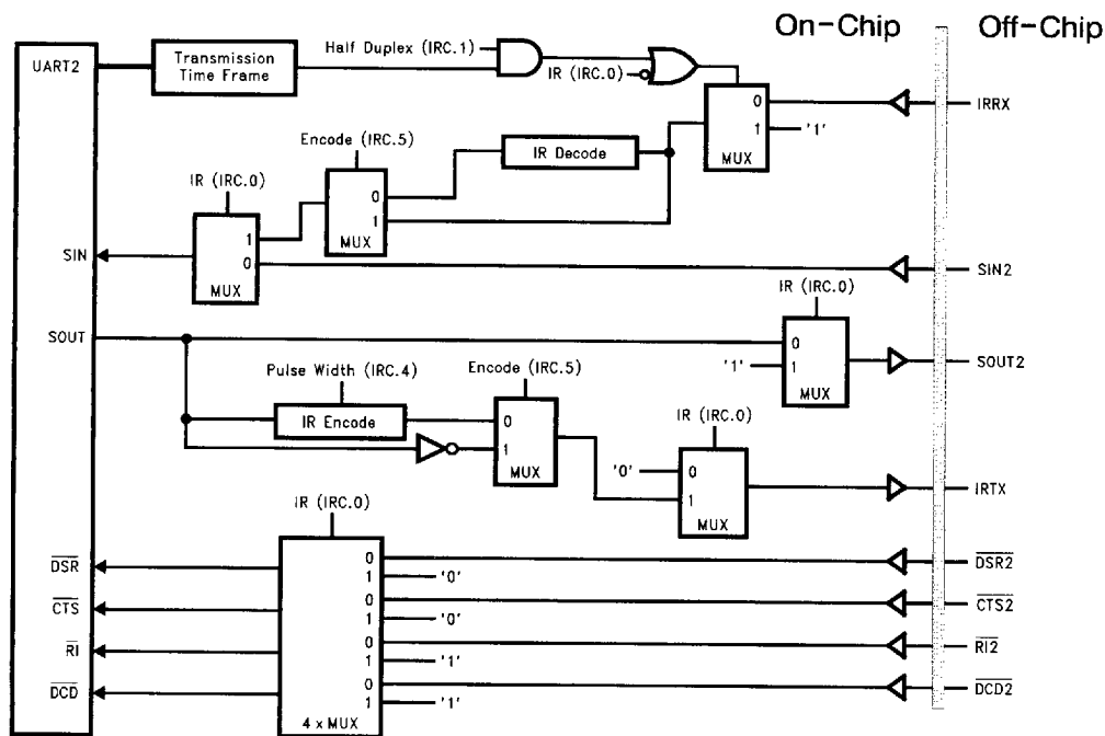
FIGURE 7-1. UART2 Serial and IR Interface Block Diagram
