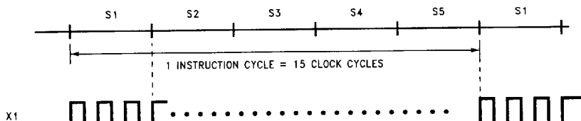
FIGURE 10-12. Instruction Cycle Timing
