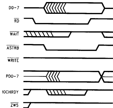
FIGURE 8-2. EPP 1.7 Address Read
