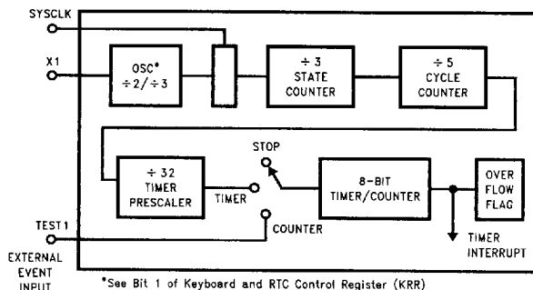
FIGURE 10-10. Timing Generation and Timer Circuit
