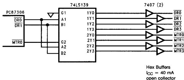
FIGURE 2-2. PC87306 Four Floppy Drive Circuit
