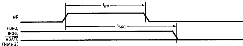
FIGURE 12-13. Reset Timing
