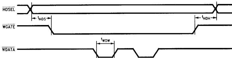
FIGURE 12-14. Write Data Timing
