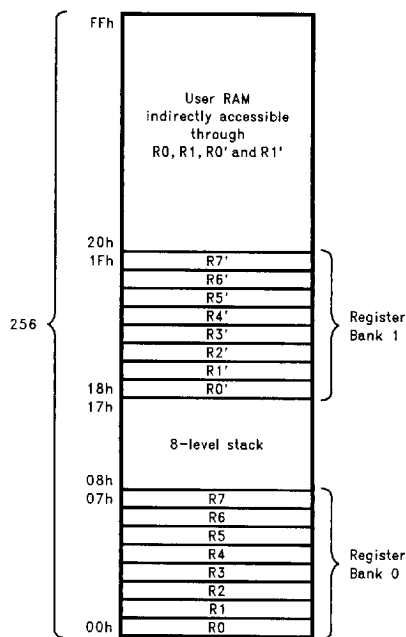
FIGURE 10-5. Keyboard Controller Data Memory Map
