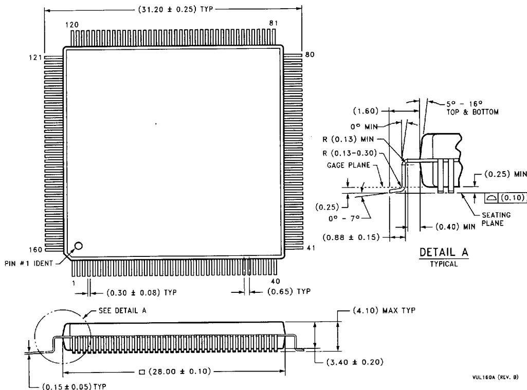
Plastic Quad Flatpak Order Number PC87306VUL NS Package Number VUL160A
