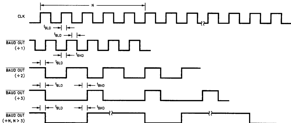
FIGURE 12-5. Baud Out Timing
