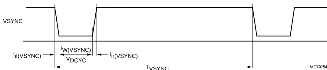
Fig.37 Vertical sync input signal.
