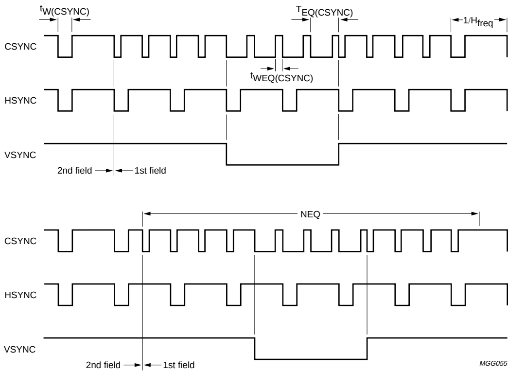
Fig.38 Standard composite sync pulse wave forms.
