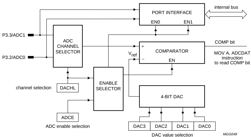
Fig.20 Block diagram of the ADC.
