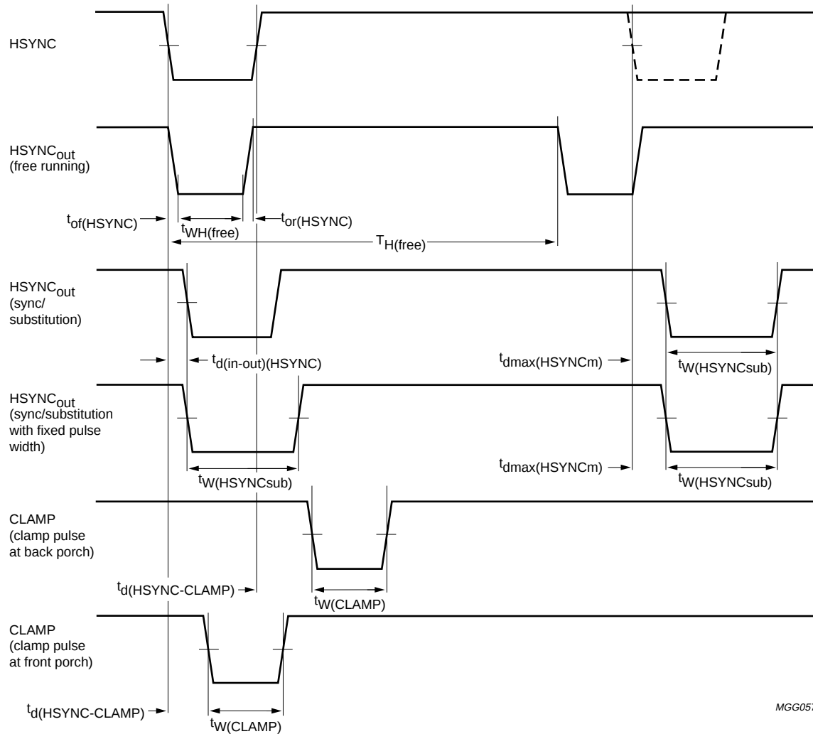
Fig.40 Horizontal sync output pulse.
