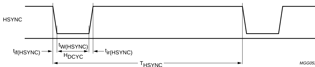
Fig.36 Horizontal sync input signal.
