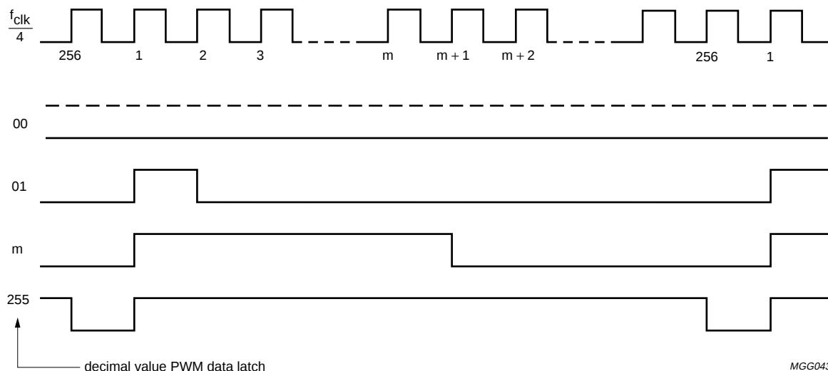
Fig.14 PWM0 to PWM9 output patterns.
