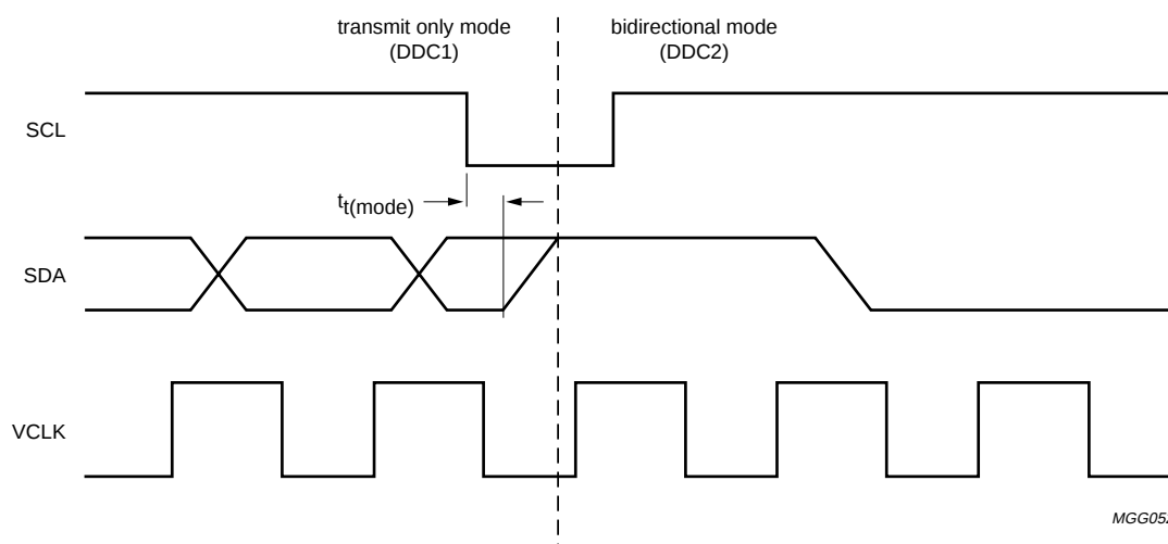
Fig.35 Mode transition from DDC1 to DDC2.
