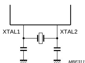
a. Crystal oscillator; C = 20 pF.
