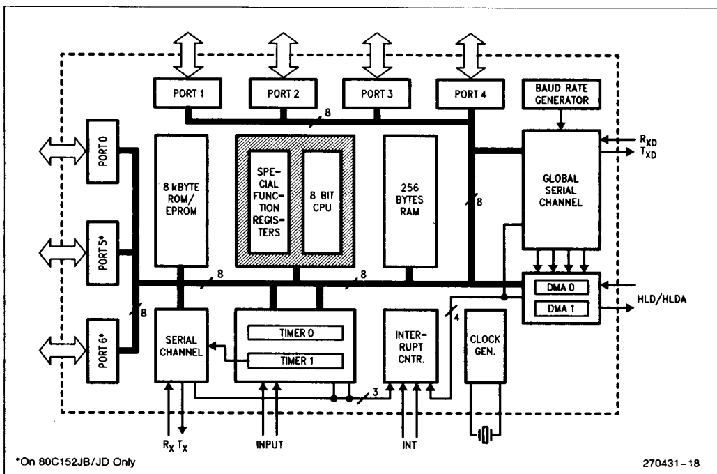
Figure 2. Block Diagram
