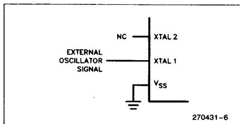
Figure 4. External Clock Drive
