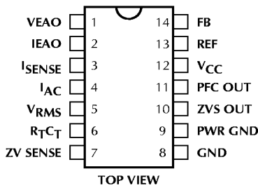
ML4822 14-Pin DIP (P14)
