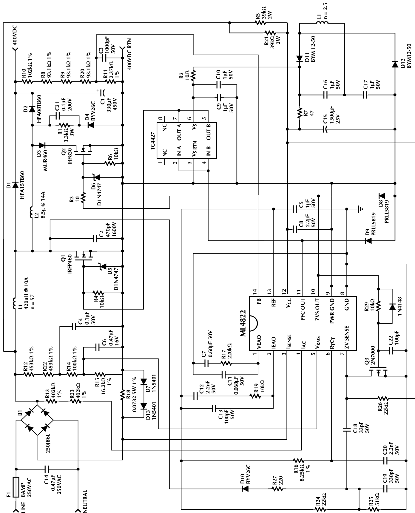
Figure 3. ML4822 Schematic
