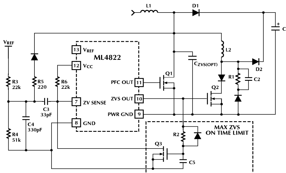
Figure 1. Simplified PFC/ZVS Schematic.
