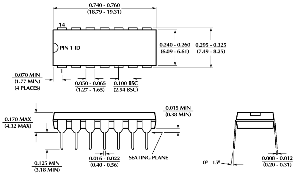
Package: P14 14-Pin PDIP
