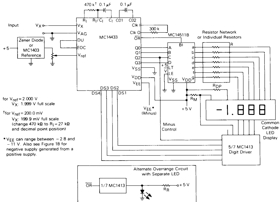
FIGURE 12 — 3½ DIGIT VOLTMEETER WITH LOW COMPONENT COUNT
