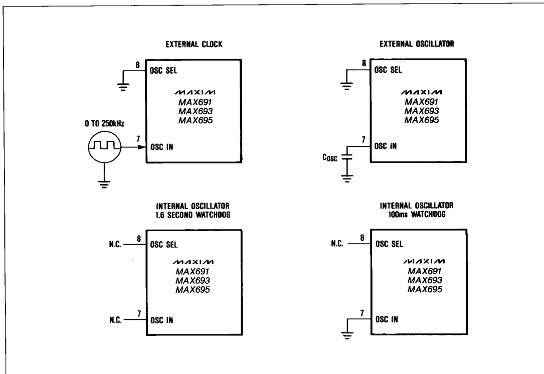
Figure 8. Oscillator Circuits
