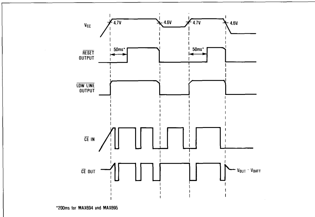
Figure 6. Reset Timing
