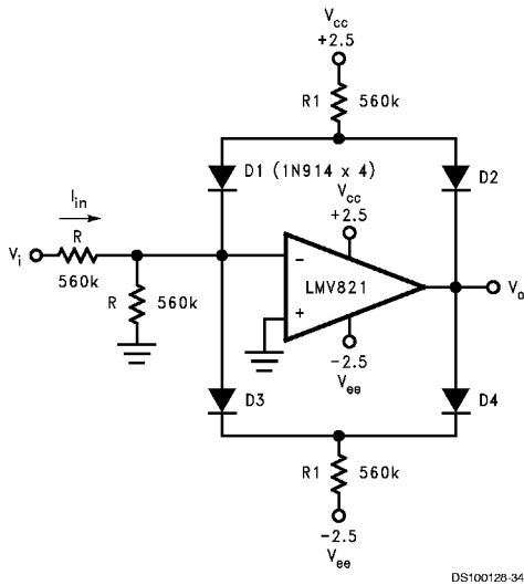
FIGURE 13. Tri-level Voltage Detector
