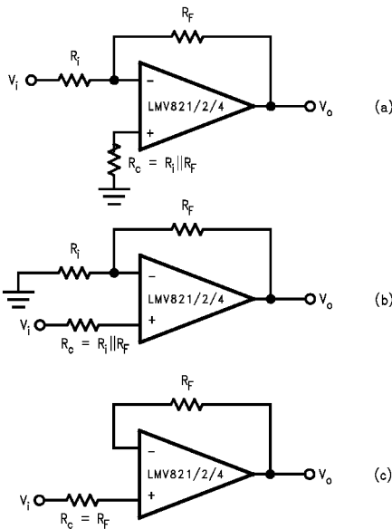
FIGURE 6. Cancelling the Voltage Offset Effect of Input Bias Current
