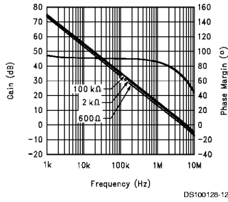
Gain and Phase Margin vs Frequency ( R_L=100k\Omega, 2k\Omega, 600\Omega ) 5V
