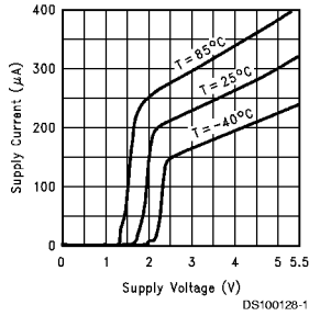
Supply Current vs Supply Voltage (LMV821)
