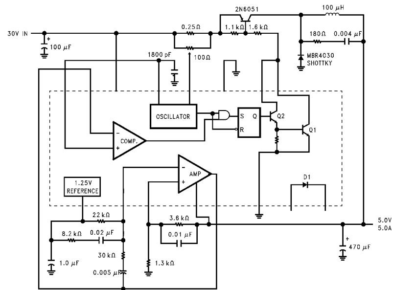
FIGURE 4. Pulse Width Modulated Step-Down Regulator ( f_{OSC} = 20 kHz)
