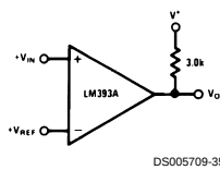
Basic Comparator
