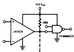
Driving CMOS
