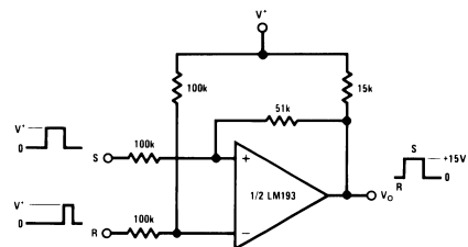
Bi-Stable Multivibrator
