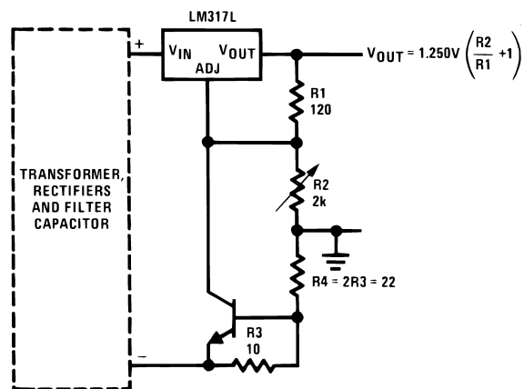
Adjustable Regulator with Current Limiter
