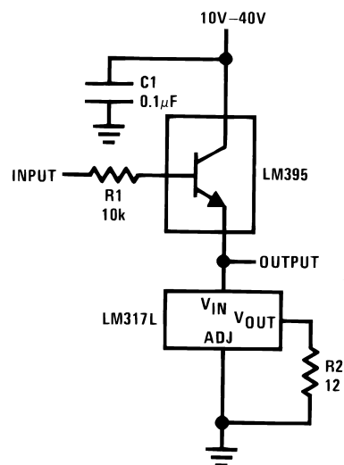
Power Follower
