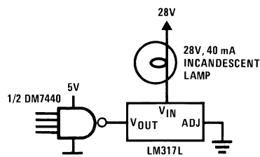
Fully Protected (Bulletproof) Lamp Driver
