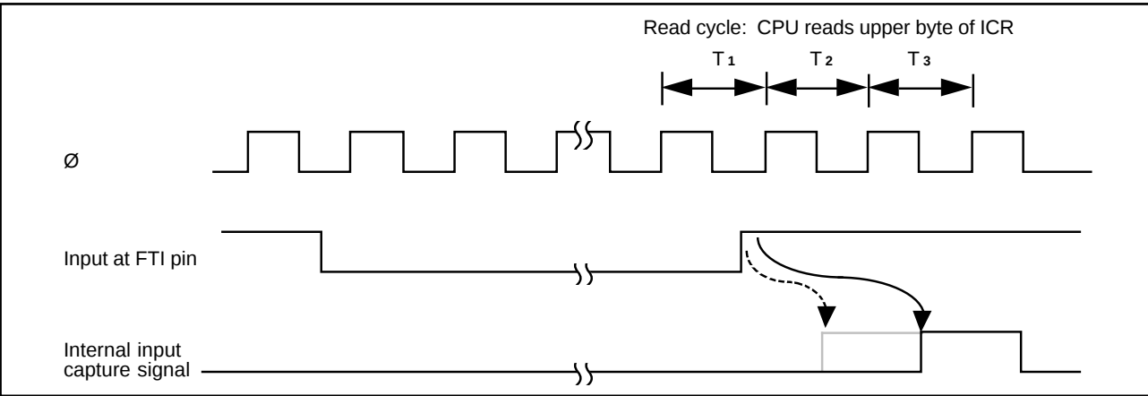
Figure 6-13. Input Capture Timing (1-State Delay)
