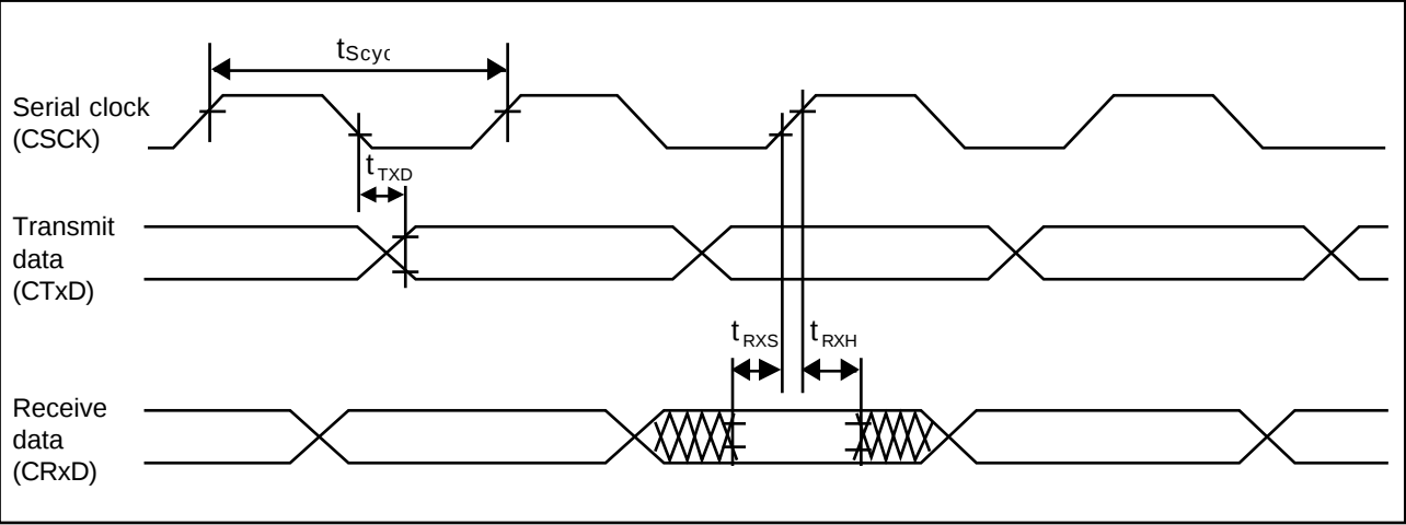
Figure 17-17. SCI Input/Output Timing (Synchronous Mode)
