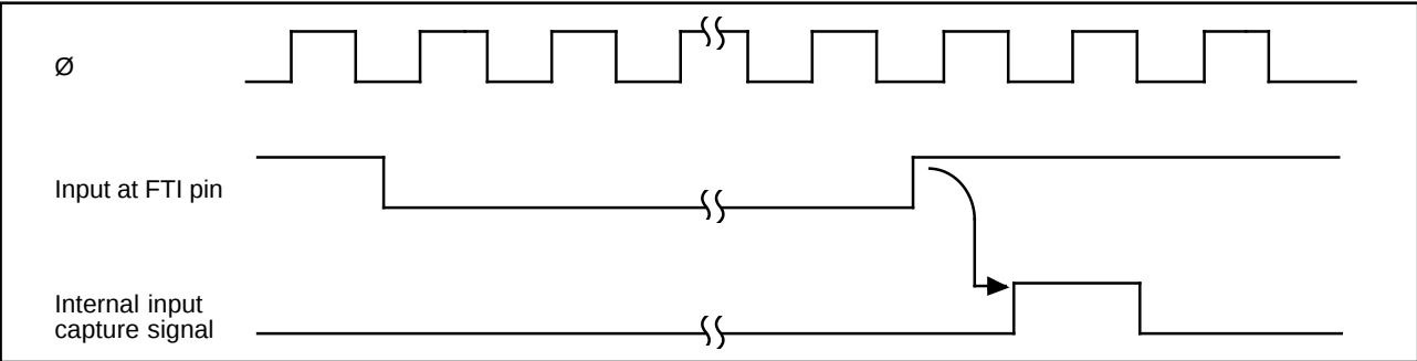
Figure 6-12. Input Capture Timing (Usual Case)
