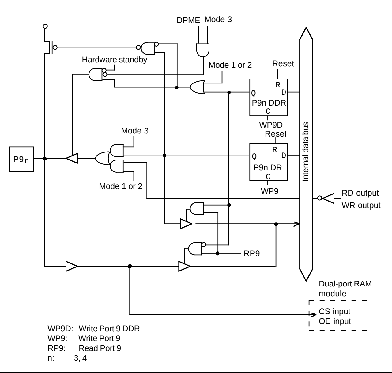
Figure 5-22. Port 9 Schematic Diagram (Pins P93 and P94)
