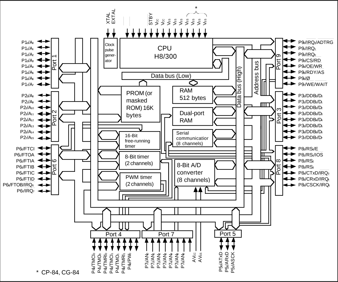
Figure 1-1. Block Diagram
