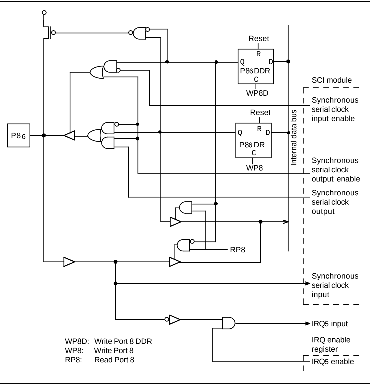
Figure 5-19. Port 8 Schematic Diagram (Pin P86)
