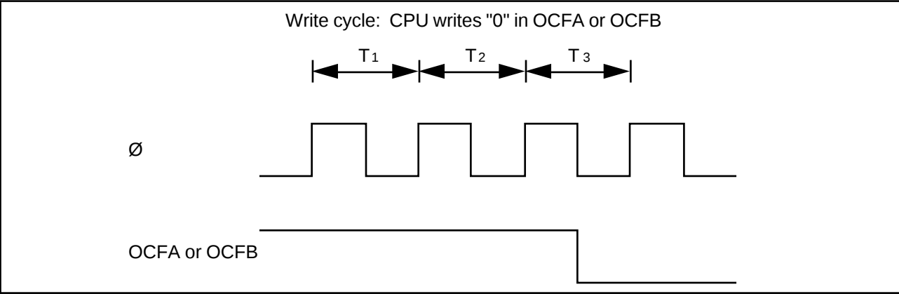
Figure 6-9. Clearing of Output Compare Flag
