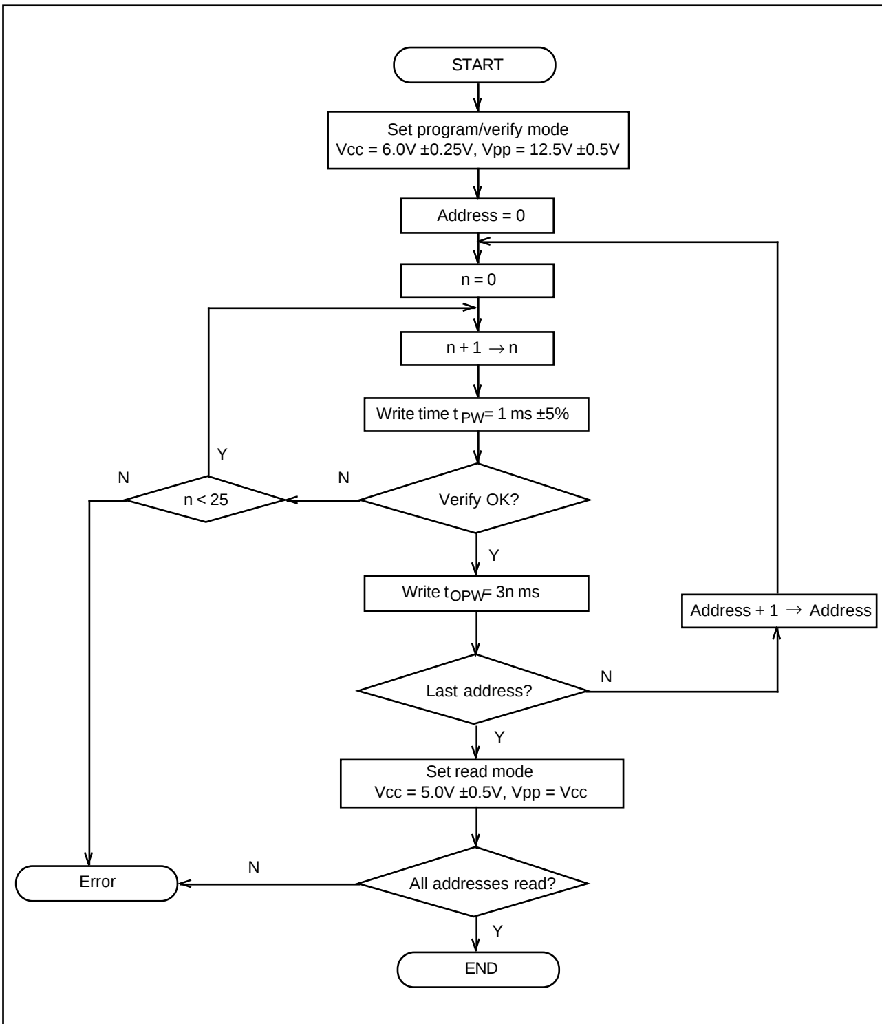
Figure 13-4. High-Speed Programming Flowchart
