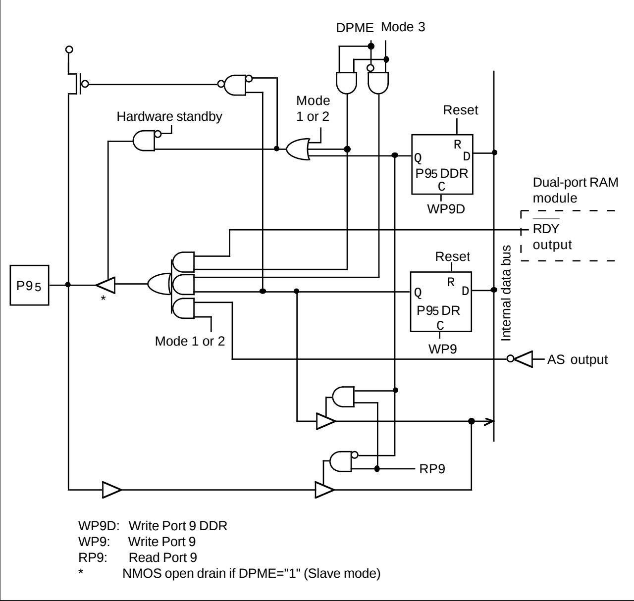
Figure 5-23. Port 9 Schematic Diagram (Pin P95)
