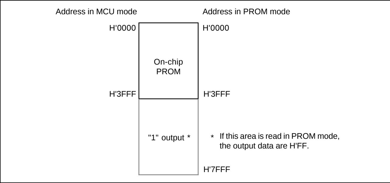
Figure 13-3. Memory Map in PROM Mode
