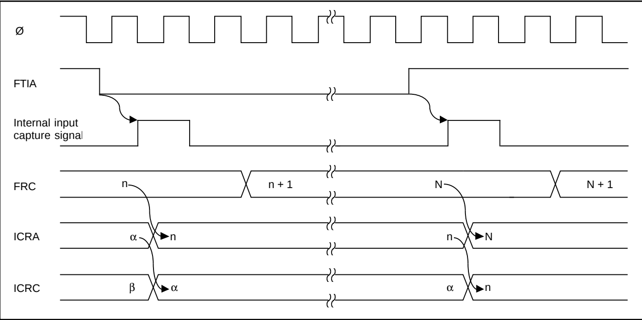
Figure 6-15. Buffered Input Capture with Both Edges Selected
