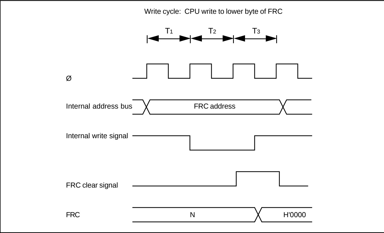
Figure 6-21. FRC Write-Clear Contention
