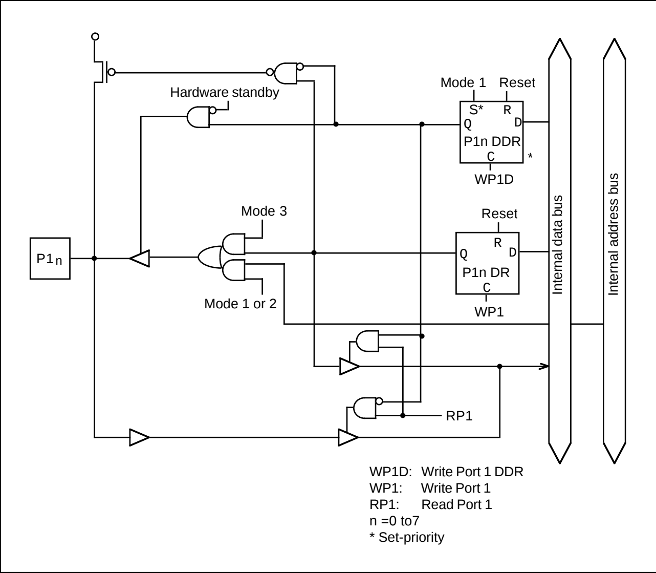
Figure 5-1. Port 1 Schematic Diagram
