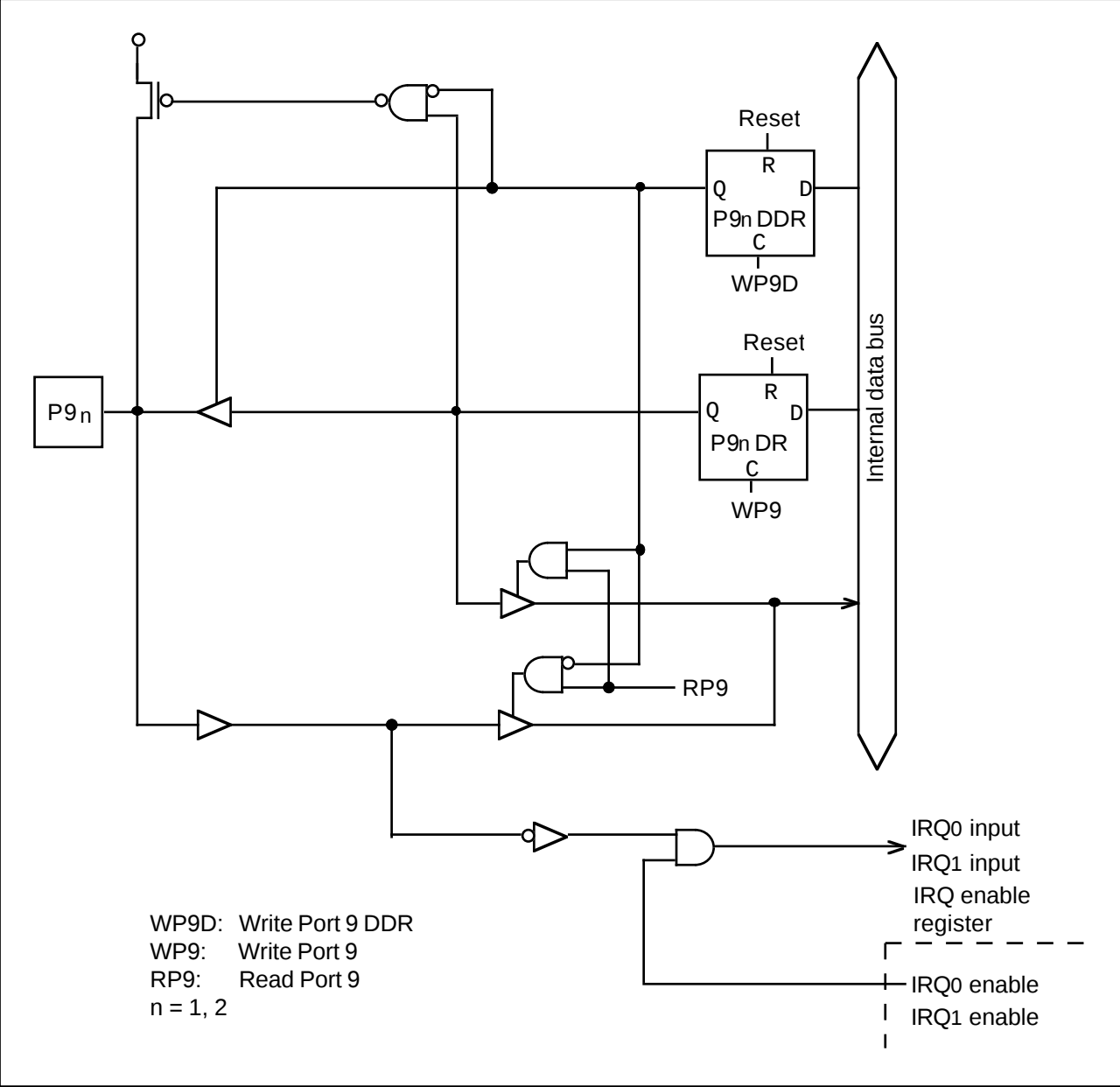
Figure 5-21. Port 9 Schematic Diagram (Pins P91 to P92)
