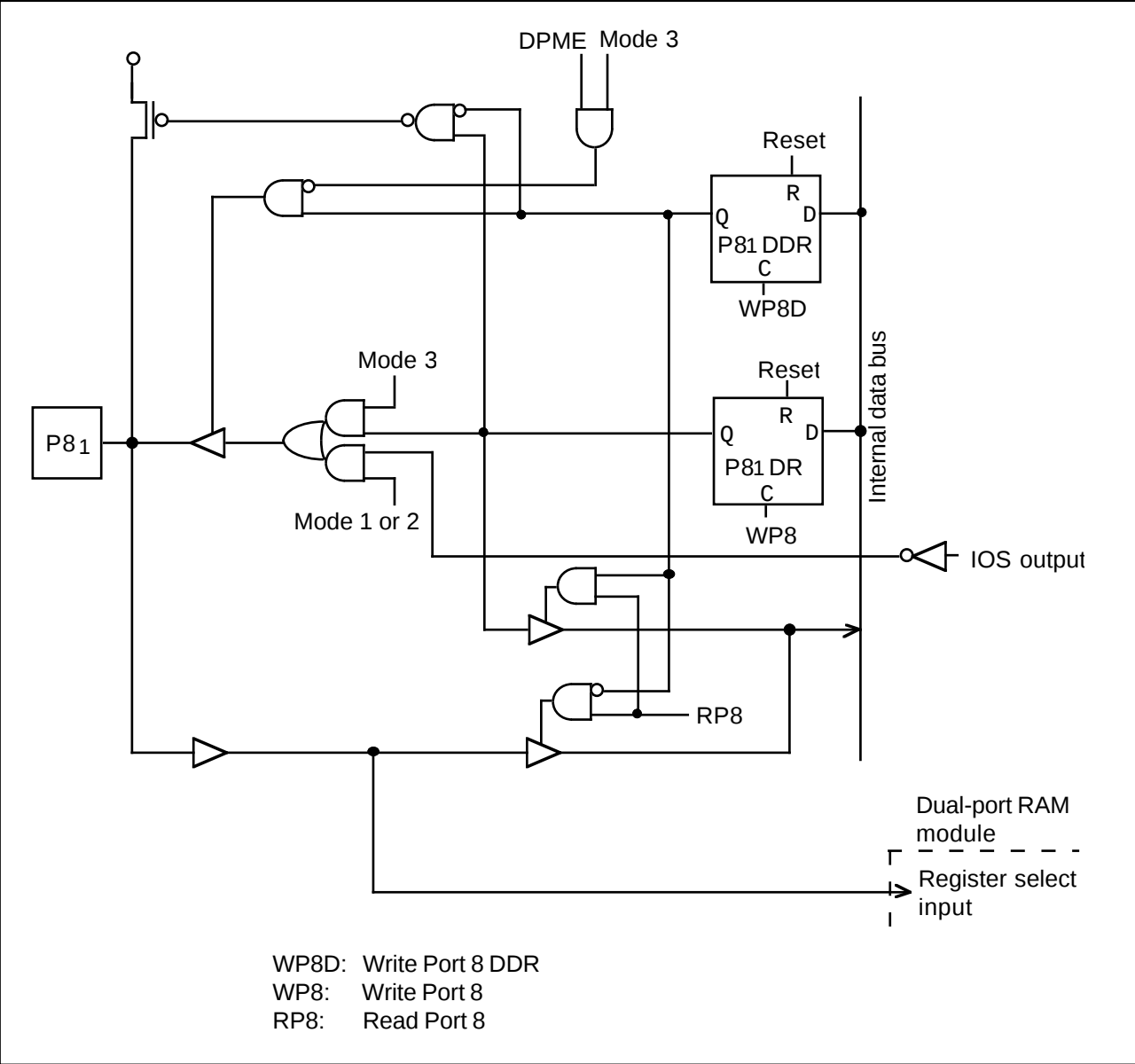
Figure 5-15. Port 8 Schematic Diagram (Pin P81)
