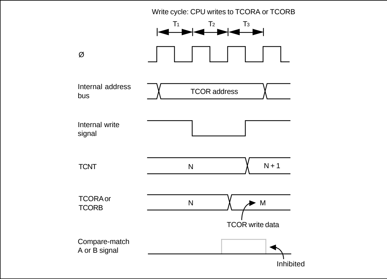
Figure 7-15. Contention between TCOR Write and Compare-Match
