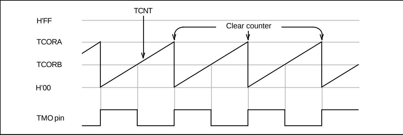
Figure 7-12. Example of Pulse Output
