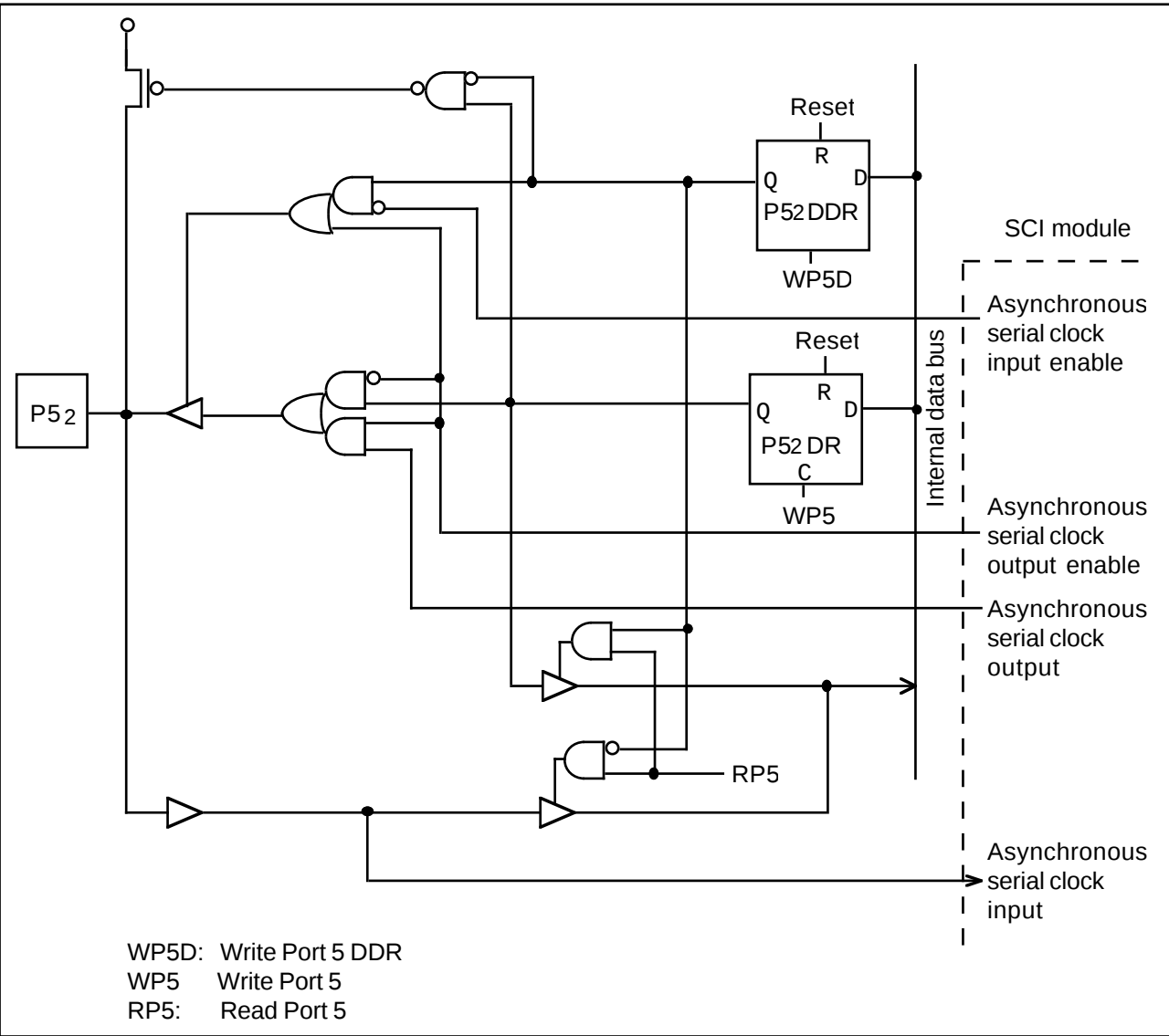
Figure 5-8. Port 5 Schematic Diagram (Pin P52)
