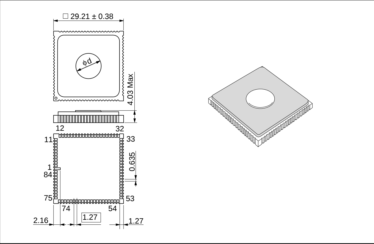
Figure E-1. Package Dimensions (CG-84)
