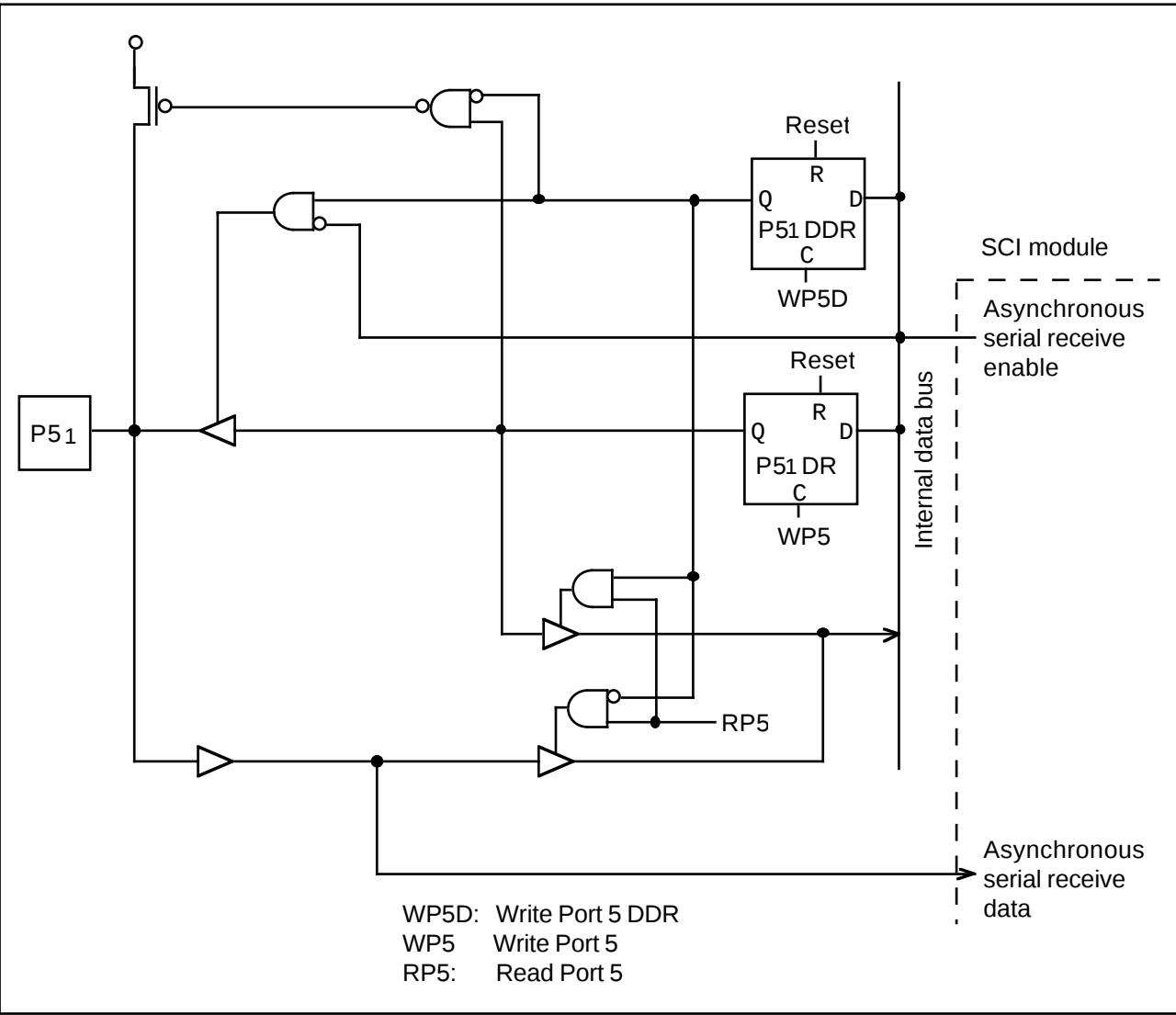
Figure 5-7. Port 5 Schematic Diagram (Pin P51)
