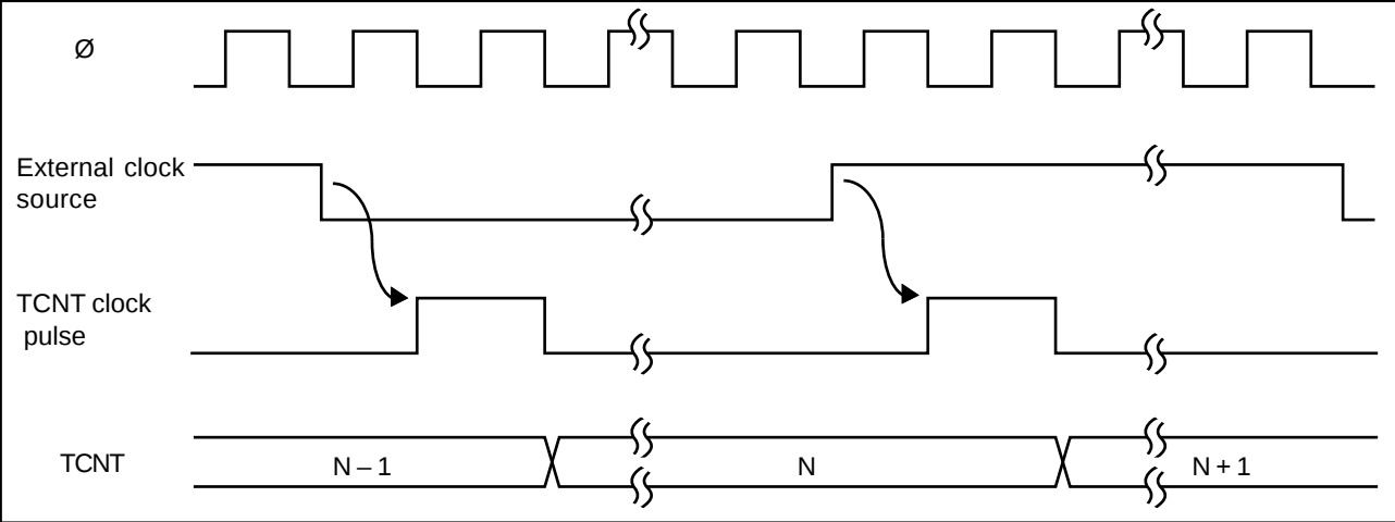
Figure 7-3. Count Timing for External Clock Input
