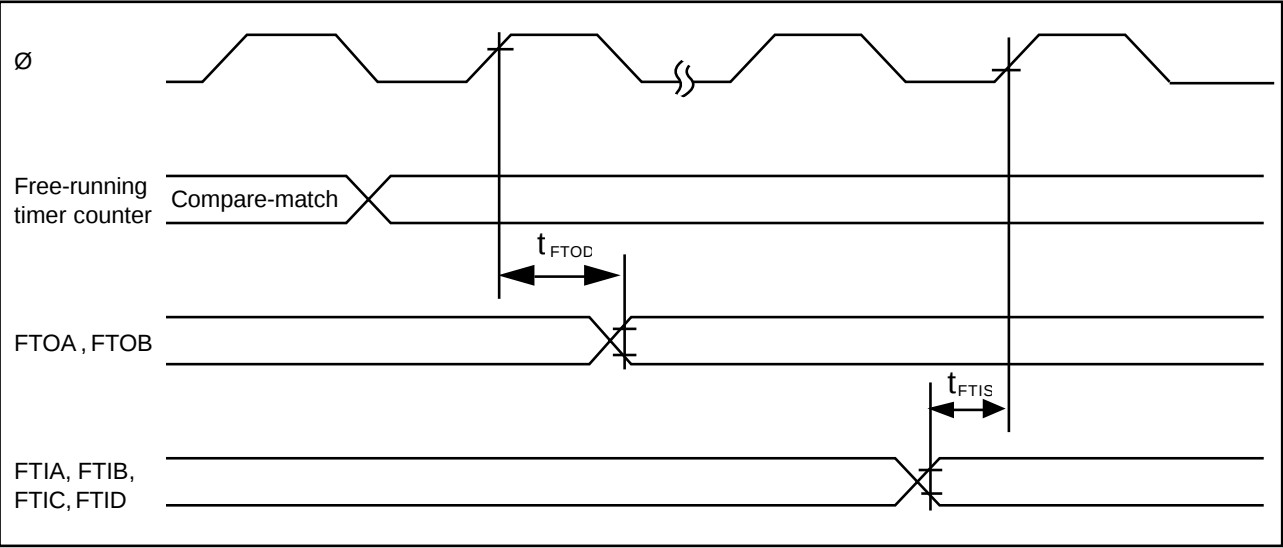
Figure 17-11. Free-Running Timer Input/Output Timing
