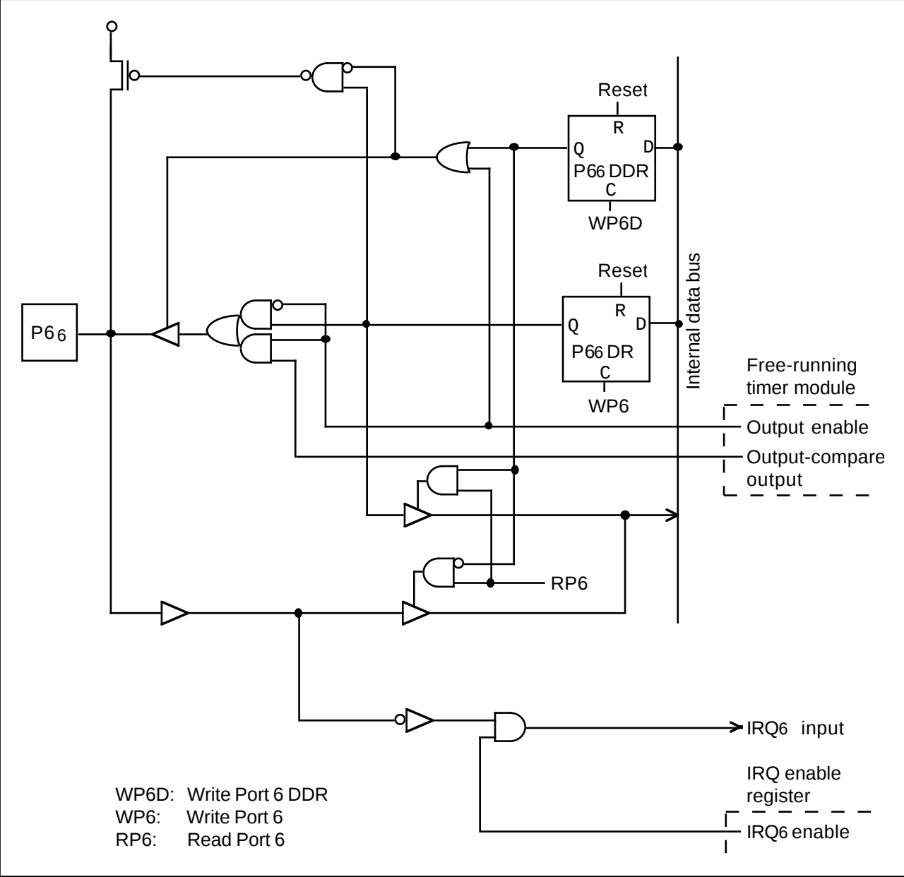
Figure 5-11. Port 6 Schematic Diagram (Pin P66)
