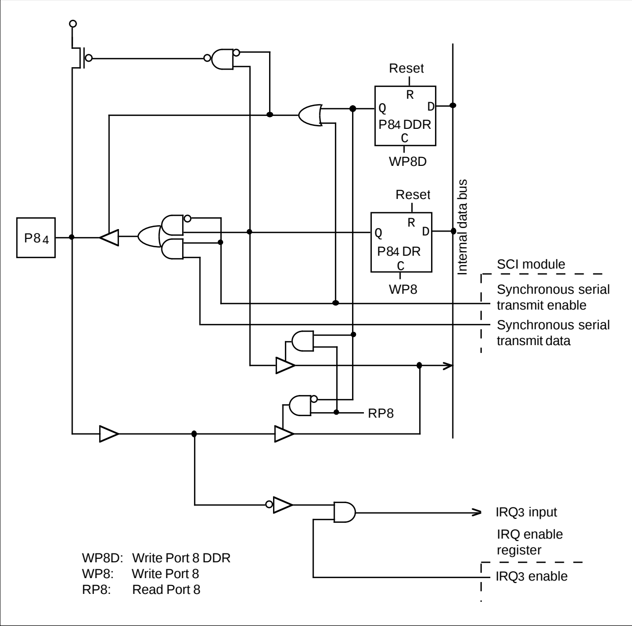
Figure 5-17. Port 8 Schematic Diagram (Pin P84)
