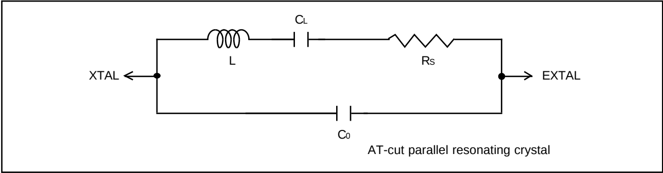
Figure 16-3. Equivalent Circuit of External Crystal
