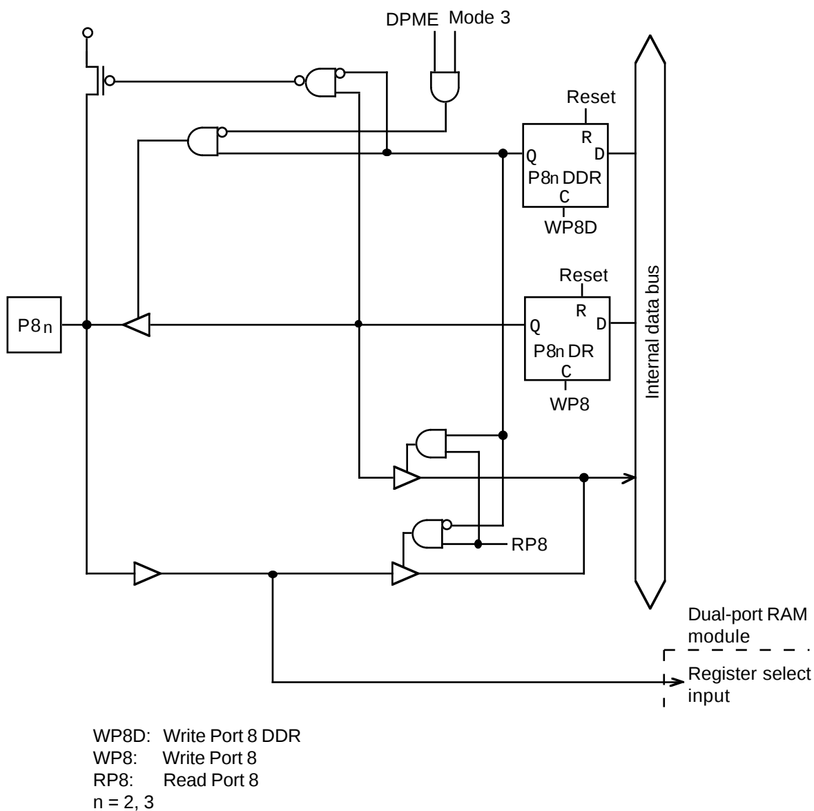
Figure 5-16. Port 8 Schematic Diagram (Pins P82 and P83)
