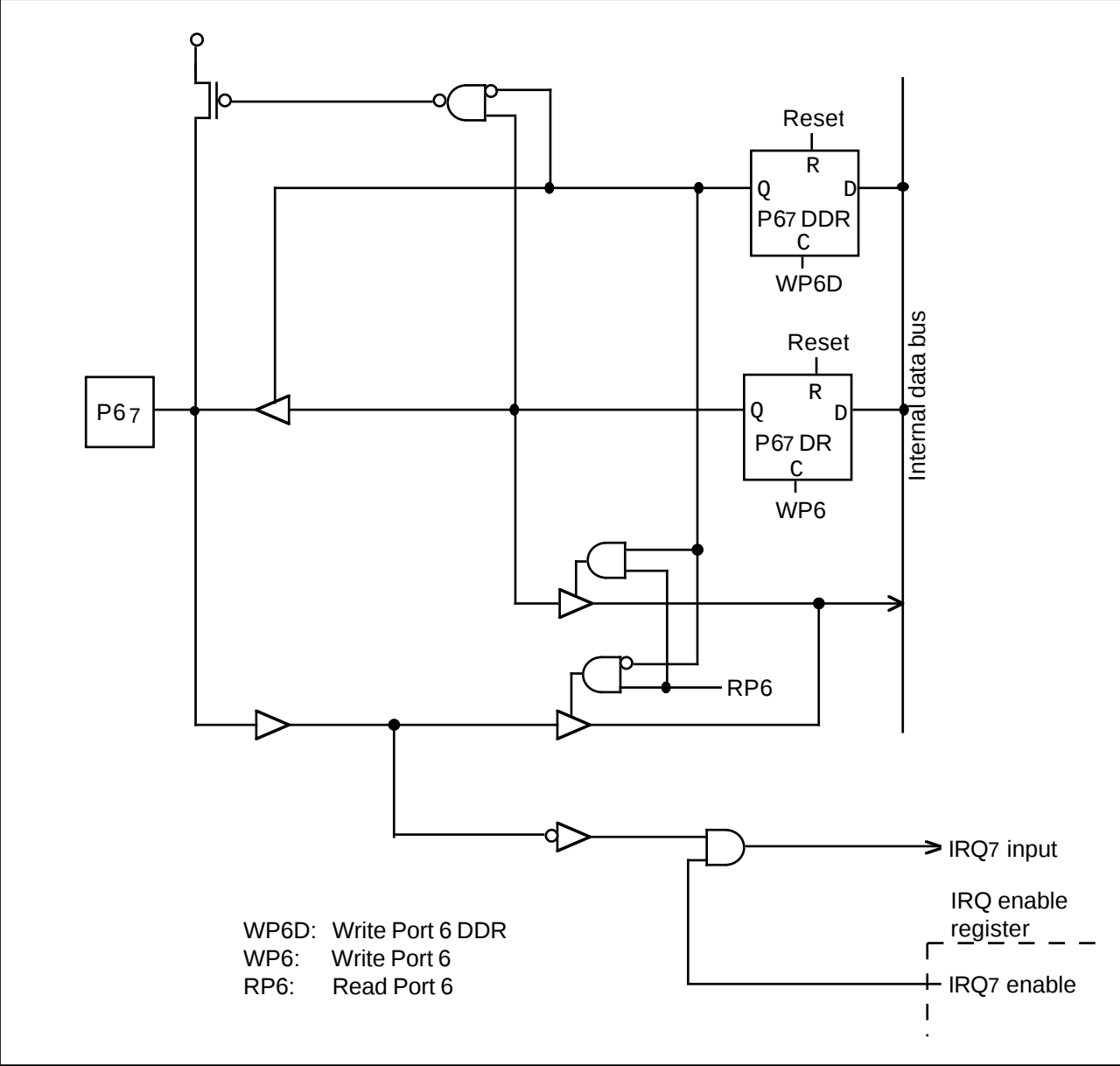
Figure 5-12. Port 6 Schematic Diagram (Pin P67)
