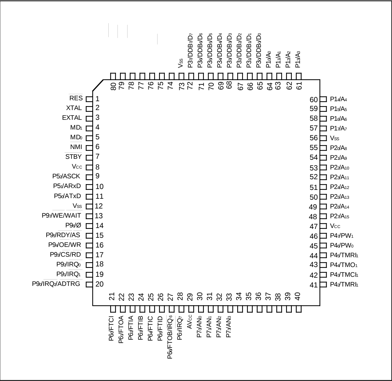
Figure 1-2. Pin Arrangement (FP-80A, Top View)
