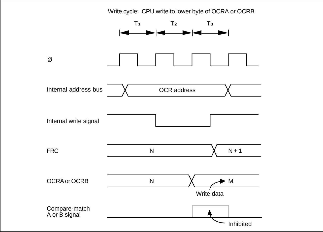
Figure 6-23. Contention between OCR Write and Compare-Match
