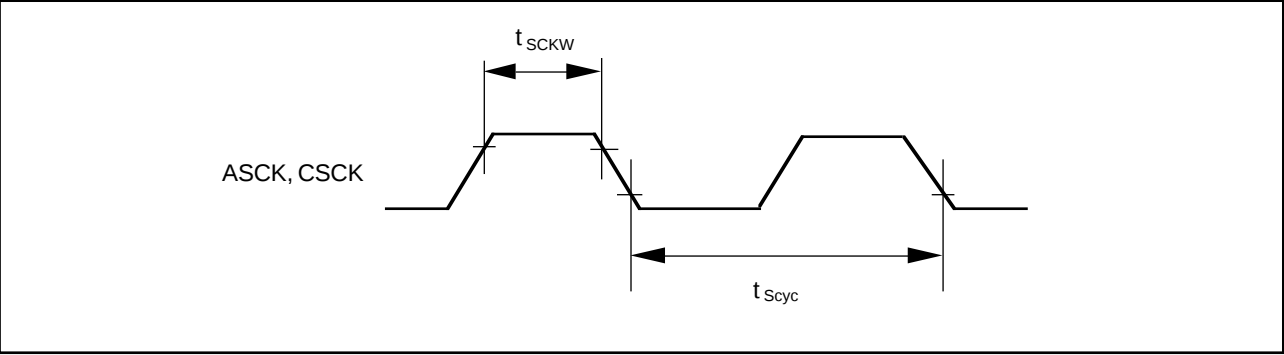
Figure 17-18. SCI Input Clock Timing
