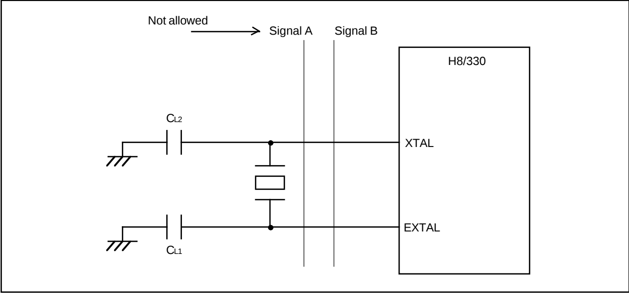
Figure 16-4. Notes on Board Design around External Crystal
