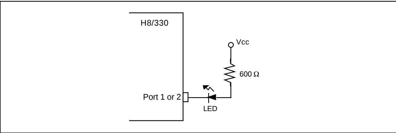
Figure 17-2. Example of Circuit for Driving a LED
