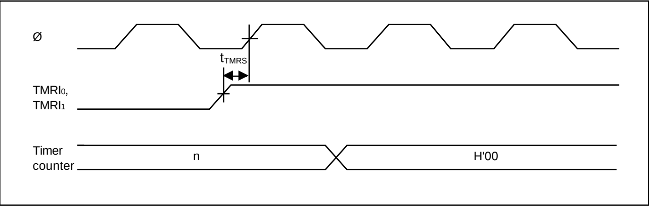
Figure 17-15. 8-Bit Timer Reset Input Timing
