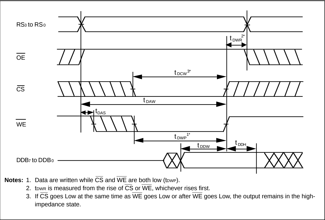
Figure 17-21. Dual-Port RAM Write Timing
