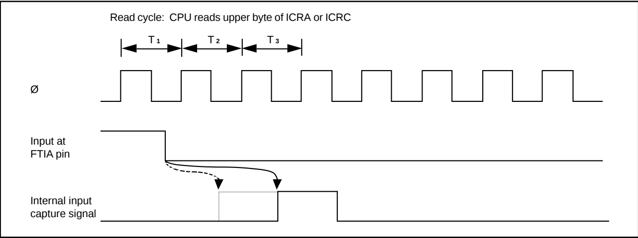
Figure 6-14. Input Capture Timing (1-State Delay, Buffer Mode)
