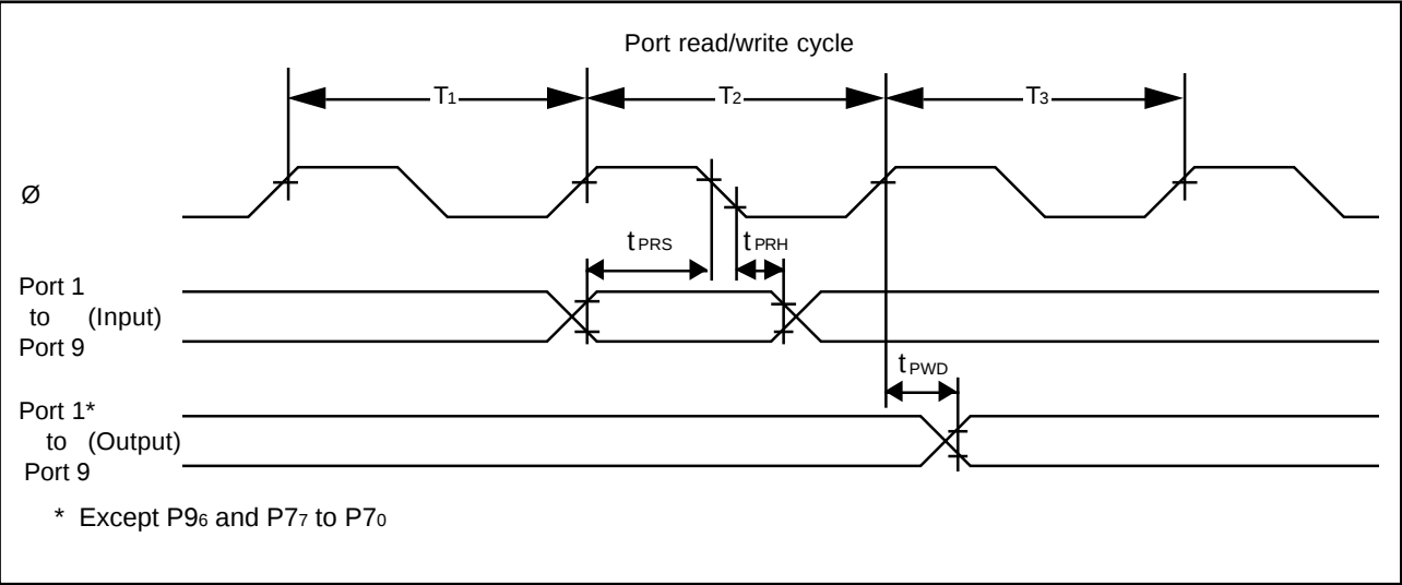
Figure 17-19. I/O Port Input/Output Timing
