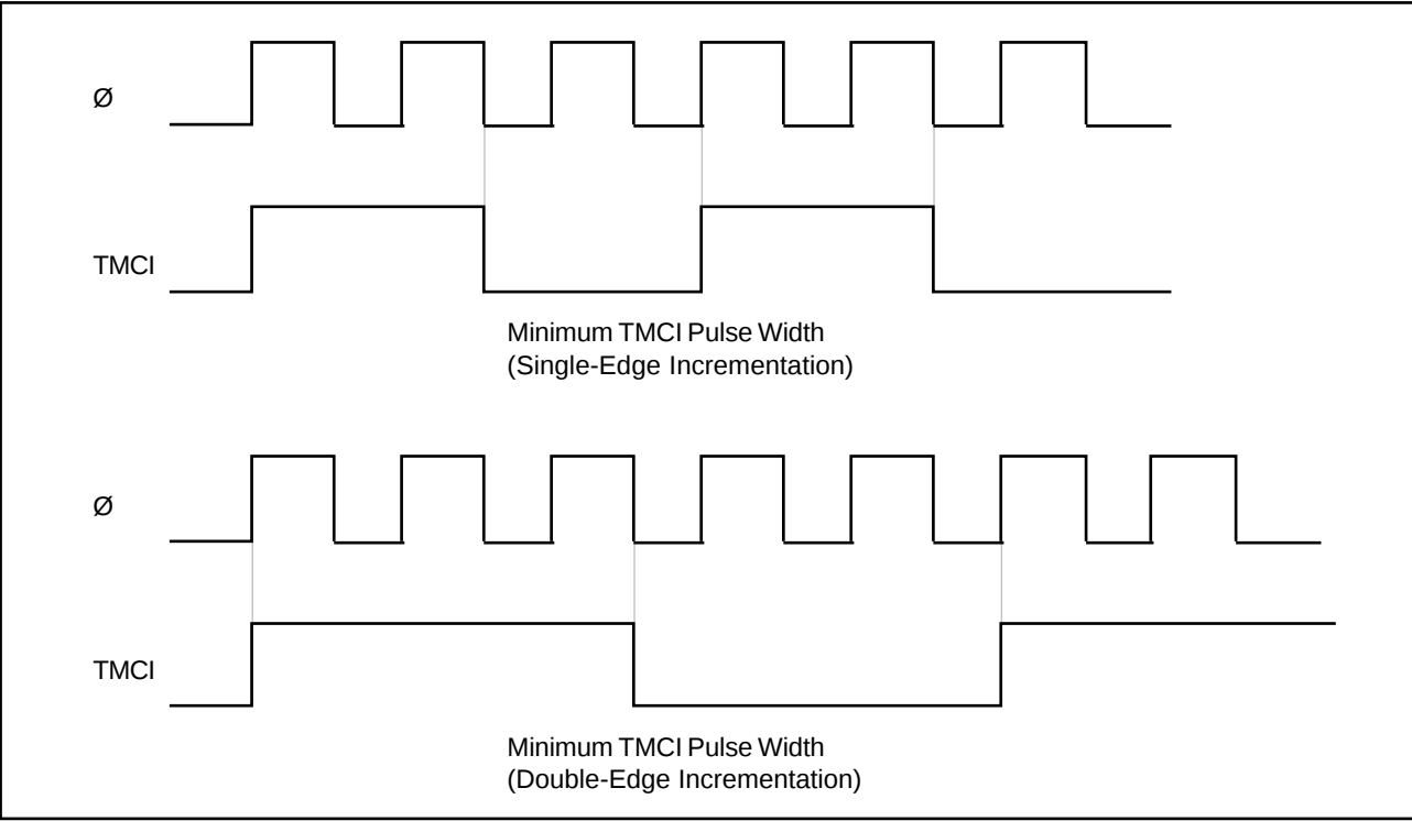
Figure 7-4. Minimum External Clock Pulse Widths (Example)
