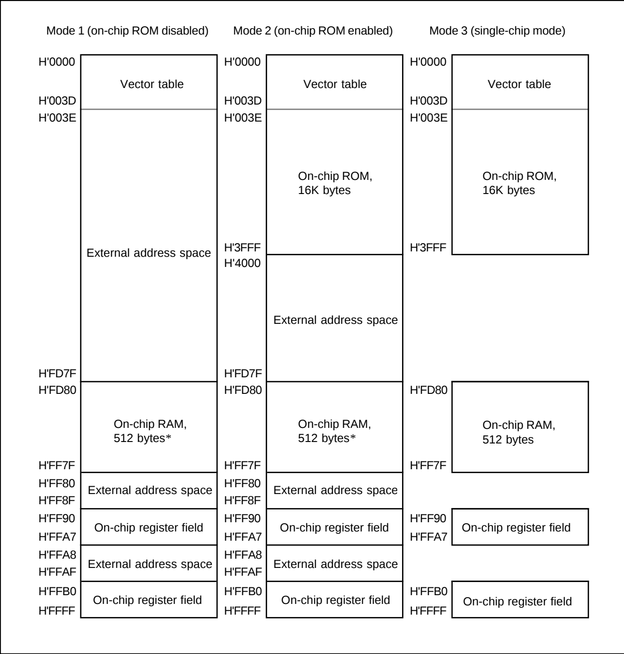
Figure 2-1. Address Space Map
