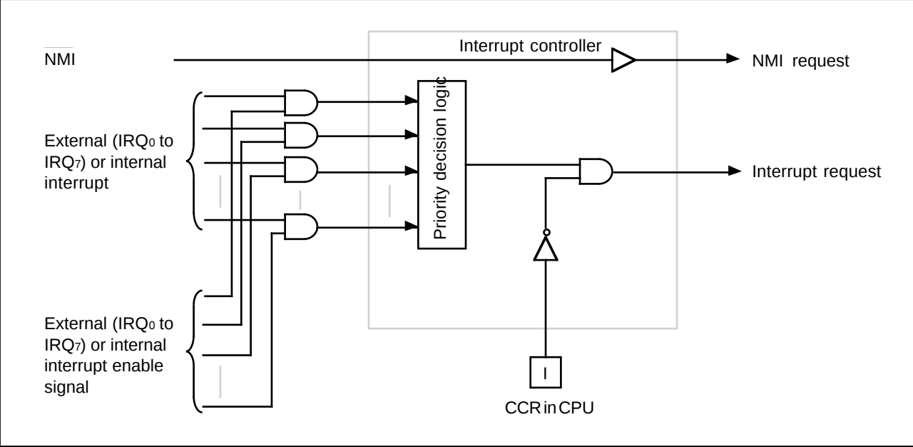
Figure 4-3. Block Diagram of Interrupt Controller
