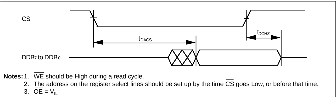
Figure 17-20. Dual-Port RAM Read Timing
