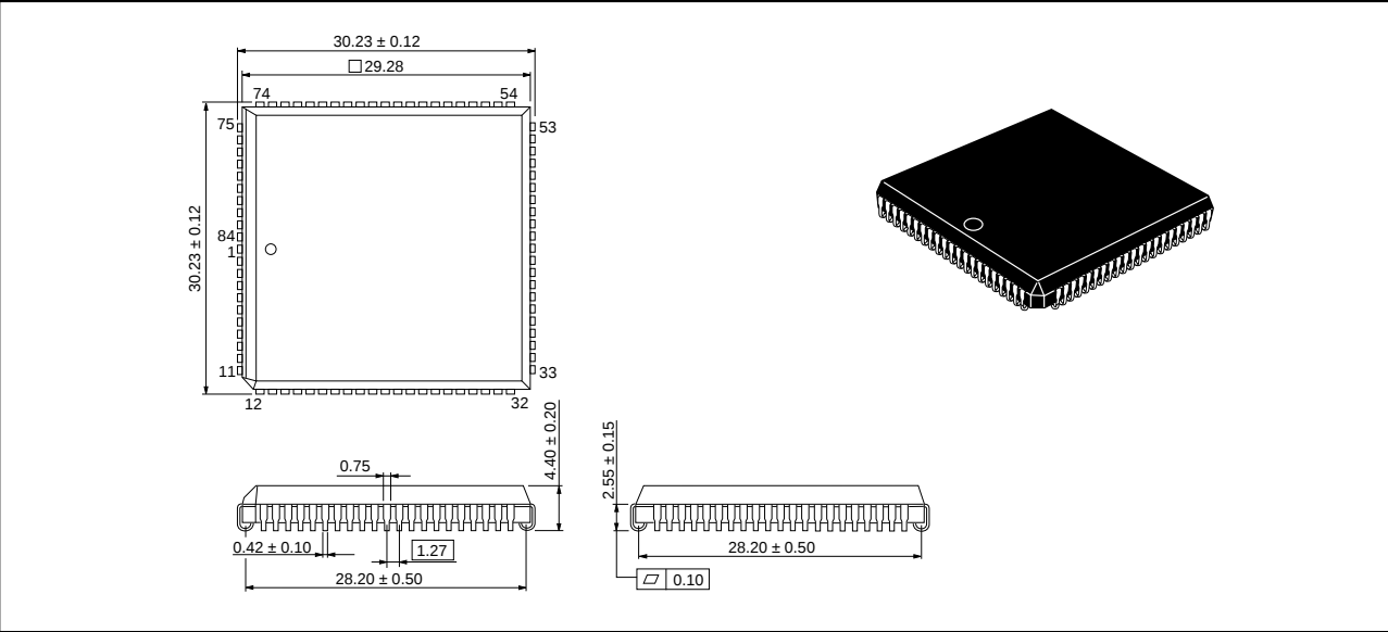
Figure E-1. Package Dimensions (CG-84)
