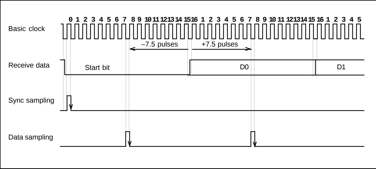
Figure 9-6. Sampling Timing (Asynchronous Mode)
