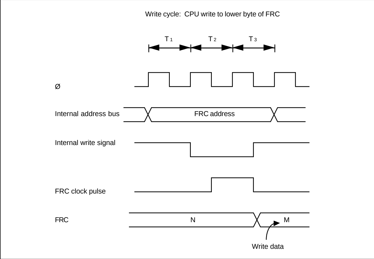
Figure 6-22. FRC Write-Increment Contention
