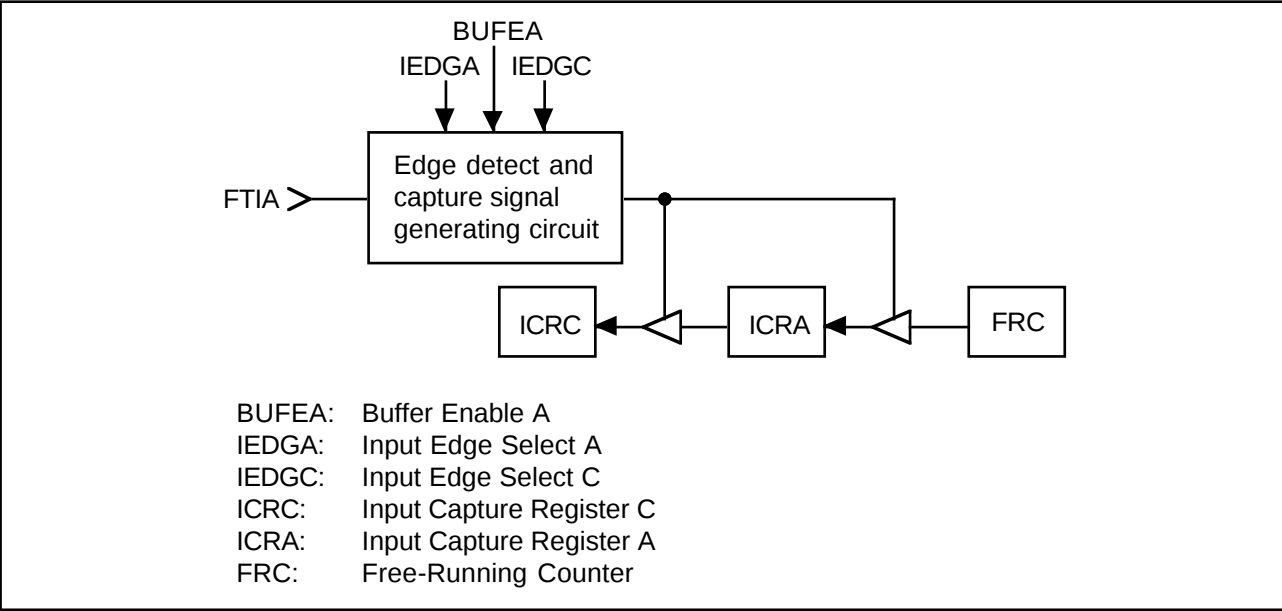
Figure 6-2. Input Capture Buffering
