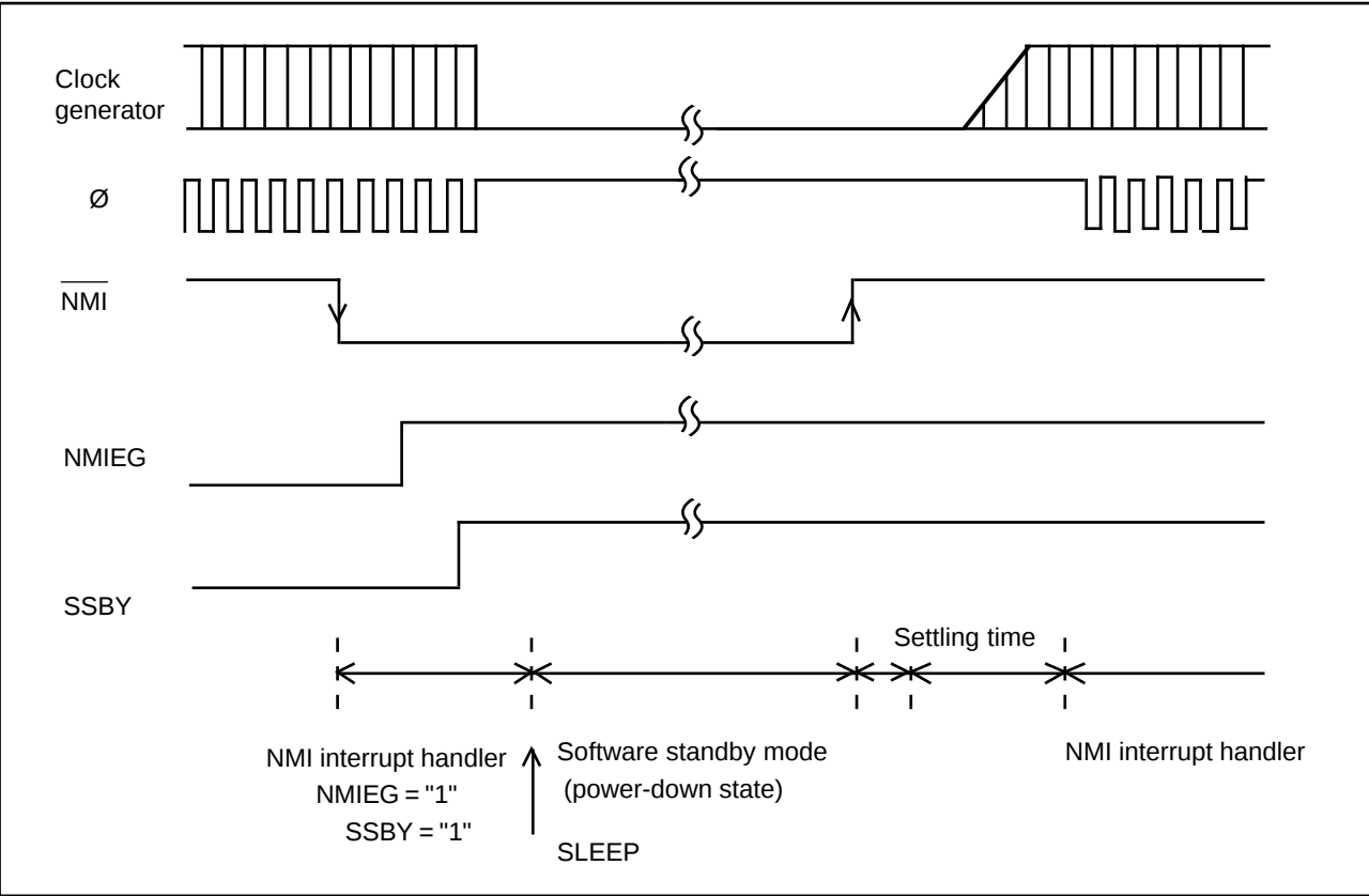
Figure 14-1. Software Standby Mode (when) NMI Timing
