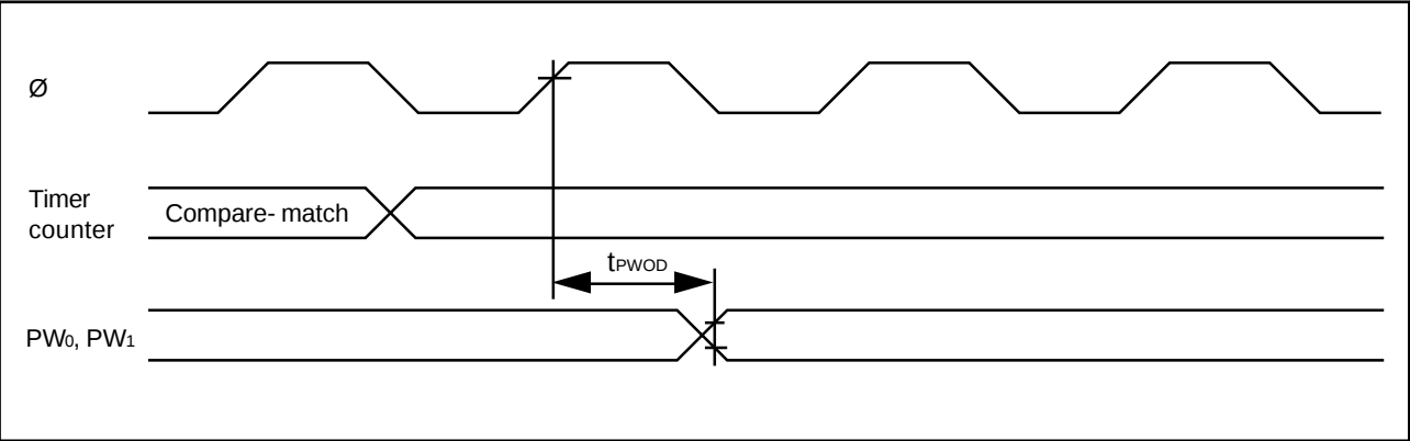
Figure 17-16. PWM Timer Output Timing
