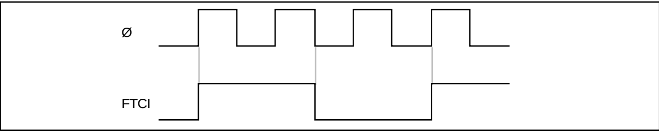
Figure 6-7. Minimum External Clock Pulse Width
