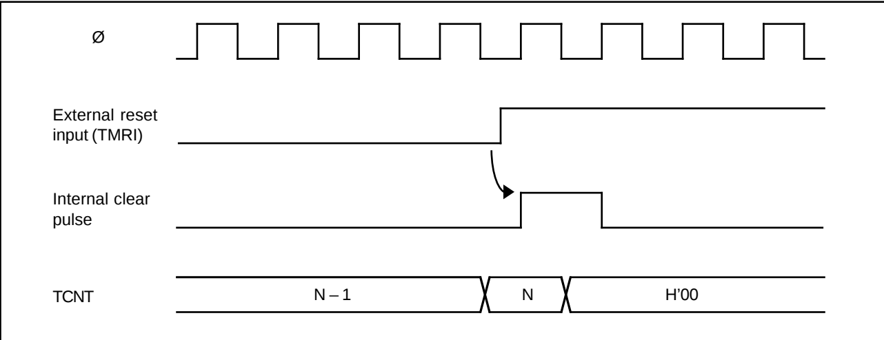
Figure 7-9. Timing of External Reset
