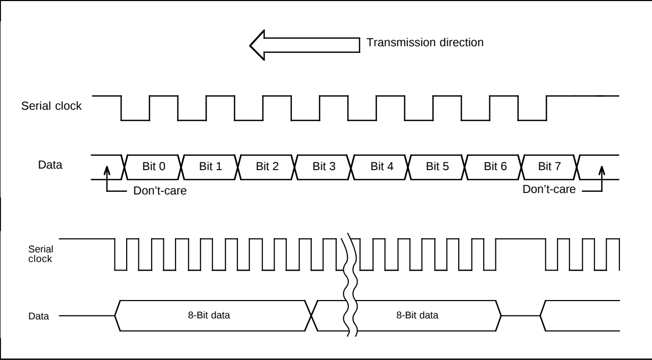
Figure 9-4. Data Format in Synchronous Mode
