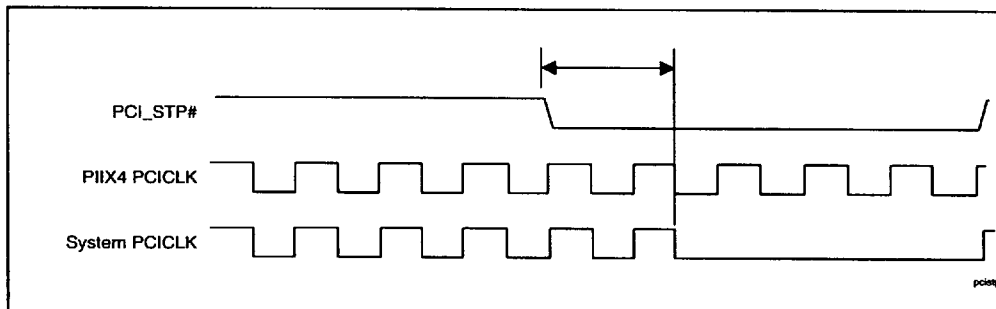
Figure 18. PCI Clock Stop Timing
