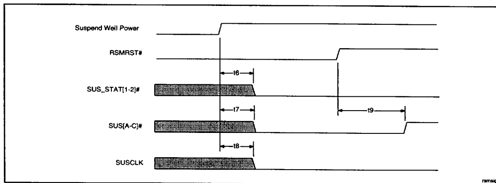
Figure 17. Suspend Well Power and RSMRST# Activated Signals
