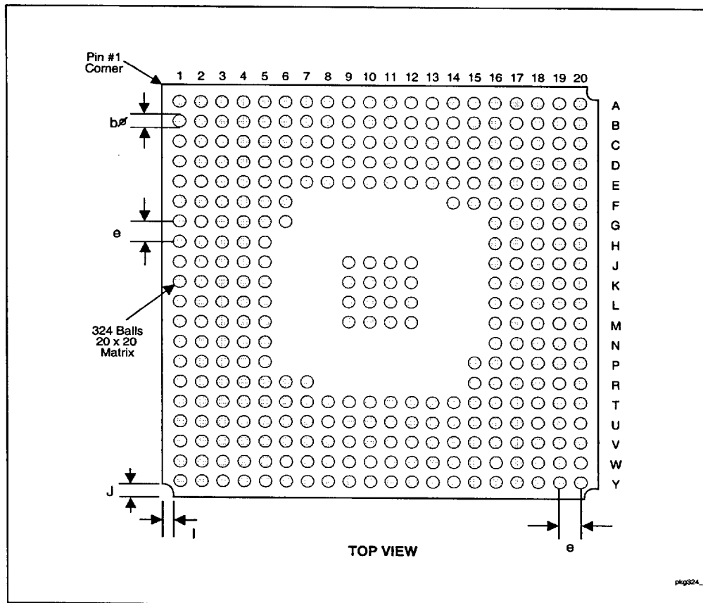
Figure 36. PIIX4 324-Pin Ball Grid Array (BGA) Ball Pattern
