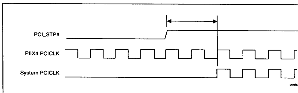
Figure 19. PCI Clock Start Timing
