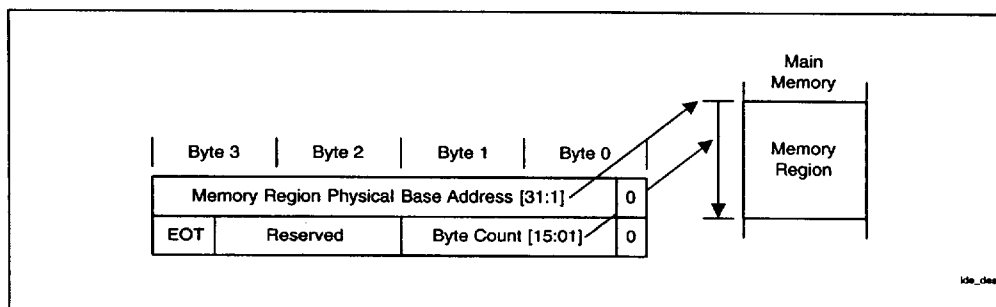
Figure 8. Physical Region Descriptor Table Entry
