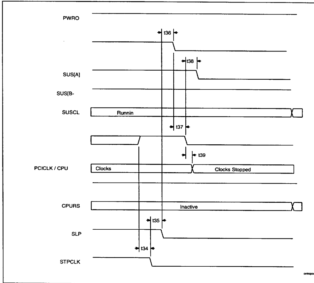
Figure 23. On to POS
