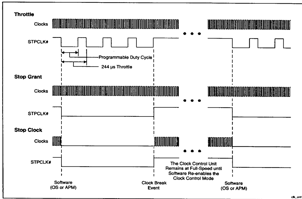
Figure 11. Clock Control Mechanisms (NON-Burst)
