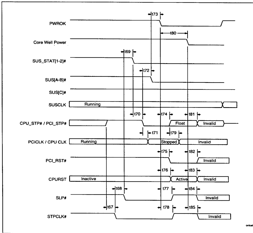
Figure 27. On to STR
