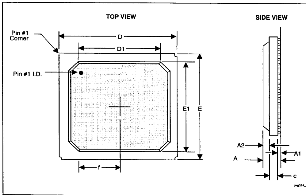
Figure 35. PIIX4 324-Pin Ball Grid Array (BGA)
