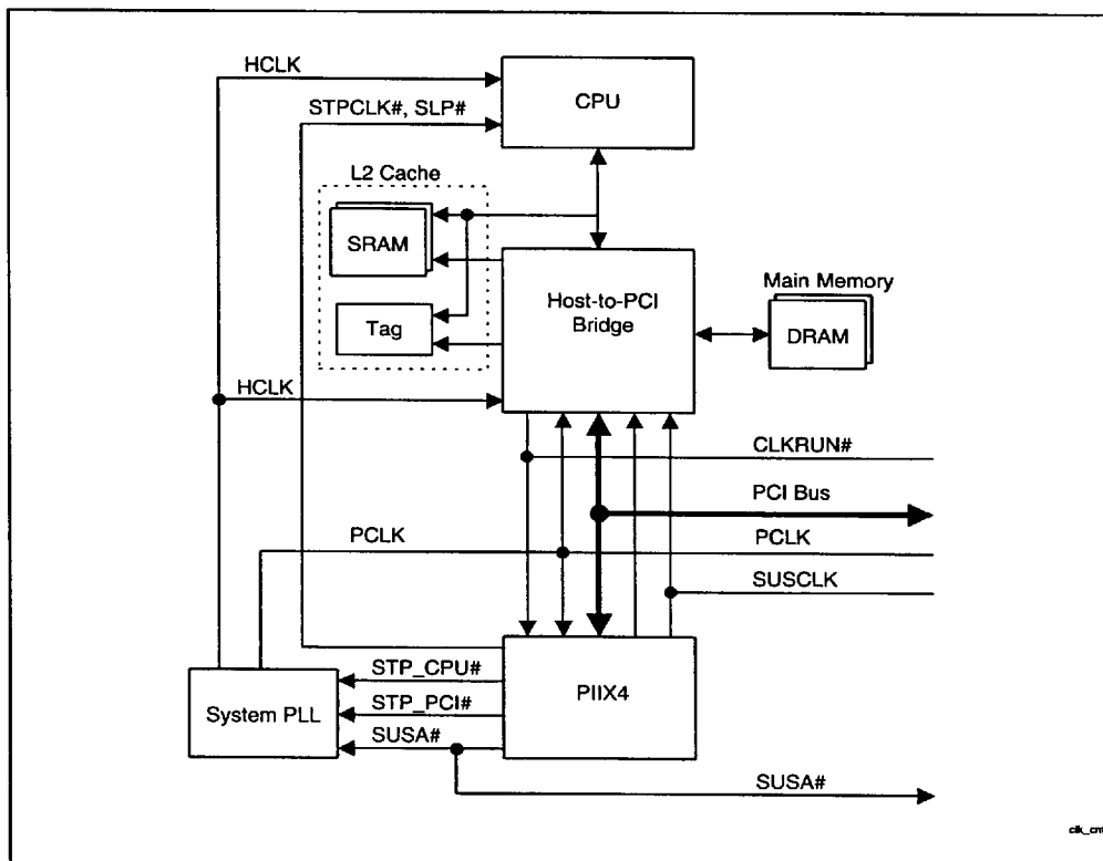
Figure 10. Clock Control
