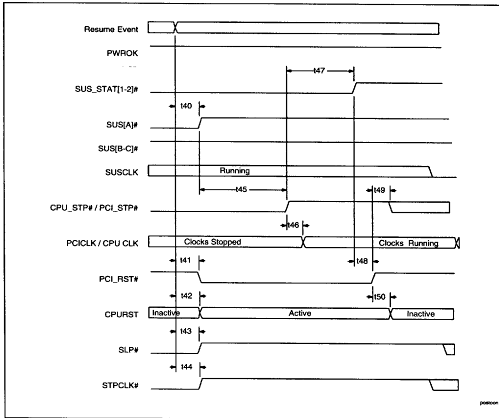
Figure 24. POS to On (w/Processor &amp; PCI Reset)
