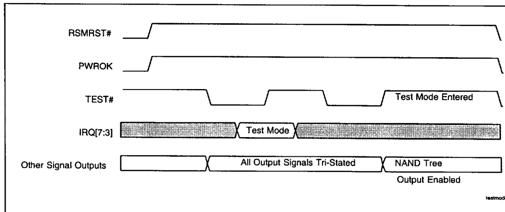
Figure 37. Test Mode Entry (NAND Tree Example)
