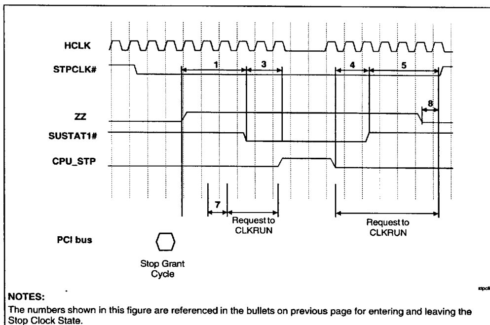
Figure 13. Stop Clock Example
