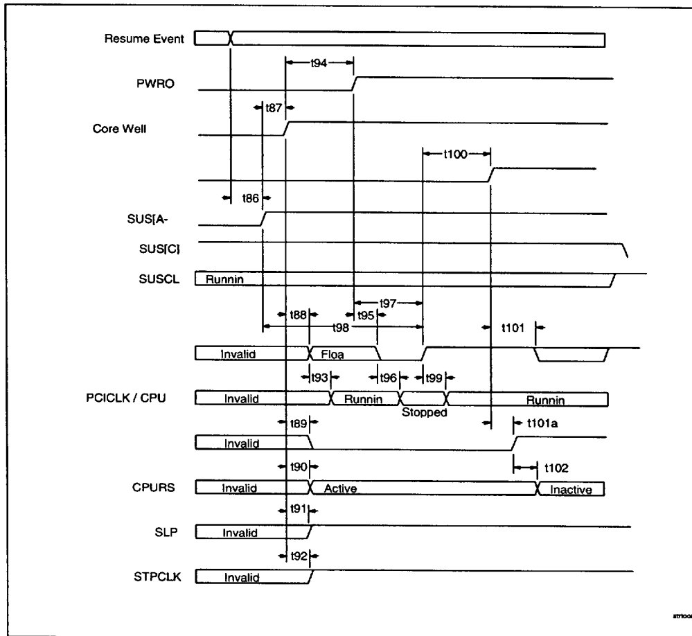
Figure 28. STR to On
