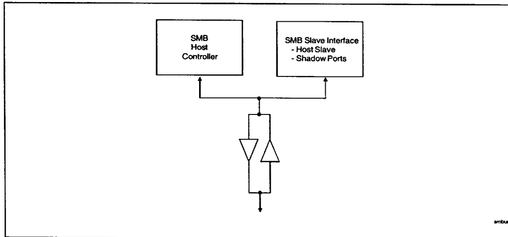
Figure 32. SMBus Interface
