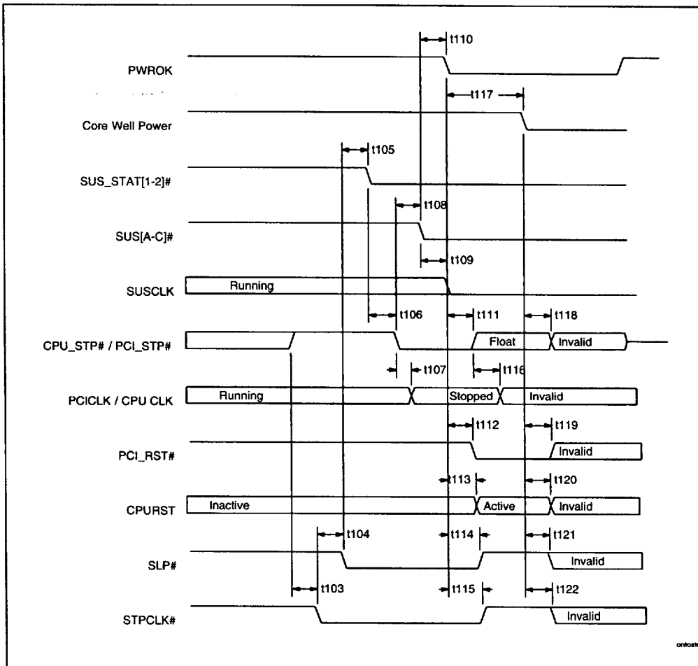
Figure 29. On to STD/SOff
