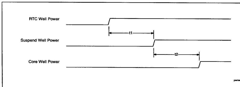
Figure 15. PIIX4 Power Well
