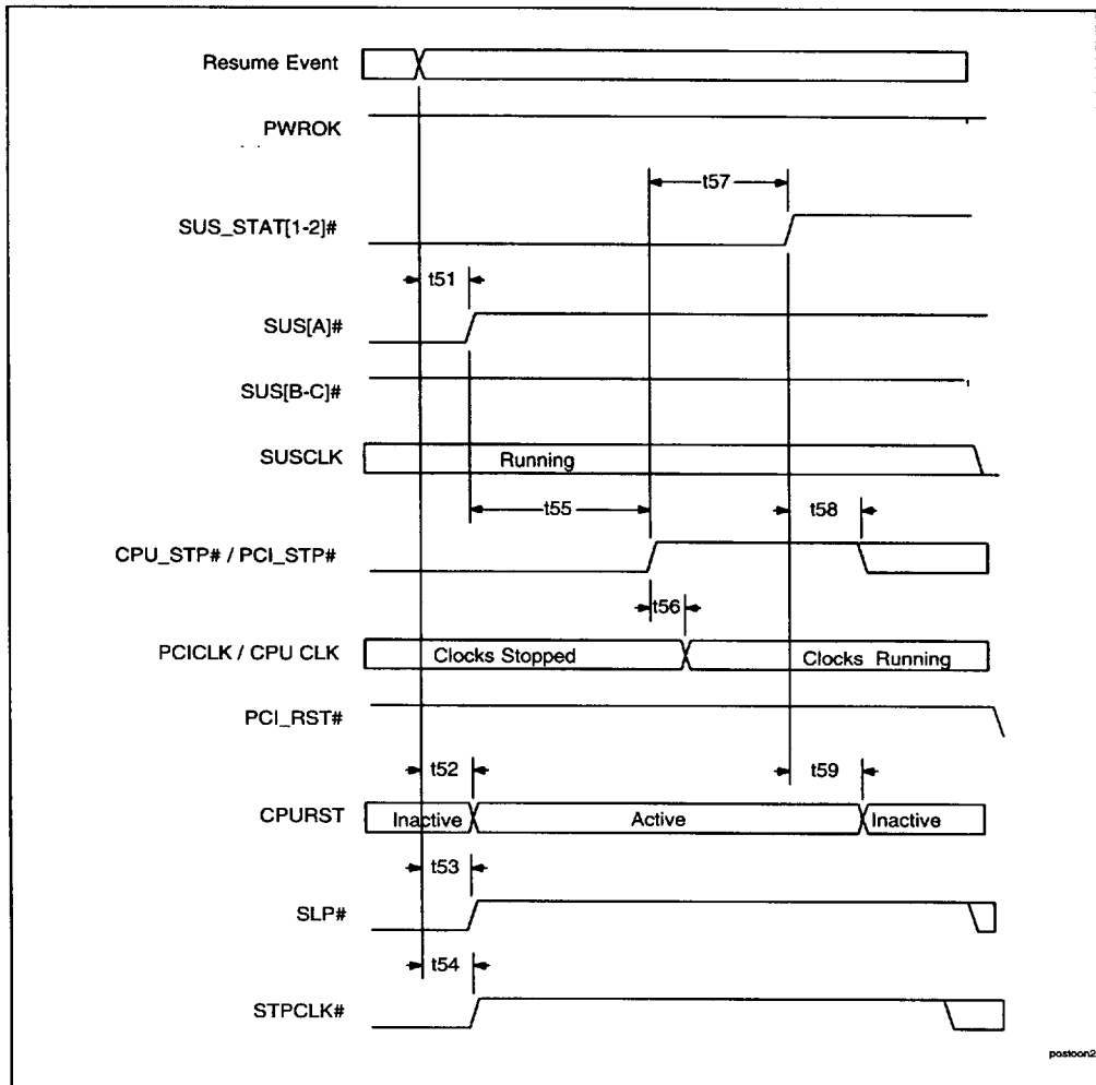
Figure 25. POS to On (w/Processor Reset)
