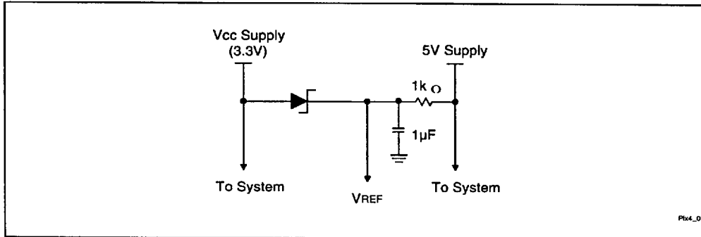
Figure 2. Example Vcc5REF Sequencing Circuit
