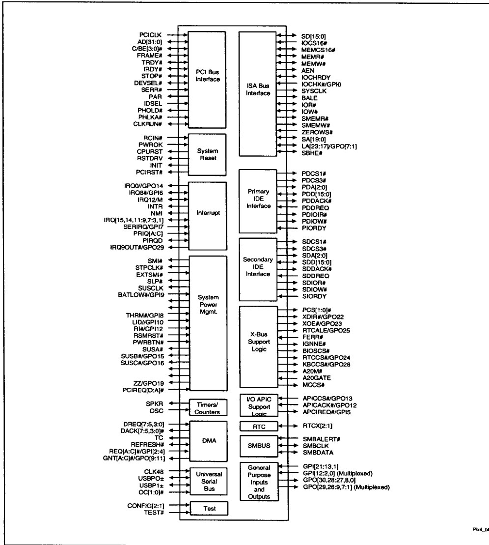
Simplified Block Diagram
