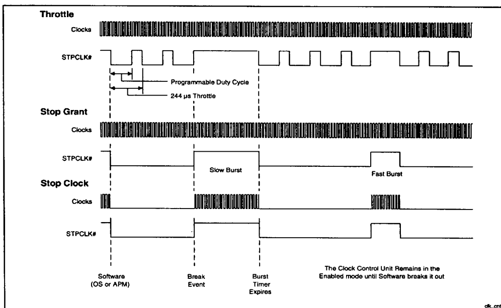
Figure 12. Clock Control Mechanisms (with BURST Enabled)
