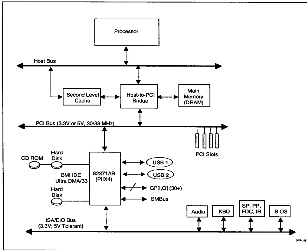
Figure 1. PIIX4 System Block Diagram
