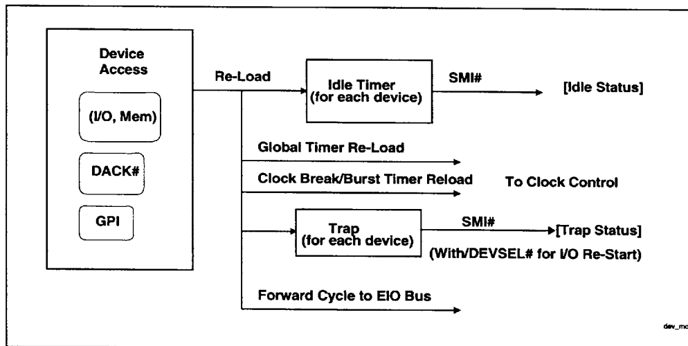
Figure 14. Device Monitoring Logic
