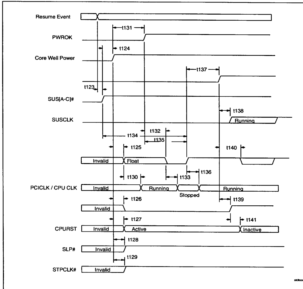
Figure 30. STD/SOff to On
