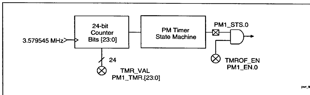
Figure 33. Power Management Timer
