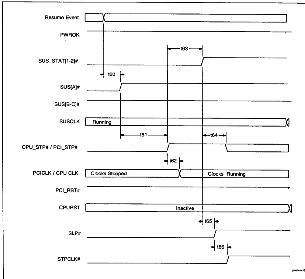
Figure 26. POS to On (No Reset)
