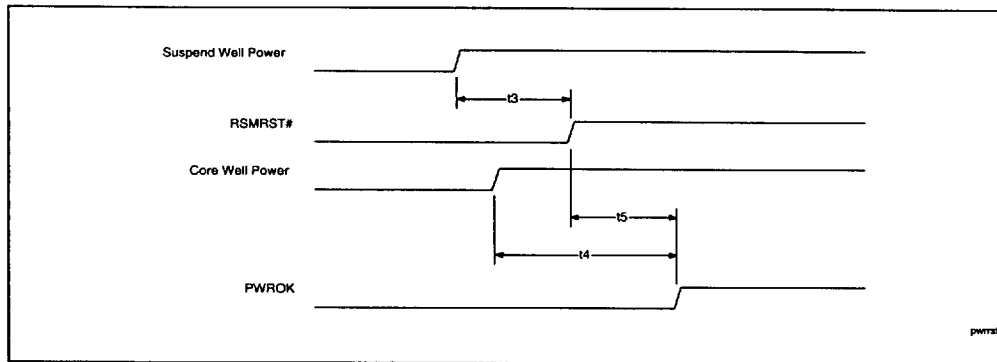
Figure 16. RSMRST# and PWROK Timings
