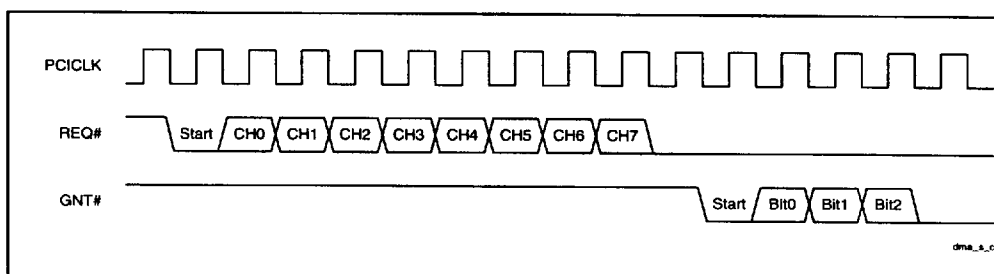
Figure 4. DMA Serial Channel Passing Protocol
