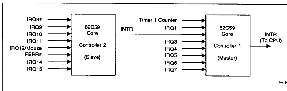
Figure 5. Interrupt Controller Block Diagram
