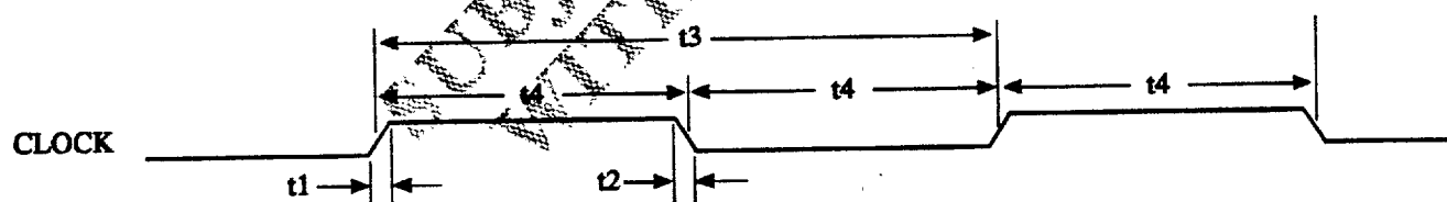
Clock Timing
