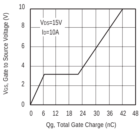
Figure 9. Gate Charge
