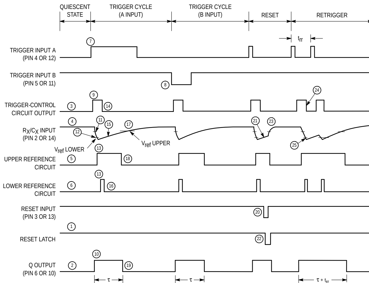
Figure 10. Timing Diagram
