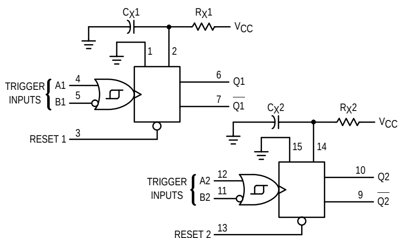
LOGIC DIAGRAM
